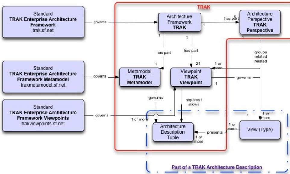
Figure 23 Structure of TRAK - formed from 1 metamodel, 5 architecture perspectives and 21 architecture viewpoints (Wikipedia, 2018)
