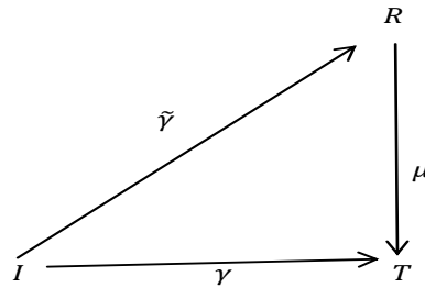
Figure 2.2: The path lifting
