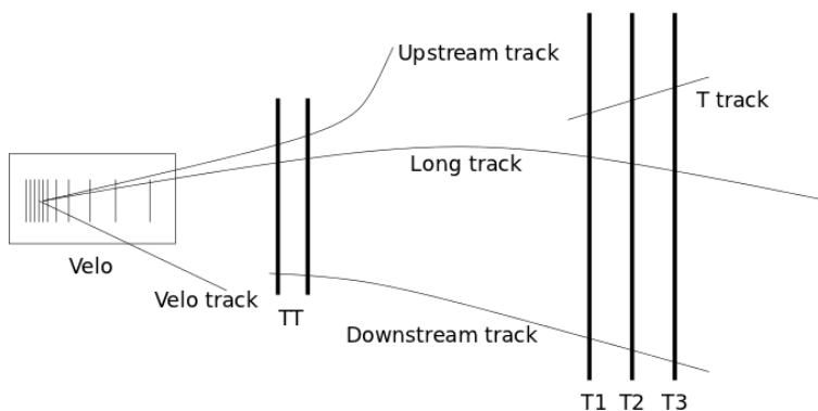
Figure 3.4: Track types in LHCb [10]
