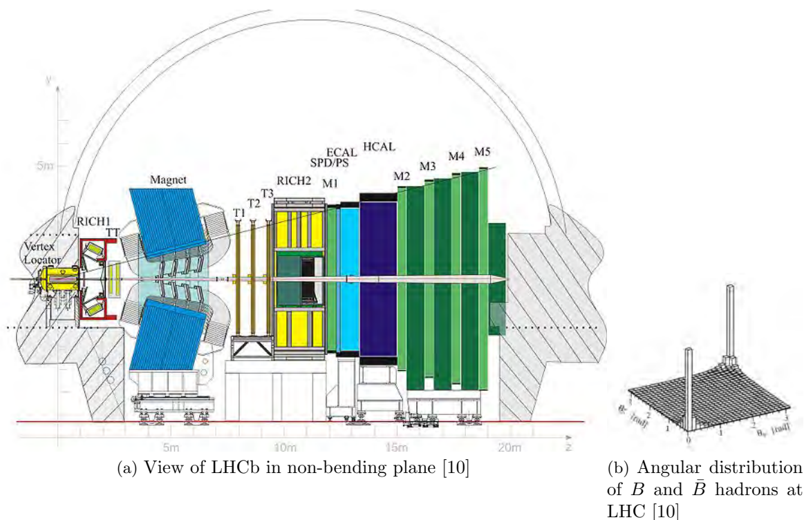
Figure 2.1: Layout of LHCb
