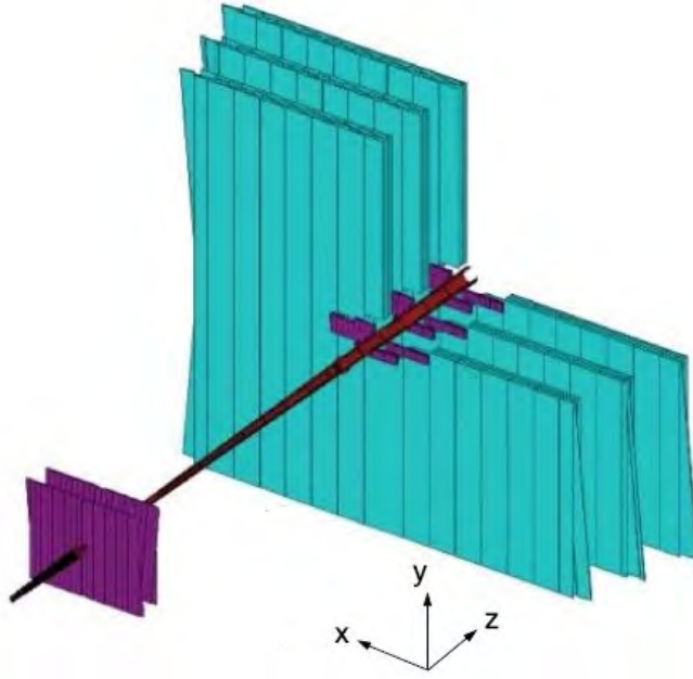
Figure 2.2: TT, IT and OT (blue) [10]
