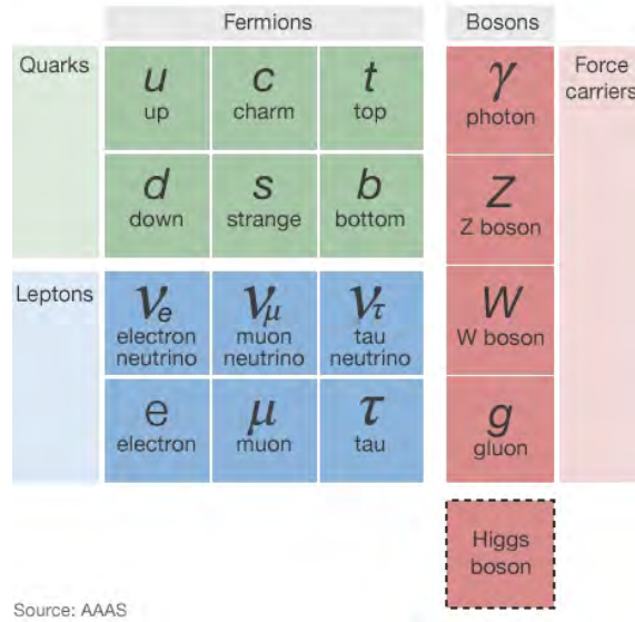
Figure 1.1: The fundamental particles in the SM [1]
