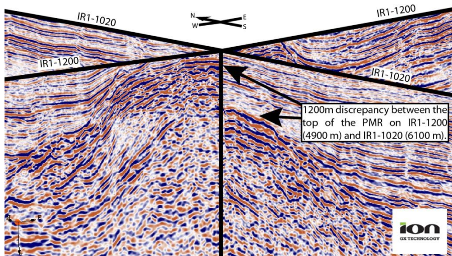
Fig. 2.7: Fence diagram showing the intersection of IR1-1200 and IR1-1020. Note the significant mis-tie between the lines. This is most noticeable for the top PMR reflections. The offset of reflections that should tie is c. 1200m. For this reason IR1-1020 is not used to generate the contours in Fig. 2.10a.
