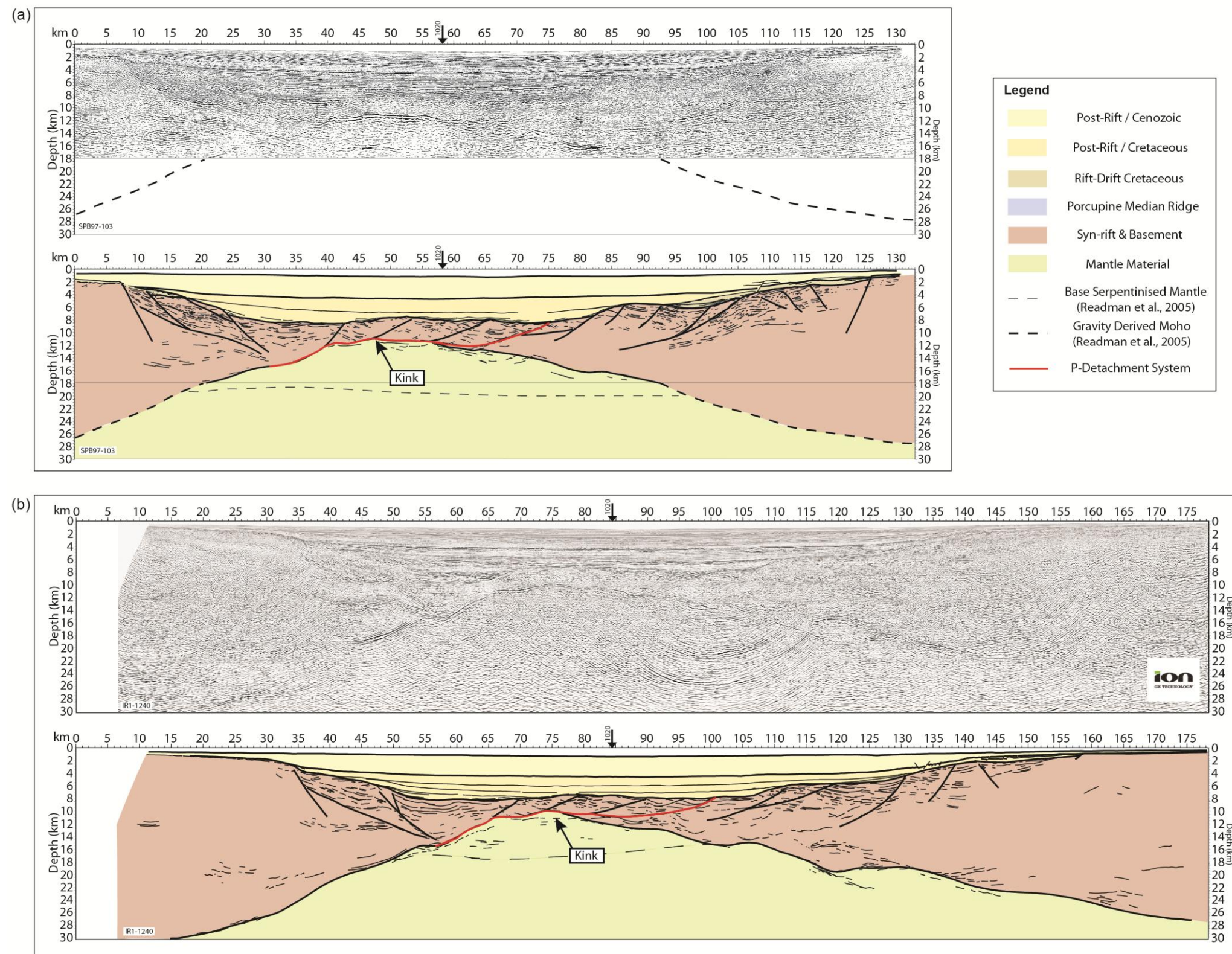
Fig. 2.5: Uninterpreted and interpreted (geoseismic) pre-stack depth migrated (PSDM) seismic profiles. (a) SPB97-103; a composite of reflection seismic data migrated to 18km depth and the gravity model of Readman et al., (2005). Line covers the entire crustal thickness. Faults soling onto the P-detachment are clearly observable. Western Margin is complicated by multiple fault generations. Well imaged fault blocks on the eastern margin. (b) IR1-10240. Migrated to a depth of 30km, images the entire crustal thickness. Western Margin is complicated by multiple fault generations, and faults soling onto the P-detachment can be seen in the central part of the basin. A potential exhumation fault is present at km 75. Well imaged fault blocks on the eastern margin
