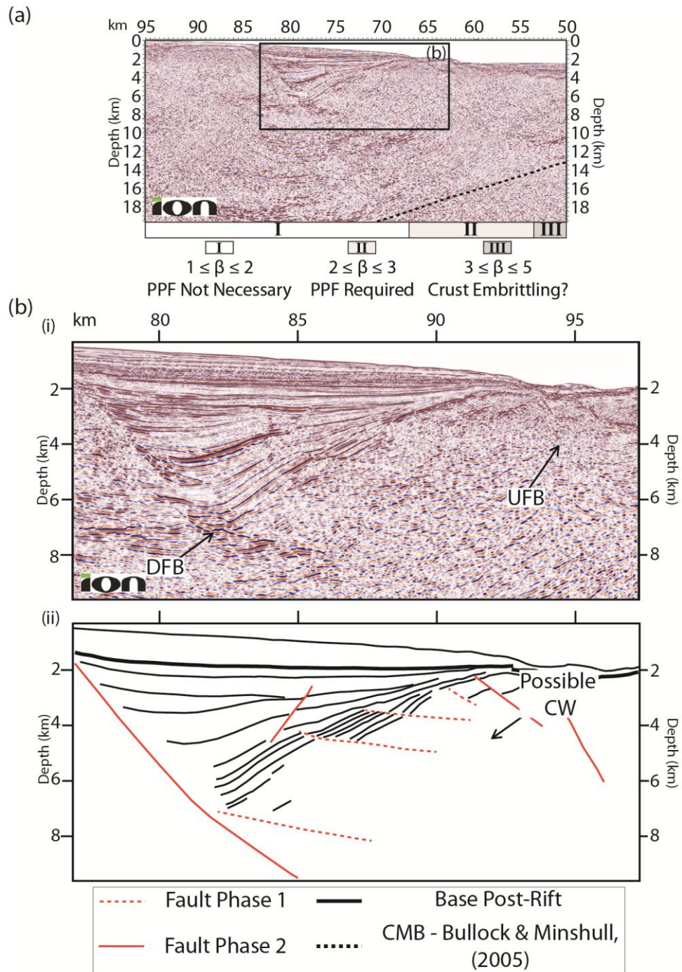
Fig. 5.10: Segment of ION-GXT's IR1-1080 PSDM line from the Goban Spur Margin. (a) Uninterpreted data, with refraction Moho applied. Stretching domains are also assigned. (b) (i) Blow up of half graben structure (Uninterpreted), (ii) Line drawing interpretation of (i) clearly demonstrating two discrete fault generations, forming DFB structures within the half graben. Also note the clearly oversteepened stratigraphy, relative to the latest fault generation.
