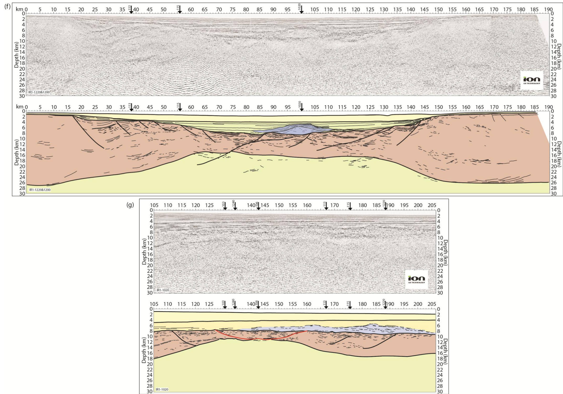
Fig. 2.5 (f): - IR1-1220 & 1200; composite of two dip sections, migrated to a depth of 30 km. Images entire crustal thickness. The PMR appears as a well-developed mounded structure in the centre of the basin. Multiple fault generations are developed on the western margin. The CMB is offset by a possible precursor to the P-detachment system west of the PMR. Fault blocks are not well imaged on the eastern margin. (g) IR1-1020; segment of axial seismic profile, migrated to a depth of 30km. The profile demonstrates thinning of the crust southwards toward the Porcupine Arch, and thickening southwards away from the Porcupine Arch. The PMR appears as a very large elongate mounded structure. The P-detachment appears to be scooped-shaped.
