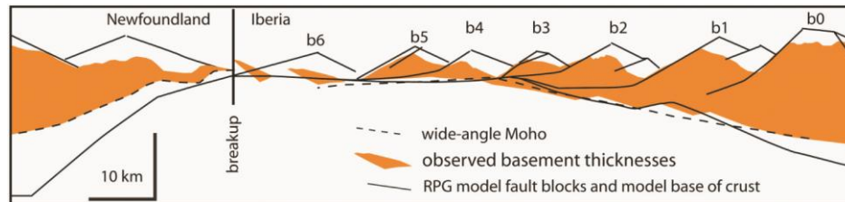
Fig. 5.15: From McDermott & Reston, 2012. Comparison between basement thinning and reduction in fault block size predicted by the sequential faulting mechanism, and that which is observed. Note that the predicted thinning does not match the observed basement thinning at all.
