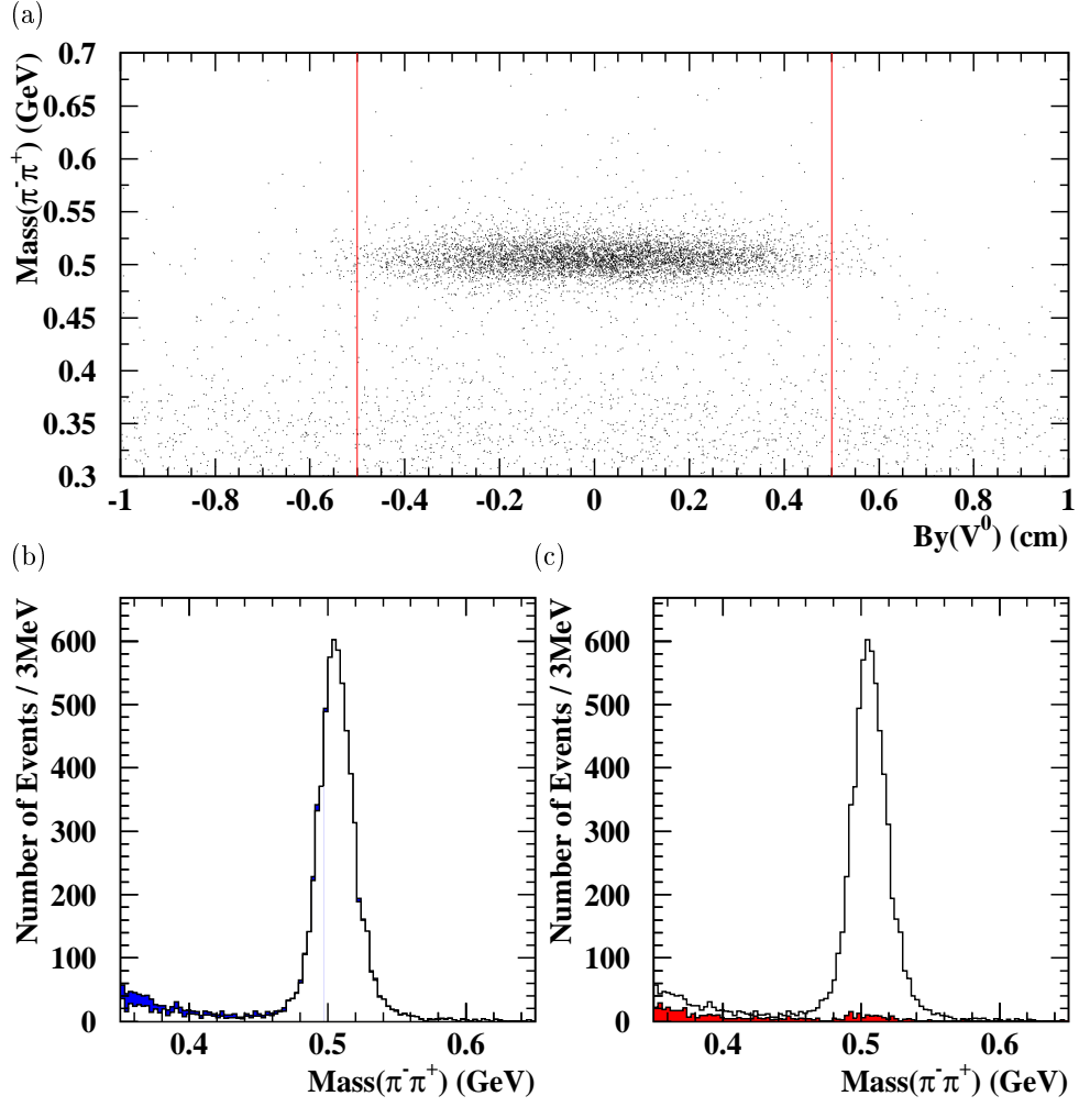
Figure 5.2: (a) \pi^- \pi^+ mass versus the B_y parameter of the V^0 , with all selections except the byv selection, (b) K_S^0 mass with all selections, scaled to, and superimposed on the mass signal without the byv selection, the shaded area is what is removed. (c) What has been removed with the byv selection (shaded) superimposed on the mass signal without the byv selection.
