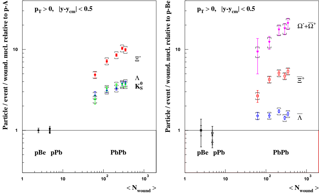
Figure 7.5: Particle yields per wounded nucleon in Pb–Pb, relative to p–Be (p–Pb in the case of K_S^0 ), interactions at 158 A GeV/c as a function of number of wounded nucleons. The vertical lines represents the statistical errors, the \square symbols represents the systematic errors. (NA57 Collaboration).
