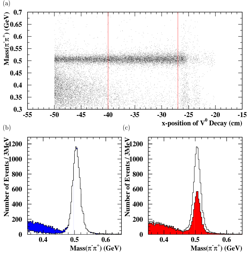
Figure 5.1: (a) \pi^- \pi^+ mass versus x -position of V^0 decay, with all selections except the xvc selection, (b) K_S^0 mass with all selections, scaled to, and superimposed on the mass signal without the xvc selection, the shaded area is what is removed. (c) What has been removed with the xvc selection (shaded) superimposed on the mass signal without the xvc selection.
