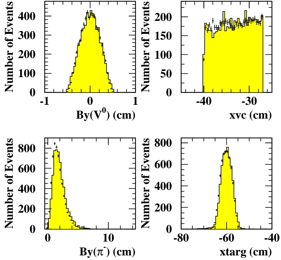
Figure 5.8: The simulated K_S^0 data (crosses) and real data (shaded region) compared, the areas of the simulated data has been scaled to those of the real data.
