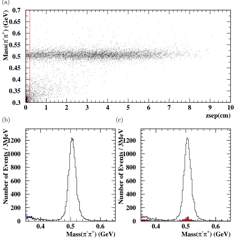
Figure 5.5: (a) \pi^-\pi^+ mass versus the zsep parameter of the V^0 , with all selections except the zsep selection, (b) K_S^0 mass with all selections, scaled to, and superimposed on the mass signal without the zsep selection, the shaded area is what is removed. (c) What has been removed with the zsep selection (shaded) superimposed on the mass signal without the zsep selection.
