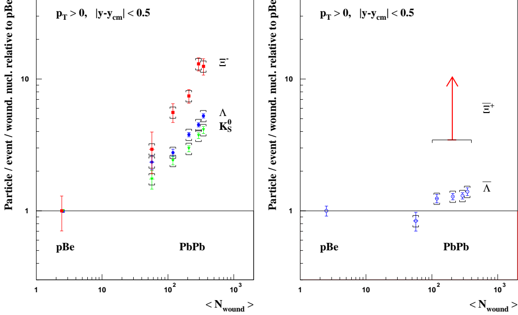
Figure 7.2: Particle yields per wounded nucleon in Pb–Pb, relative to p–Be, interactions at 40 A GeV/c as a function of the number of wounded nucleons using the results in this thesis. The vertical lines represents the statistical errors, the \square symbols represents the systematic errors.
