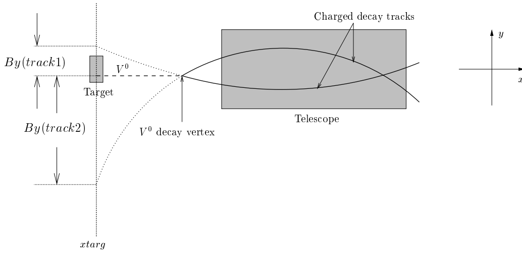
Figure 3.13: The definition of the B_y parameters of the charged tracks: the distance in y in a vertical ( y-z ) plane, with x value fixed to x_{targ} , between the nominal centre of the beam profile, y_0 , and the intersection of the plane with the curvature of flight of each of the charged tracks.
