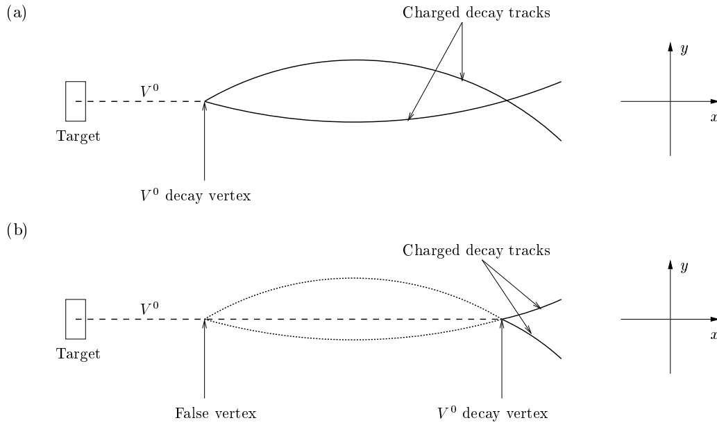
Figure 3.1: A neutral particle, known as a V^0 , decays into two oppositely charged tracks in either (a) a cowboy topology or (b) a sailor topology. NA57 favours the cowboy topology.
