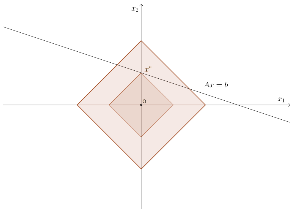
Figure 1.1: Geometry of \ell_1 -minimization in two dimensions. x^* is the sparsest solution of Ax = b with the least \ell_1 -norm.
