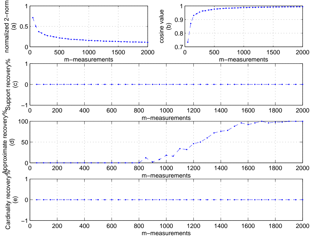
Figure 5.4: Performance of 1-bit basis pursuit with Gaussian matrices and varied measurements at the fixed sparsity level k = 5 . (a) Normalized \ell_2 -norm residual \left\| \frac{x^*}{\|x^*\|_2} - \frac{x}{\|x\|_2} \right\|_2 , (b) Cosine value of the angle between x^* and x , (c) Success rate of support recovery at each measurements level, (d) Success rate of approximate sparse recovery at each measurements level, and (e) Success rate of finding a sparsest solution to the linear system (5.1.1) at each measurements level.
