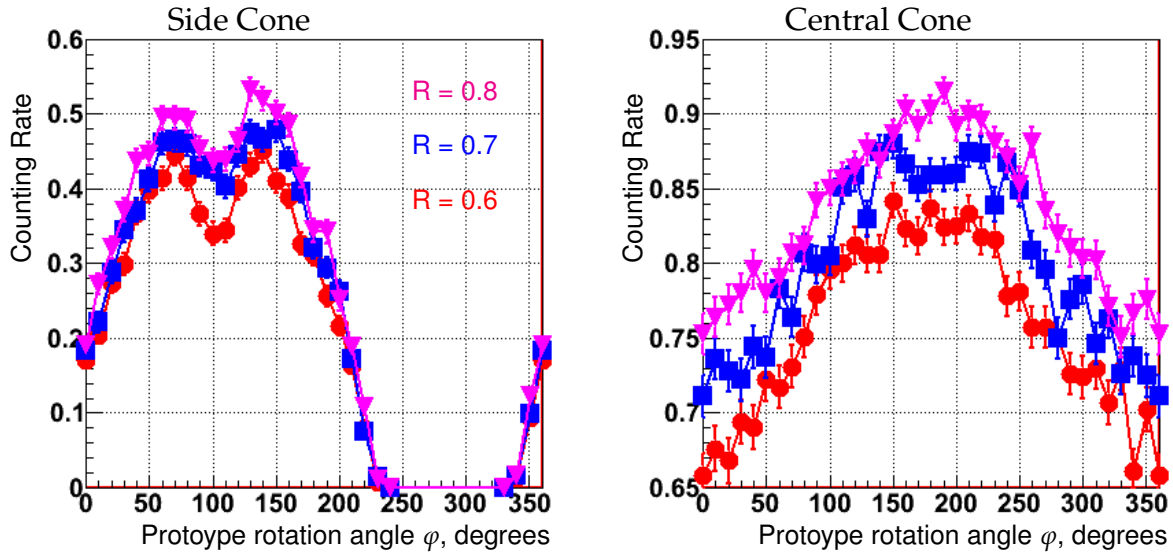
Figure 6.14: MC predictions for counting rates per beam pion, as a function of prototype rotation angle \varphi for different reflectivities ( R ) of the aluminium cones.
