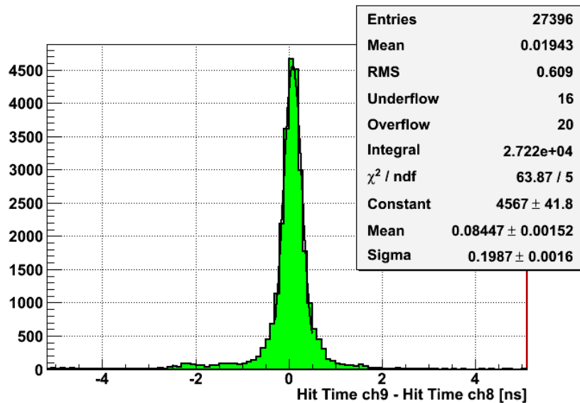
Figure 6.21: Time difference of new PMTs in channels 8 and 9 with the rad-hard front-end option. Solid line is the Gaussian fit of the central part of the distribution.
