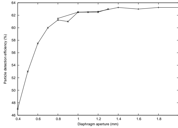
Figure 6.5: Detection efficiency as a function of the diaphragm aperture at fixed gas pressure on the pion peak
