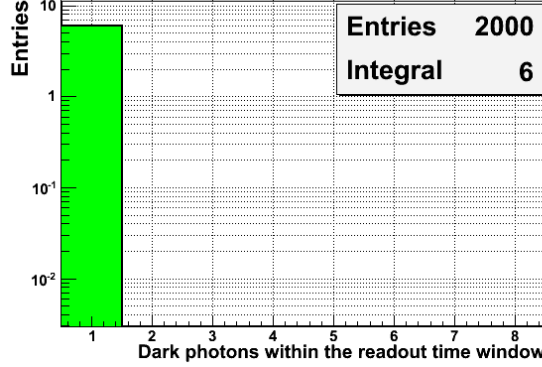
Figure 5.24: Dark photon events within readout time windows.
