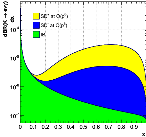
Figure 1.5: Spectra of differential branching ratio of K_{e2\gamma}^+ as functions of x for SD ( \chi PT \mathcal{O}(p^6) ) and IB terms (logarithmic scale). The contributions from \text{INT}^\pm are not plotted as they are vanishingly small ( 10^{-5} < \text{BR}_{\text{INT}^\pm} / \text{BR}_{\text{SD}^\pm} < 10^{-2} ).
