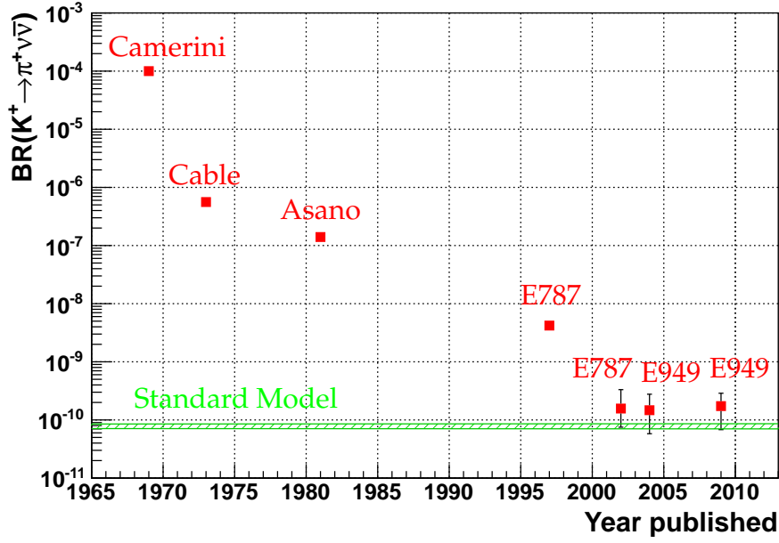
Figure 1.12: Summary of the \text{BR}(K^+ \rightarrow \pi^+ \nu \bar{\nu}) experimental status over the years.
