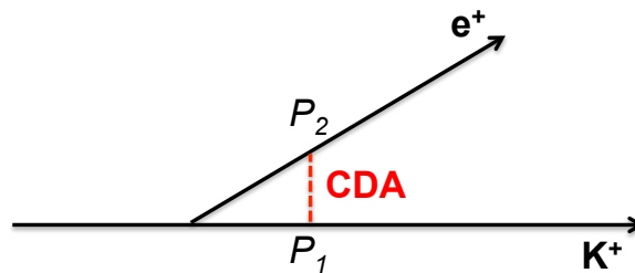
Figure 3.1: Schematic of the Closest Distance of Approach (CDA) between the kaon and the positron trajectories.
