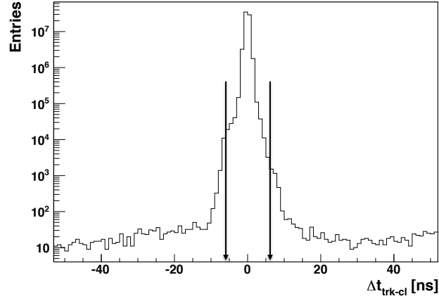
Figure 3.6: Data distribution of the time difference between the positron track and the photon cluster at LKr ( \Delta t_{trk-cl} ). The arrows represent the cut applied in the event selection.
