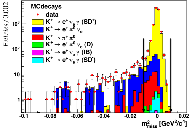
Figure 3.35: Reconstructed m_{miss}^2 distributions of K_{e2\gamma}^+ ( SD^2 ) candidates compared with the sum of normalised estimated signal and background components (logarithmic scale). The arrows define the signal region chosen for the analysis. The deficit of reconstructed MC events in the region below 0.01 \text{ GeV}^2/c^4 is mostly outside the signal region and due to resolution effects dominated by non-Gaussian tails. Such effects are being investigated.
