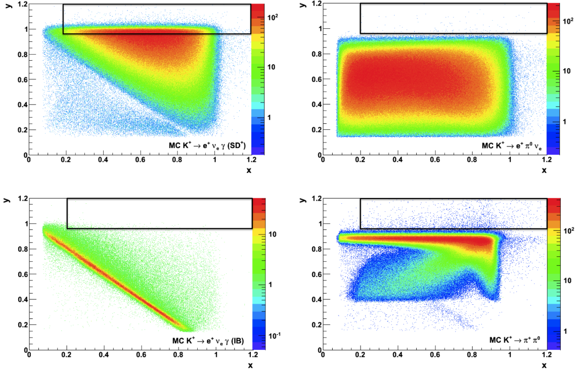
Figure 3.9: Distribution of reconstructed x and y kinematic variables for the signal K_{e2\gamma}^+(\text{SD}^+) (top-left) and background K^+ \rightarrow \pi^0 e^+ \nu_e (top-right), K_{e2\gamma}^+(\text{IB}) (bottom-left) and K^+ \rightarrow \pi^+ \pi^0 (bottom-right) MC events (logarithmic colour scale). The overlay regions define the analysis kinematic region.
