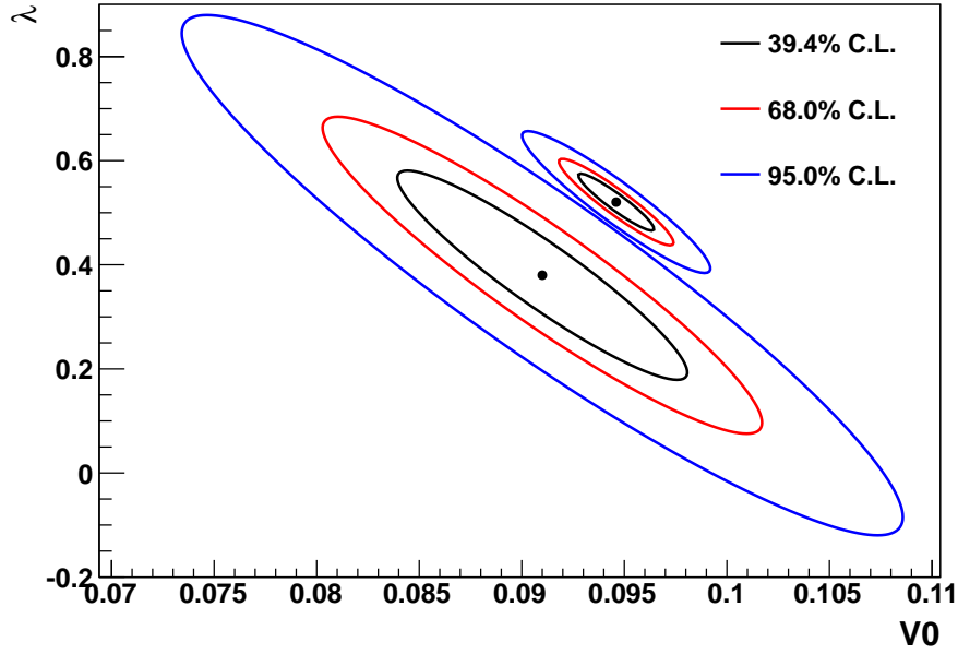
Figure 3.42: Comparison between NA62 and KLOE K_{e2\gamma}^+ ( SD^+ ) form factor measurements. Confidence interval ellipses in the (V_0, \lambda) plane at 1\sigma , 2\sigma , 3\sigma (2D case).
