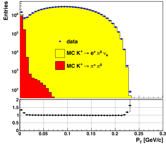
Figure 3.17: Reconstructed transverse momentum, P_T , distributions of K^+ \rightarrow \pi^0 e^+ \nu_e candidates compared with the sum of normalised estimated signal and background components (logarithmic scale). Data/MC ratio shows a disagreement for P_T < 0.01 \text{ GeV}/c , which might be due to a non perfect rejection of the K^+ \rightarrow \pi^+ \pi^0 decay peaking in this P_T region.
