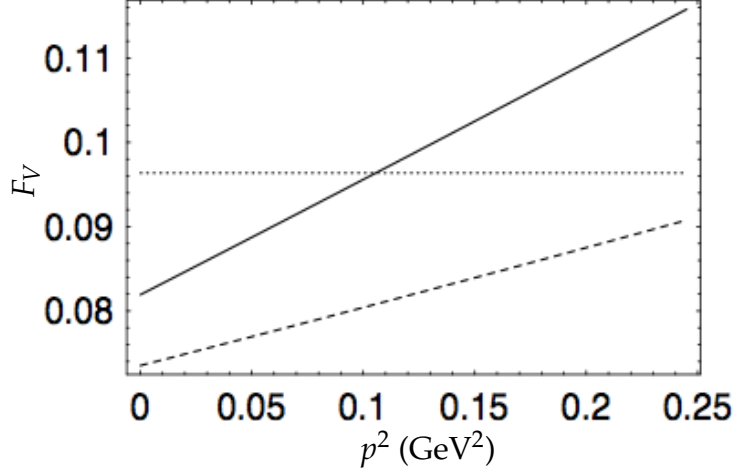
Figure 1.4: The form factor F_V as a function of the momentum transfer p^2 for K_{e2\gamma}^+ . Dotted, solid and dashed lines are the \chi PT predictions at \mathcal{O}(p^4) , \mathcal{O}(p^6) in the VMD model and \mathcal{O}(p^6) in the CQM model, respectively [13].
