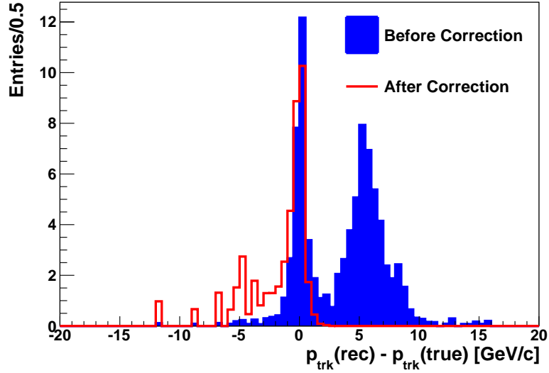
Figure 3.29: \Delta p = p_{\text{trk}}(\text{rec}) - p_{\text{trk}}(\text{true}) distributions for K_{2\pi} MC events passing the signal event selection (without E_{\text{LKr}}/p_{\text{trk}} cut) before (blue) and after (red) the correction for the dependence of P(\pi \rightarrow e) on \Delta p . The effect of the correction is visible as the peak at 5 GeV/c disappeared due to the anti-correlation between E_{\text{LKr}}/p_{\text{trk}} and \Delta p .
