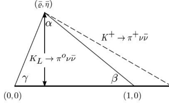
Figure 1.10: Unitarity triangle corresponding to the condition 1.38. The K^+ \rightarrow \pi^+ \nu \bar{\nu} decay rate defines the dashed side and the displacement of the right down vertex is due to the charm-quark contribution; the K_L \rightarrow \pi^0 \nu \bar{\nu} decay rate gives the \eta parameter, namely the triangle height.
