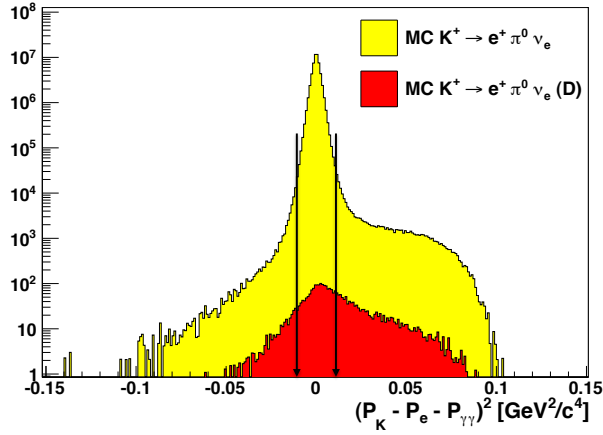
Figure 3.13: m_{miss}^2 = (P_K - P_e - P_{\gamma\gamma})^2 distributions for MC (signal, yellow) K^+ \rightarrow \pi^0 e^+ \nu_e ( \pi^0 \rightarrow \gamma\gamma ) and (background, red) K^+ \rightarrow \pi^0 e^+ \nu_e ( \pi^0 \rightarrow e^+ e^- \gamma ) Dalitz events. The difference in the spectra suggests a narrow cut at m_{miss}^2 < 0.01 GeV 2 / c^4 in order to reduce this background contamination.
