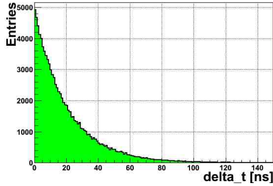
Figure 5.15: Kaon arrival time distribution.
