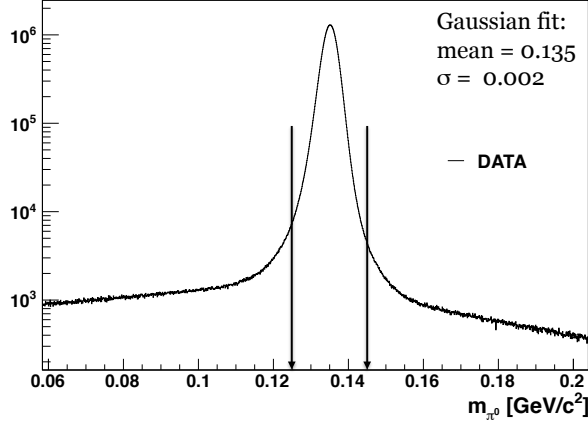
Figure 3.11: \gamma\gamma mass distribution for data (logarithmic scale) passing the K^+ \rightarrow \pi^0 e^+ \nu_e event selection cuts described up to this point.
