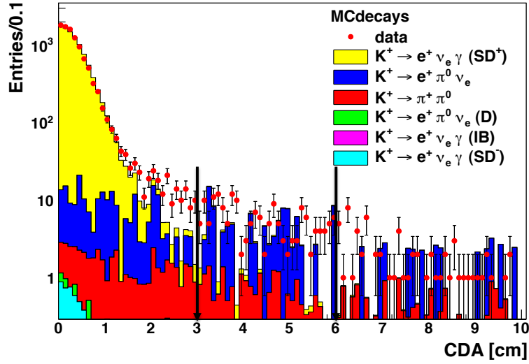
Figure 3.34: Reconstructed CDA distributions of K_{e2\gamma}^+ ( SD^2 ) candidates compared with the sum of normalised estimated signal and background components (logarithmic scale). The deficit of reconstructed MC events in the region above 2 cm is due to resolution effects dominated by non-Gaussian tails. Detailed studies of such effects are on still going. The arrows represent the side-band chosen for the study of the background from non-Gaussian tails of MCS.
