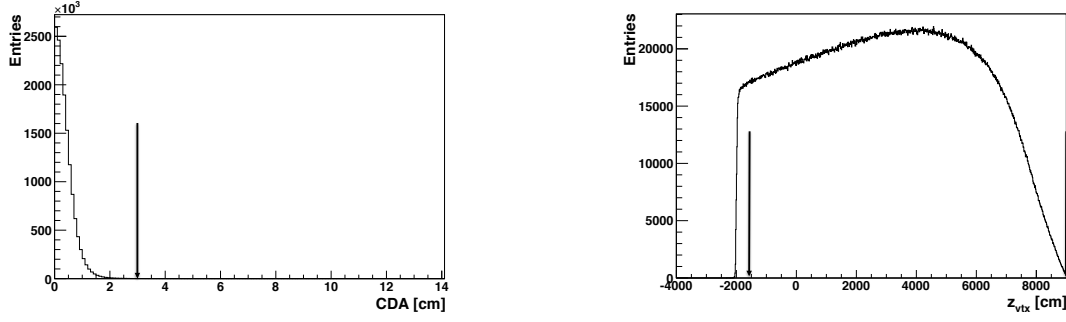
Figure 3.2: (Left) Closest Distance Approach (CDA) parameter for MC K_{e2\gamma}^+ ( SD^+ ) events. (Right) Longitudinal decay vertex ( z_{vtx} ) for MC K_{e2\gamma}^+ ( SD^+ ) events; the arrows represent the cuts applied in the event selection. z_{vtx} = -18 m corresponds to the position of the final collimator on the beam line.
