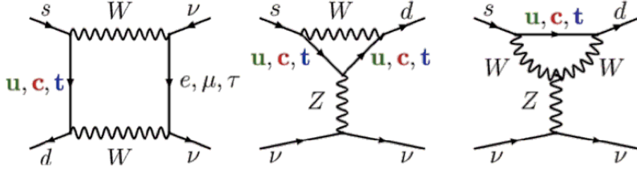
Figure 1.9: One-loop diagrams contributing to the s \rightarrow d\nu\bar{\nu} process. From left: a W -box diagram and two Z -penguin diagrams.
