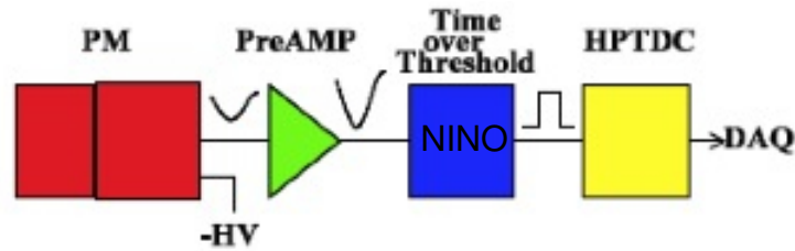
Figure 6.6: CEDAR new front-end and readout system designed for NA62.
