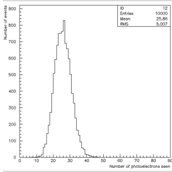
Figure 5.12: Number of photo-electrons seen per kaon event: plot taken from a Monte-carlo simulation on the existing CEDAR [93].
