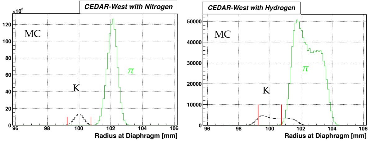
Figure 5.3: Cherenkov photon ring radius at the diaphragm plane expected for kaons (black) and pions (green). Left: CEDAR operating with N_2 gas at an absolute pressure of 1.7 bar. Right: CEDAR operating with H_2 gas at an absolute pressure of 3.3 bar. The standard annular aperture ( w_D = 1.5 mm) is represented by red lines.
