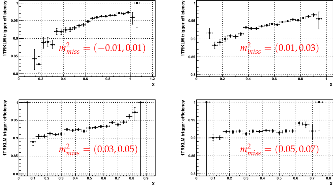
Figure 3.32: 1TRKLM trigger efficiency versus x for events passing the K_{e2\gamma}^+ ( SD^+ ) event selection without kinematic cuts; the plots correspond to 4 control regions of the m_{miss}^2 variable. The top-left panel corresponds to the signal region.
