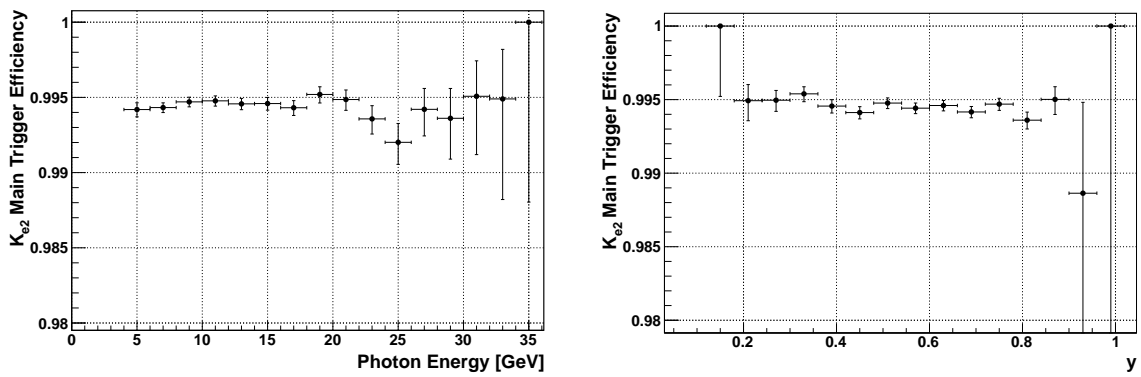
Figure 3.23: The total “ K_{e2} main trigger” efficiency vs the photon energy in the lab frame (left) and the y variable in the kaon rest frame (right) for K_{e3} events.
