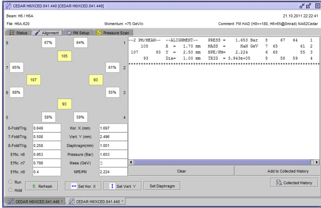
Figure 6.2: Standard “CEDAR” software interface screenshot: (left-up side) counting rates for eight standard PMTs written on white boxes which are displaced in circle; counting rates for four grouped PMTs written on yellow boxes arranged on an inner circle; (left-down side) indicators for 6-, 7- and 8-fold coincidence rates; X-Y positions of the nose, diaphragm width, gas pressure; controls for the CEDAR alignment. In the right side of the screenshot a typical printout of the alignment procedure is showed; the CEDAR was set on the pion pressure and the counting rates ((55 ÷ 68)%) reflect the pion fraction in the beam.
