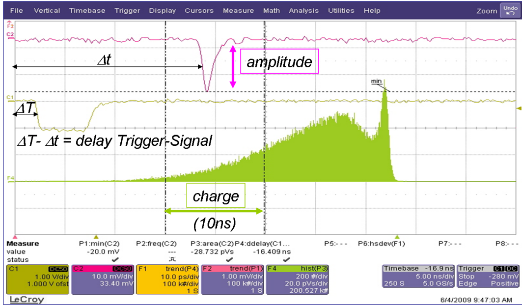
Figure 5.9: Digital sampling oscilloscope snapshot (time scale 5\text{ns}/\text{div} ): PMT anode signal (top waveform, voltage scale 10\text{mV}/\text{div} ), laser signal (central waveform, voltage scale 1\text{V}/\text{div} ), anode charge spectrum (bottom distribution) and fixed time window for charge integration ( 10\text{ns} ).
