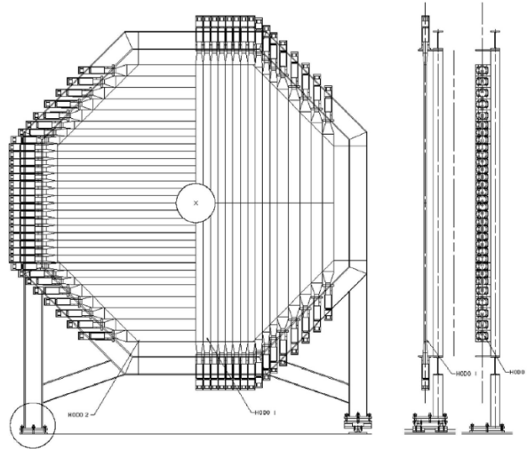
Figure 2.5: Schematic layout of the HOD detector.
