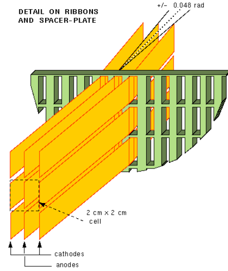
Figure 2.6: LKr calorimeter: (left) half structure while under construction; (right) details of the cell structure.
