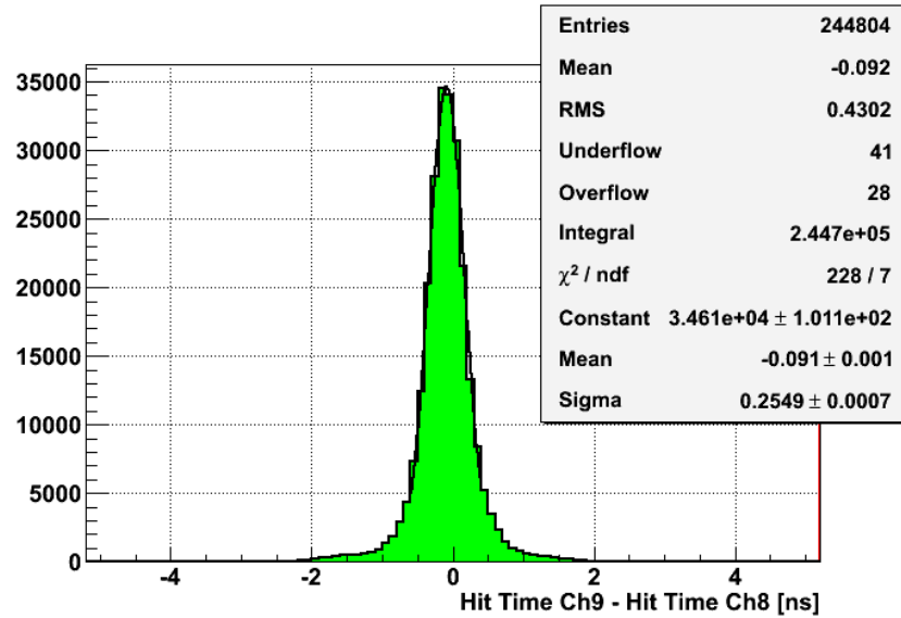
Figure 6.19: Time difference of new PMTs in channels 8 and 9. Solid line corresponds to a gaussian fit of the core of the distribution.
