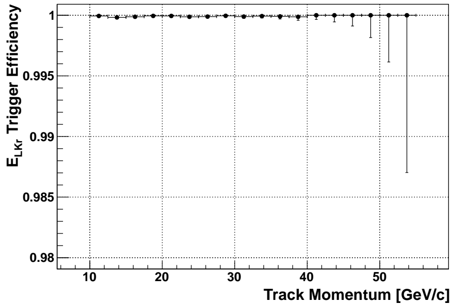
Figure 3.20: The E_{LKr}(10 \text{ GeV}) trigger efficiency as a function of the track momentum measured using K_{e3} events.
