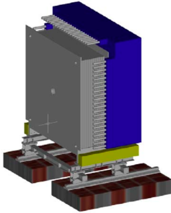
Figure 4.10: Schematic view of MUV1 (grey) and MUV2 (blue). The beam is coming from the left.
