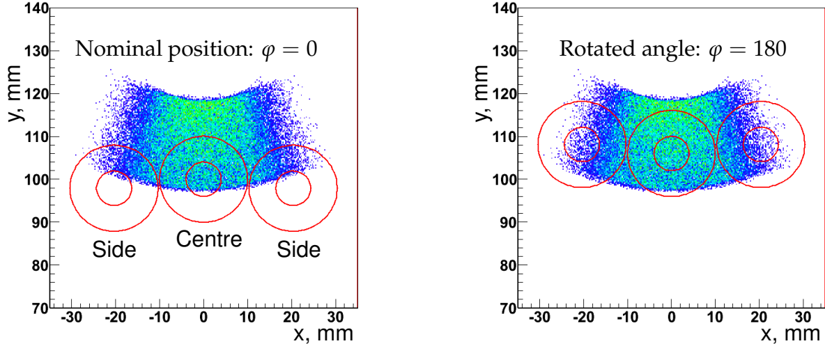
Figure 6.11: NA62-MC simulation of the Cherenkov light at the new-PMT plane (with extension tube in place) overlaid with the PMT assembly in its nominal position (left) and rotated by 180 degree (right). The y-axis in the plots points radially but the actual prototype was rotated by 22.5^\circ with respect to the plot. The centre of rotation of the prototype was at x = 0, y = 103 mm.
