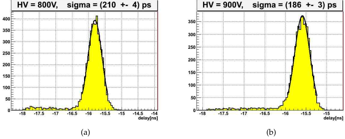
Figure 5.11: PMT response time distributions with a 20% light attenuation optical filter at V_{HV} values: 800 V, 900 V.
