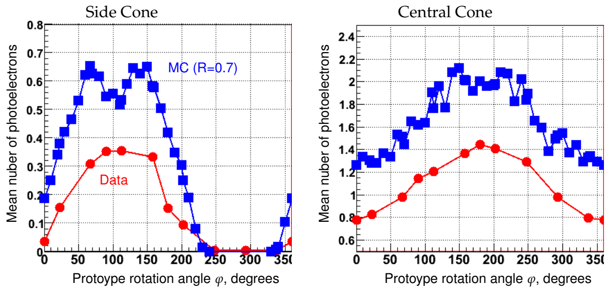
Figure 6.16: Data and MC comparison for mean numbers of photoelectrons per beam pion (assuming cone reflectivity of 0.7).
