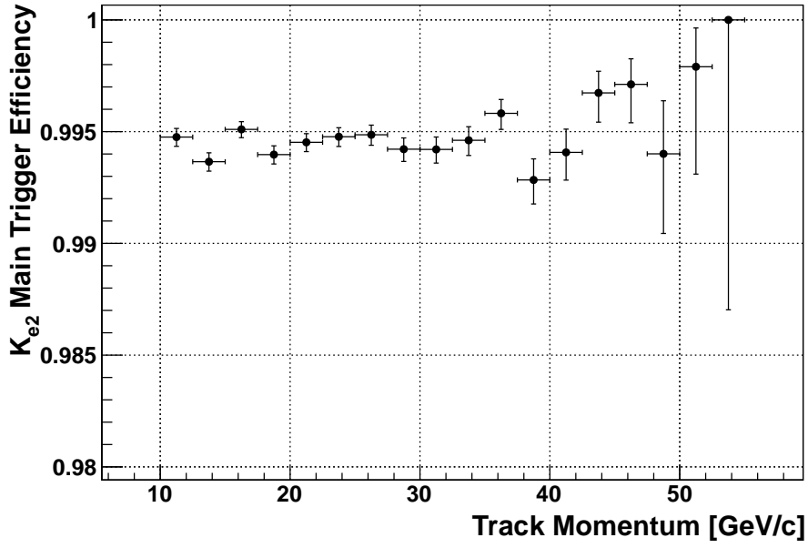
Figure 3.22: The total “ K_{e2} main trigger” efficiency as a function of the track momentum measured using K_{e3} events.
