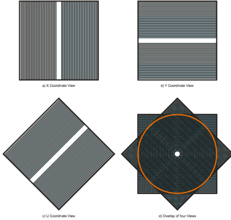
Figure 4.7: Straw chamber four “Views” assembly: a) the x “view” with straws vertically oriented; b) the y “view” with horizontal straws; c) the u “view” with straws rotated by 45 degrees with respect to the straws in the y “view” (the v “view” is rotated by 90 degrees with respect to the u “view”); d) One straw chamber assembly made of the four “Views”; each chamber has an active area of 2.1 m diameter. The central hole allows the beam passage.
