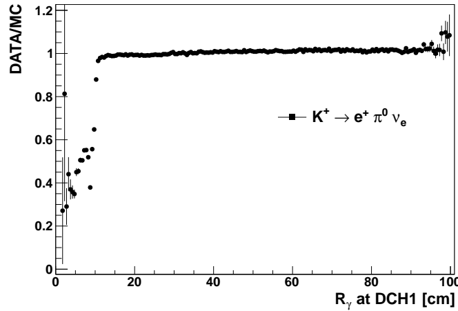
Figure 3.7: Photon radius at the DCH1: data-MC ratio for fully reconstructed K^+ \rightarrow \pi^0 e^+ \nu_e events. The discrepancy for values below 12 cm is compatible with photon interactions in the DCH1 flange, which are not adequately simulated.
