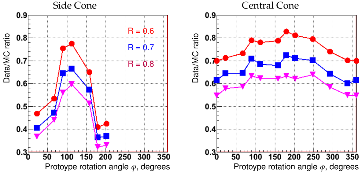
Figure 6.17: Data/MC ratios for mean numbers of photoelectrons per beam pion, as a function of prototype rotation angle \varphi for different reflectivities ( R ) of the aluminium cones.
