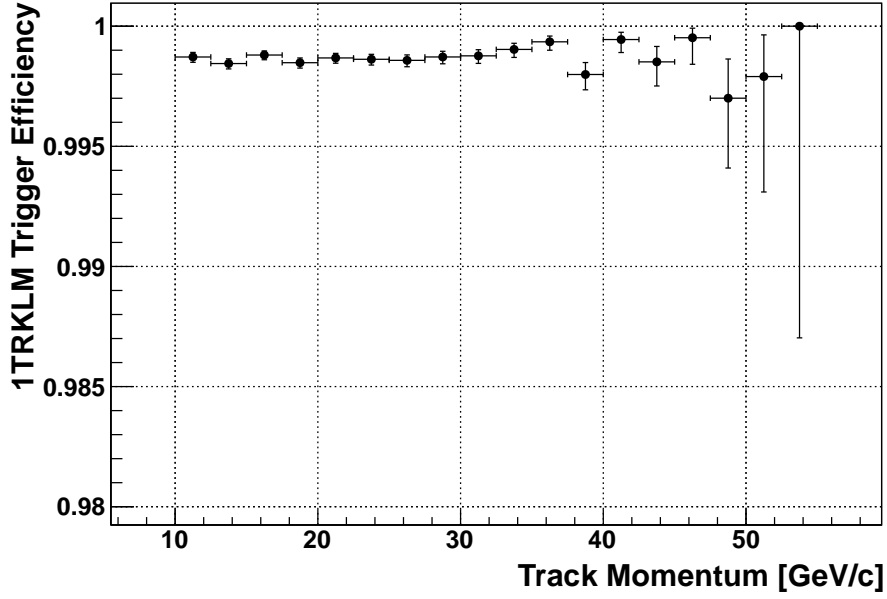
Figure 3.21: The 1TRKLM trigger efficiency as a function of the track momentum measured using K_{e3} events.
