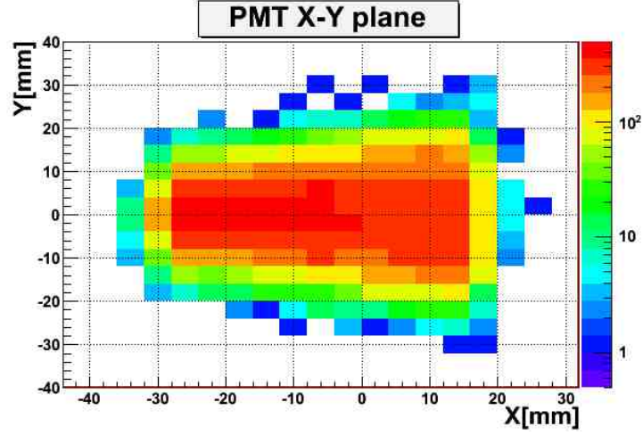
Figure 5.14: One-Spot light distribution on the X-Y photodetector (PMT) plane.
