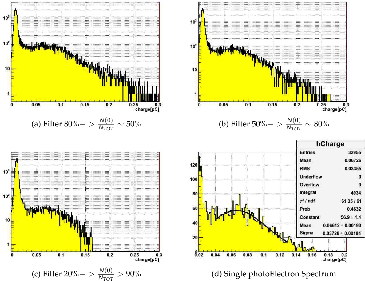
Figure 5.10: PMT anode charge spectra measured at a gain of 10^6 ( V_{HV} = 900 V) for different values of the light attenuation.
