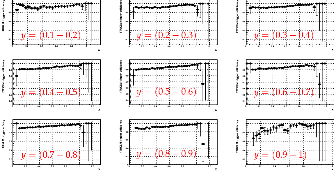
Figure 3.31: 1TRKLM trigger efficiency versus x for events passing the K_{e2\gamma}^+ (SD + ) event selection without kinematic cuts; the plots correspond to 9 regions of y defined as (y_i, y_i + 0.1) with y_i = 0.1, 0.2, \dots, 0.9 .
