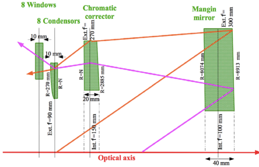
Figure 5.2: Schematic layout of the optical elements inside the CEDAR vessel and a sketch of the light path.
