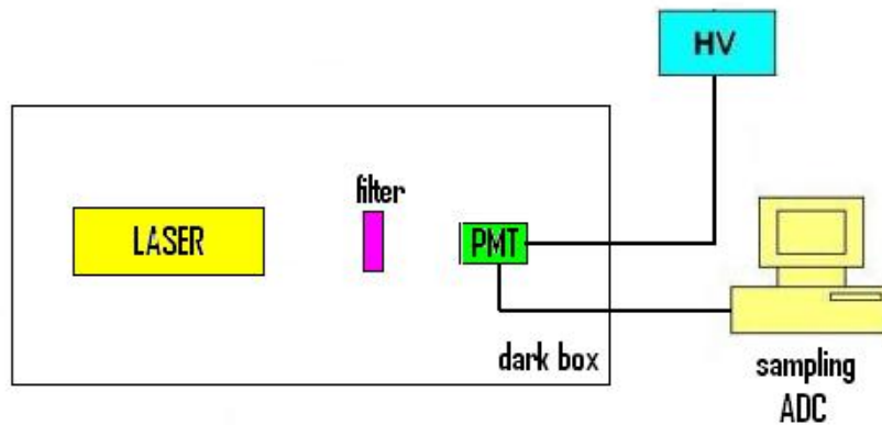
Figure 5.7: Experimental setup at CERN.
