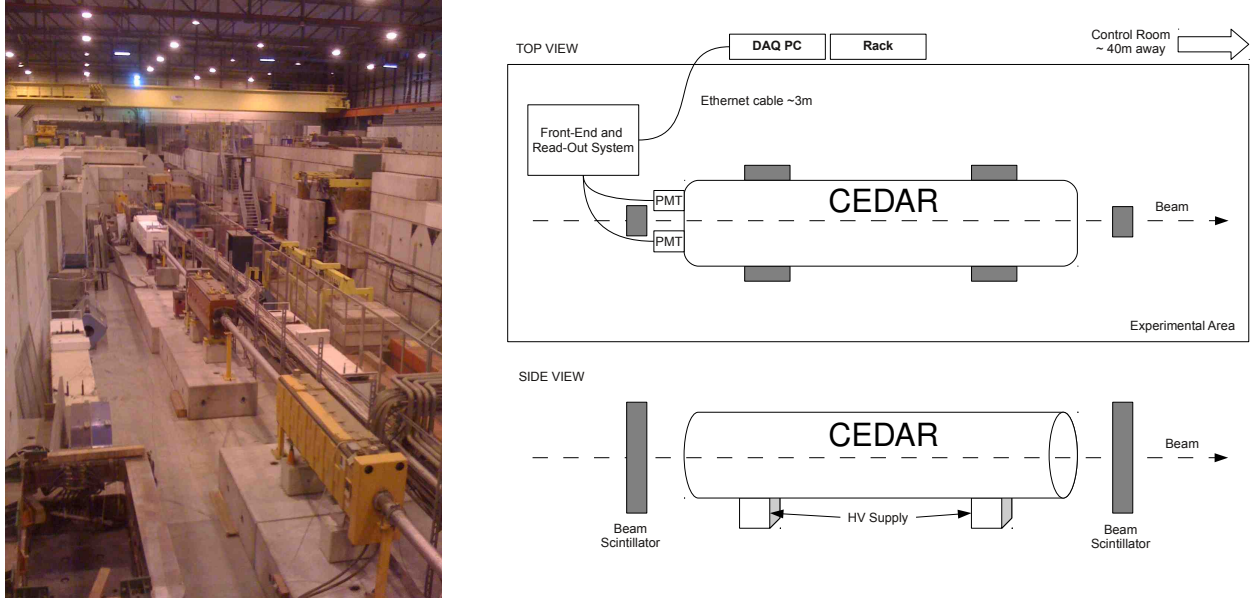
Figure 6.1: Left: CEDAR counter (white rectangular box) positioned on the H6 beam line. Right: schematic layout used for the CEDAR test beam (top view, side view, not to scale).
