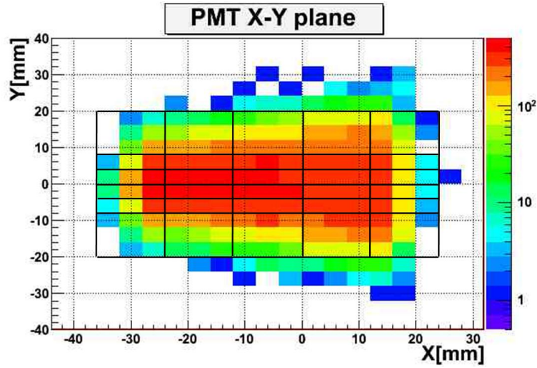
Figure 5.16: One-Spot light distribution on the X-Y photodetector plane: a matrix of 30 PMTs allows to define different sized regions of light collected by PMTs.
