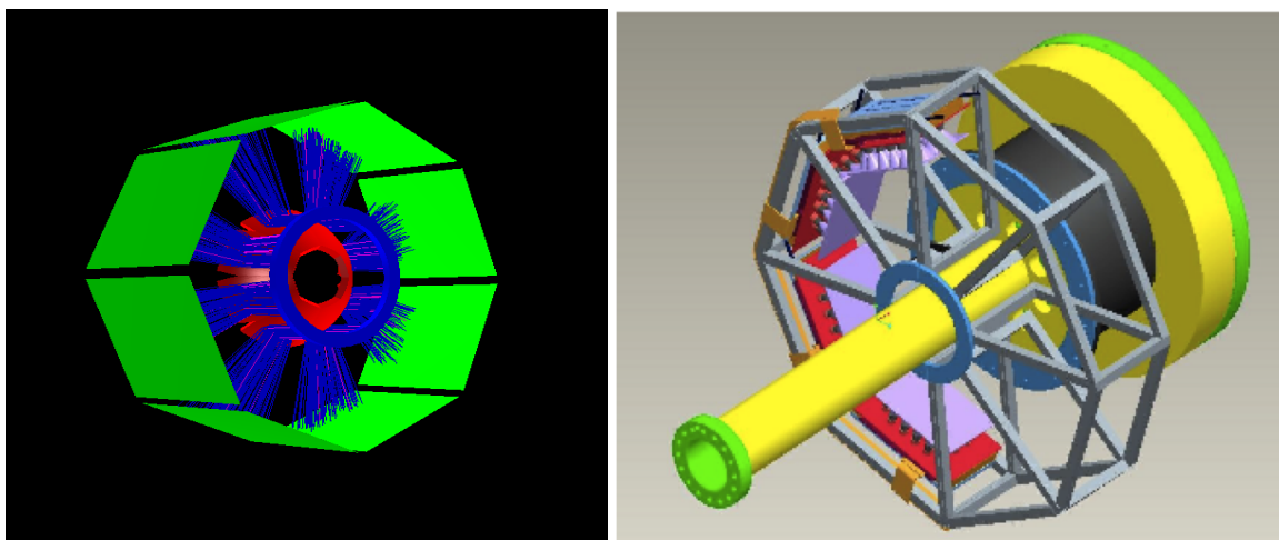
Figure 5.5: Simulation of Cherenkov photons (left-panel) with the ray tracing from the CEDAR quartz windows (blue), to the external mirrors (red) and to the new PMT planes (green). Mechanical design of the new CEDAR photon detector (right-panel) with the main structure positioned after the quartz windows, surrounding the nose and housing external mirrors, light collection cones and PMTs.
