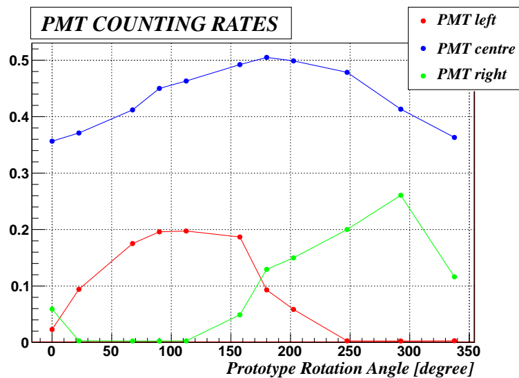
Figure 6.13: New PMTs: study of counting rates vs the orientation of the assembly.
