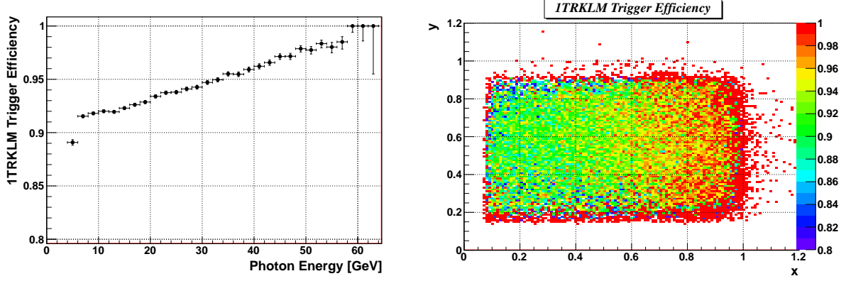
Figure 3.24: The 1TRKLM trigger efficiency vs photon energy in the lab frame (left) and on the (x,y) plot (right) evaluated using the K_{e2\gamma}^+(\text{SD}^+) event selection with no kinematic cuts ( m_{\text{miss}}^2 , x and y ).
