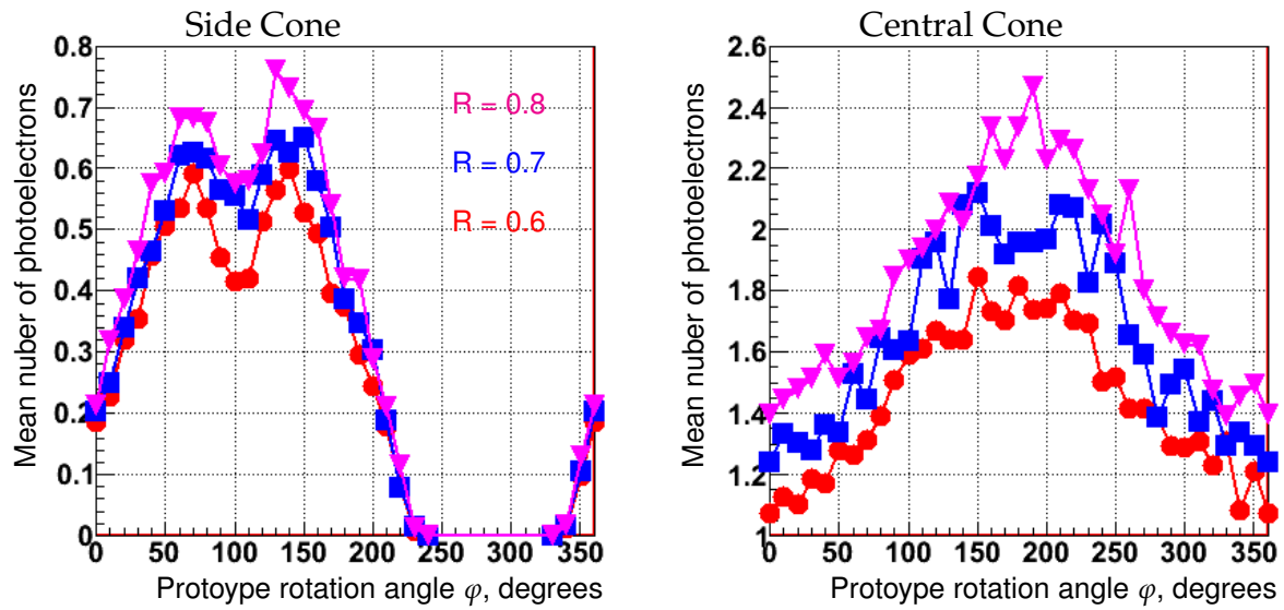
Figure 6.15: MC predictions for mean number of photoelectrons per beam pion, as a function of prototype rotation angle \varphi for different reflectivities ( R ) of the aluminium cones.
