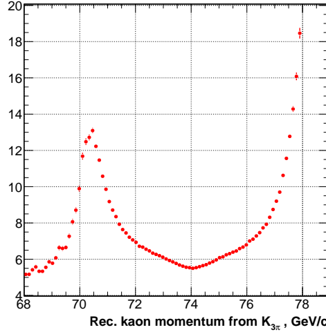
Figure 3.8: Data to MC ratio of the kaon momentum distribution reconstructed using K_{3\pi} events [72]. The formula for the weight is chosen to flatten the parabolic-like shape visible in the distribution.
