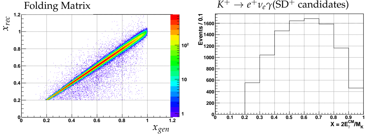
Figure 3.30: (Left) Folding matrix of the x distribution. Events reconstructed with an energy lower than the true energy are visible (mis-reconstructed events). (Right) Distribution of the K_{e2\gamma} candidates over x .
