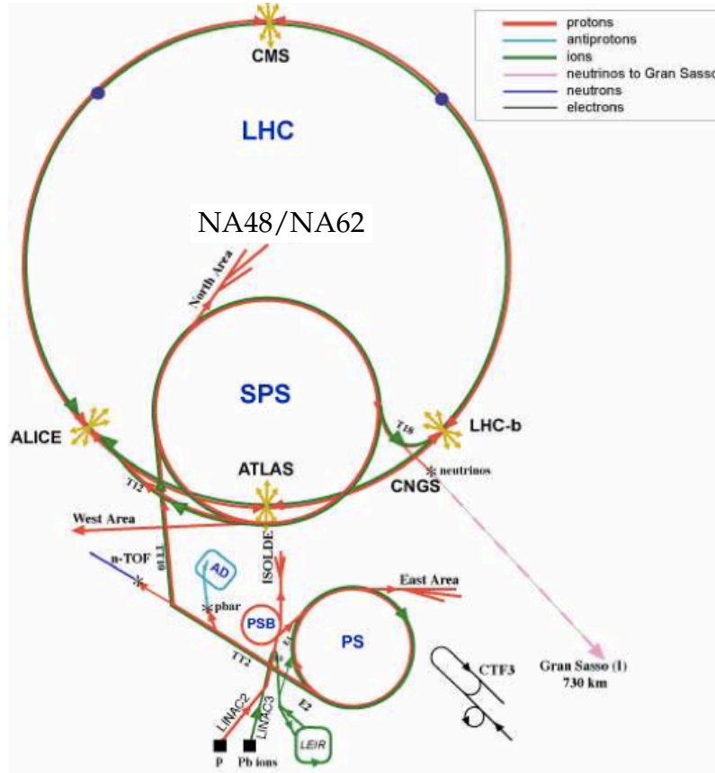
Figure 2.1: Accelerator complex at CERN. The NA62 experiment is located in the North Area of the SPS.
