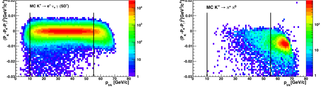
Figure 3.3: Distributions of m_{miss}^2 = (P_K - P_e - P_\gamma)^2 vs the p_{trk} for K_{e2\gamma}^+ (left, signal) and K^+ \rightarrow \pi^+\pi^0 (right, background) MC events. The difference in the spectra suggests a cut on the track momentum in the range (10,55) \text{GeV}/c (see arrows) in order to minimise the background contamination from K^+ \rightarrow \pi^+\pi^0 events.
