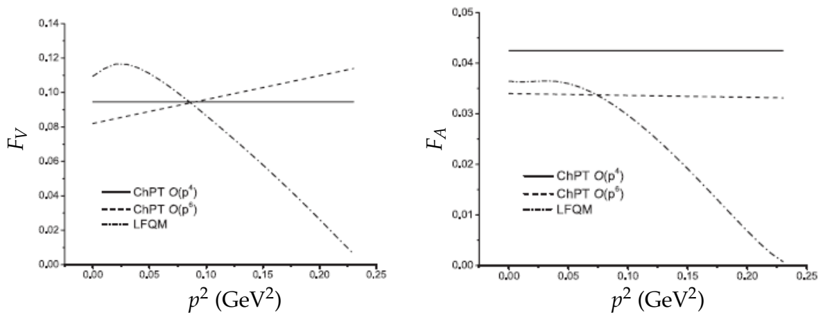
Figure 1.3: Theoretical predictions in \chi PT at \mathcal{O}(p^4) , \mathcal{O}(p^6) and LFQM for F_V (left) and F_A (right) as a function of the squared momentum transfer [9].
