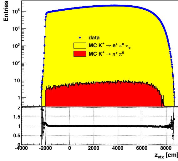
Figure 3.14: Reconstructed z_{vtx} distributions of K^+ \rightarrow \pi^0 e^+ \nu_e candidates compared with the sum of normalised estimated signal and background components (logarithmic scale). Data/MC ratio shows that the agreement fails for resolution effects outside the signal region: -2000 \text{ cm} < z_{vtx} < 8000 \text{ cm} .
