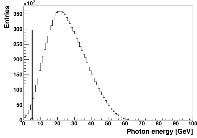
Figure 3.5: Photon energy distribution for K_{e2\gamma}^{+}(SD^{+}) MC events in the lab. frame. The arrow represents the lower cut applied in the event selection.
