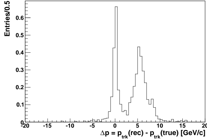
Figure 3.26: \Delta p = p_{trk}(rec) - p_{trk}(true) for K_{2\pi} MC events passing the signal event selection (no E_{LKr}/p_{ptrk} cut applied).
