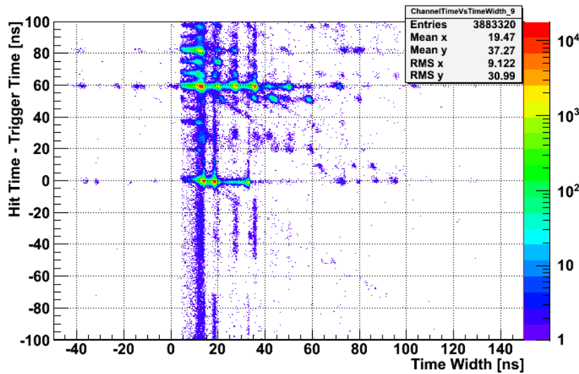
Figure 6.20: Signal time vs time width (trailing - leading) distributions for one new PMT.
