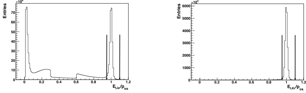
Figure 3.4: E_{LKr}/p_{trk} distributions for data (left) and K_{e2\gamma}^{+} ( SD^{+} ) MC events (right) passing the charged-track selection cuts described in Sec. 3.1.2. The depletion of events in the region 0.3 < E_{LKr}/p_{trk} < 0.6 , outside the signal region, is due to a trigger feature and is known from previous analyses. The arrows represent the cuts applied in the event selection to identify positrons.
