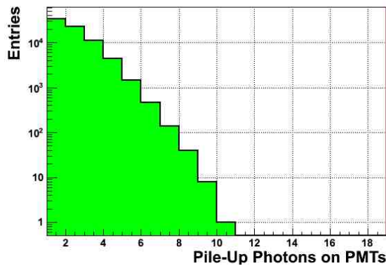
Figure 5.18: Pile-up photons on PMTs within the same kaon event.
