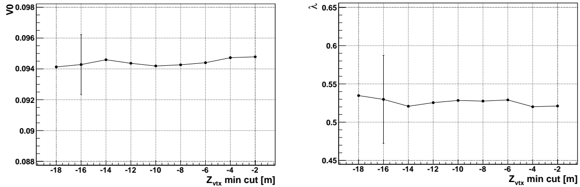
Figure 3.38: Stability check of the form factor parameters on the lower limit of the Z_{vtx} cut. The variations of V_0 and \lambda are within the statistical errors associated for the nominal lower cut: Z_{vtx} = -16 \text{ m} . No systematic uncertainties are considered.
