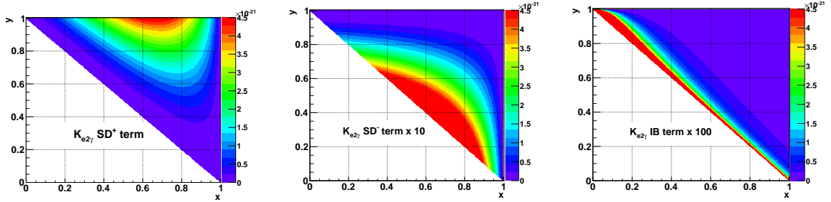
Figure 1.2: Contributions to the differential decay rate d^2\Gamma(K_{e2\gamma}^+)/dxdy (expressed in GeV) from the SD^+ (left), SD^- (centre) and IB (right) terms at \mathcal{O}(p^6) in \chi PT .
