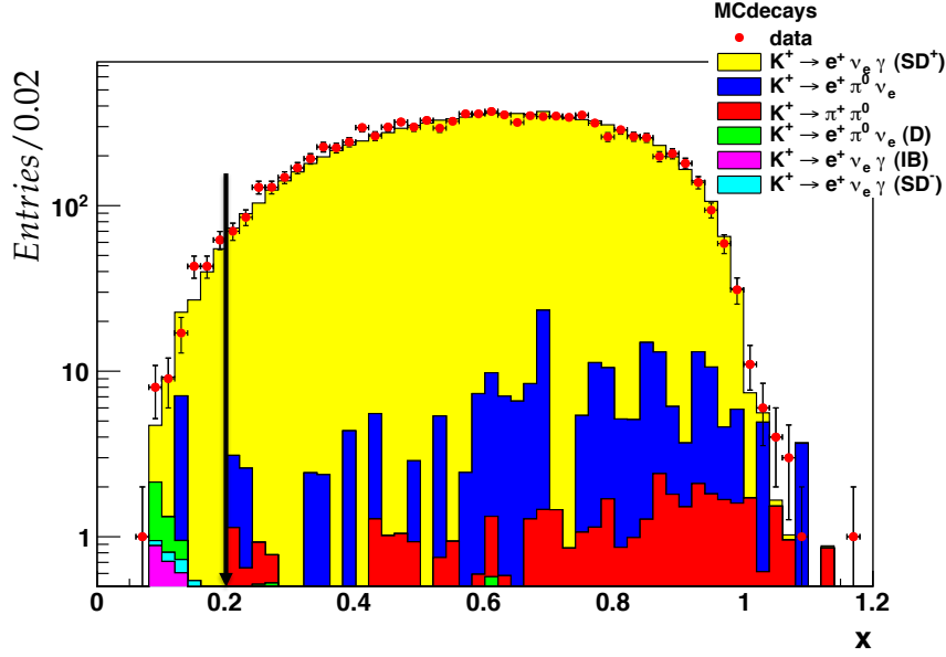
Figure 3.36: Reconstructed x distributions of K_{e2\gamma}^{+} ( SD^2 ) candidates compared with the sum of normalised estimated signal and background components (logarithmic scale). The x variable is proportional to the photon energy in the kaon rest frame. The arrow represents the lower limit: x = 0.2 applied in the event selection and corresponding to a lower limit on the photon energy in the kaon rest frame of about 50 MeV.
