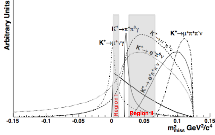
Figure 4.3: Distributions of the m_{miss}^2 variable, as expected under the assumption that the detected charged particle in the final state is a pion, for the signal (solid curve) and the kaon decays not kinematically constrained (dashed curves). The spectra are plotted in arbitrary units and neglecting the resolution effects introduced by the detector. The analysis regions: “Region I” and “Region II” are indicated with grey areas [84].
