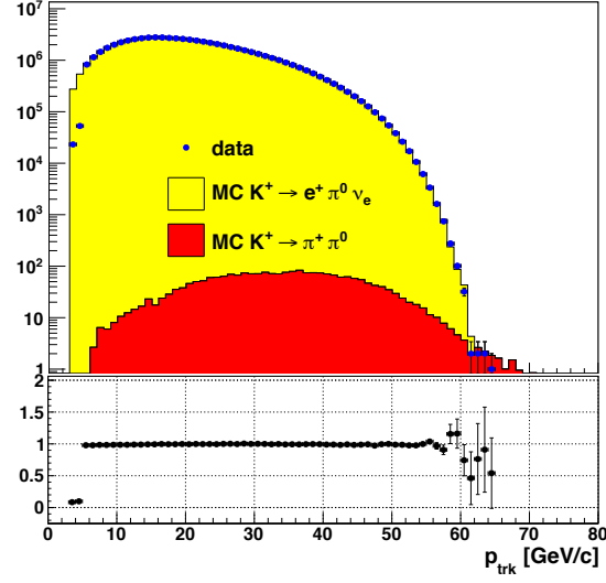
Figure 3.16: Reconstructed track momentum distributions of K^+ \rightarrow \pi^0 e^+ \nu_e candidates compared with the sum of normalised estimated signal and background components (logarithmic scale). Data/MC ratio shows a disagreement for p_{trk} < 5 \text{ GeV}/c , which might be due to low-momentum positrons interacting in the detector material on the beam line.
