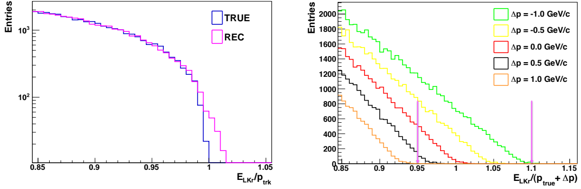
Figure 3.27: Left: simulated E_{LKr}/p_{trk} for “true” and reconstructed variables (log scale). Right: simulated E_{LKr}/(p_{true} + \Delta p) , where \Delta p = -1, -0.5, 0, 0.5, 1 GeV/c. The arrows indicate the “electron-like” region (0.95,1.10).
