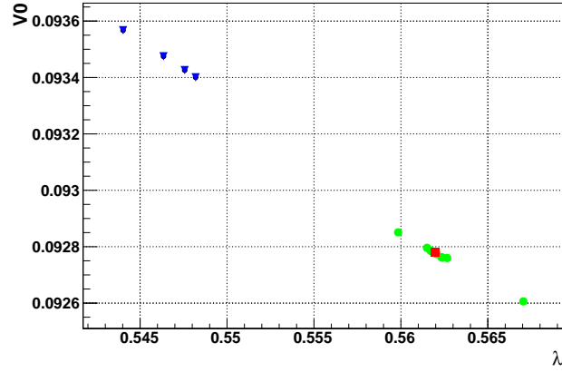
Figure 3.33: (V_0, \lambda) results obtained by correcting the K_{2\pi} and K_{e3} background MC events with a lost photon for the 1TRKLM trigger efficiency dependence on x . The measurements are performed in 9 different kinematic regions of y (green markers), in the whole y spectrum (red marker) and in 4 different kinematic regions of m_{miss}^2 (blue markers).
