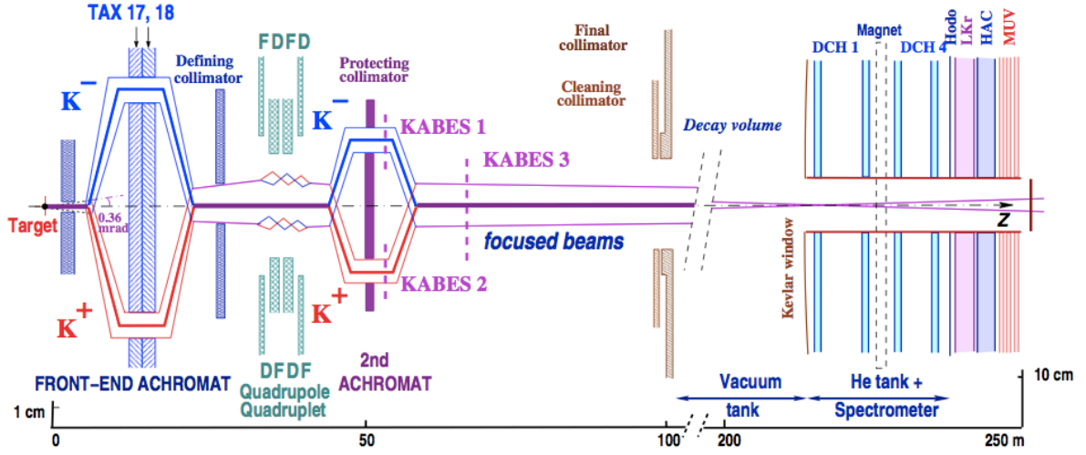
Figure 2.2: The NA48/2 beam line and detector [64, 65].
