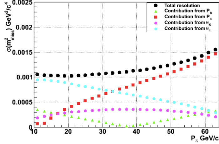
Figure 4.4: The m_{miss}^2 total resolution (black circle) as a function of the pion momentum ( P_\pi ). Single components contributing to the resolution from the measurement of P_K (green triangle), P_\pi (red square), \theta_K (magenta circle) and \theta_\pi (cyan circle), i.e. the kaon and pion momenta and directions, as a function of P_\pi [85].
