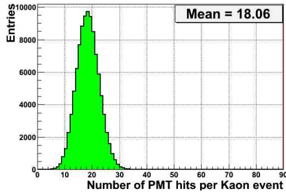
Figure 5.21: Number of photo-electrons detected per kaon event.
