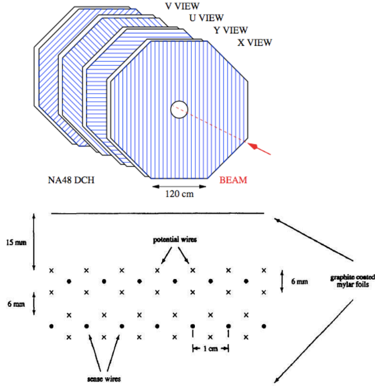
Figure 2.4: NA48 drift chambers (DCHs): (top) X,Y,U,V views; (bottom) geometry of a drift cell.
