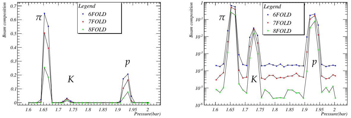
Figure 6.3: Pressure scan over the full range of gas pressures.
