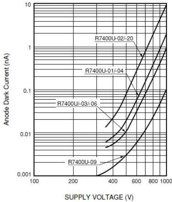
Figure 5.8: HAMAMATSU specification: Anode Dark Current versus the supply voltage applied, each trend corresponding to a different PMT of the R7400/U series [96].
