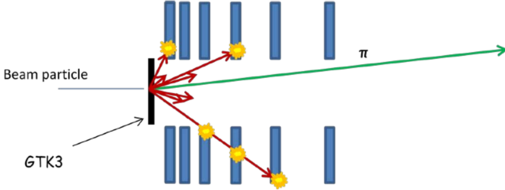
Figure 4.11: Sketch of beam particles undergoing inelastic interactions in the GTK material. The scattered particles are detected in the CHANTI detector placed immediately after GTK3.
