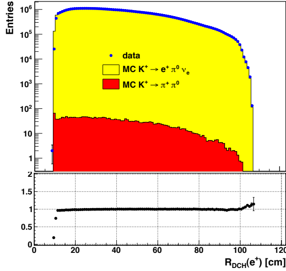
Figure 3.15: Reconstructed positron radius at DCH1, R_{DCH}(e^+) , distributions of K^+ \rightarrow \pi^0 e^+ \nu_e candidates compared with the sum of normalised estimated signal and background components (logarithmic scale). Data/MC ratio shows that the agreement fails for R_{DCH}(e^+) < 12 \text{ cm} , which is understood to be caused by particle interactions in the DCH1 flange.
