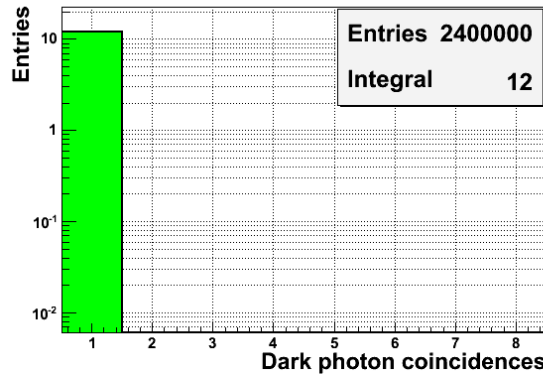
Figure 5.23: Dark photon event coincidences: the first bin is filled if a double coincidence is found.
