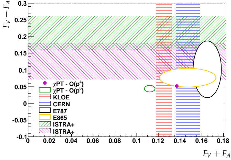
Figure 1.7: Theoretical expectations for F_V \pm F_A in \chi PT at \mathcal{O}(p^4) (magenta marker) and \mathcal{O}(p^6) (green ellipse). Results on the form factor combinations from KLOE [21], CERN [22,23] and ISTRA+ [26,27] collaborations; 1\sigma contours in the (F_V - F_A, F_V + F_A) plane, assuming no correlation, from E787 [24] and E865 [25] experiments at BNL.
