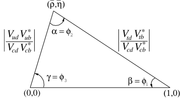
Figure 1.8: Unitarity triangle corresponding to the condition 1.27.
