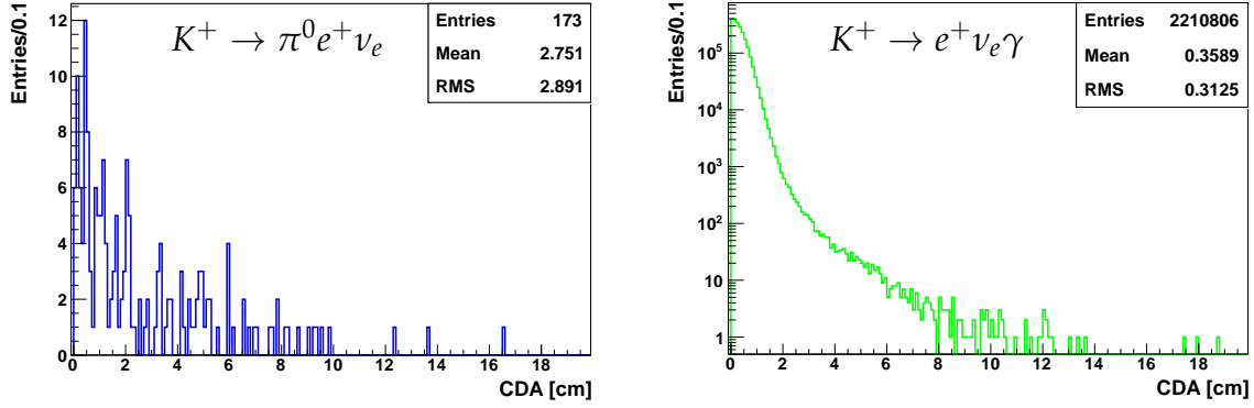
Figure 3.25: CDA distributions for K_{e3} (left, background) and K_{e2\gamma}^+ (right, signal) MC events. The observable is sensitive to MCS of the positron in the kevlar window and DCH1; the difference in the mean value of one order of magnitude confirms large MCS as the origin of K_{e3} events passing the signal selection.
