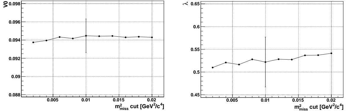
Figure 3.40: Stability check of the form factor parameters on the |m_{miss}^2| cut. The variations of V_0 and \lambda are within the statistical errors associated for the nominal cut: |m_{miss}^2| < 0.01 \text{ GeV}^2/c^4 . No systematic uncertainties are considered.
