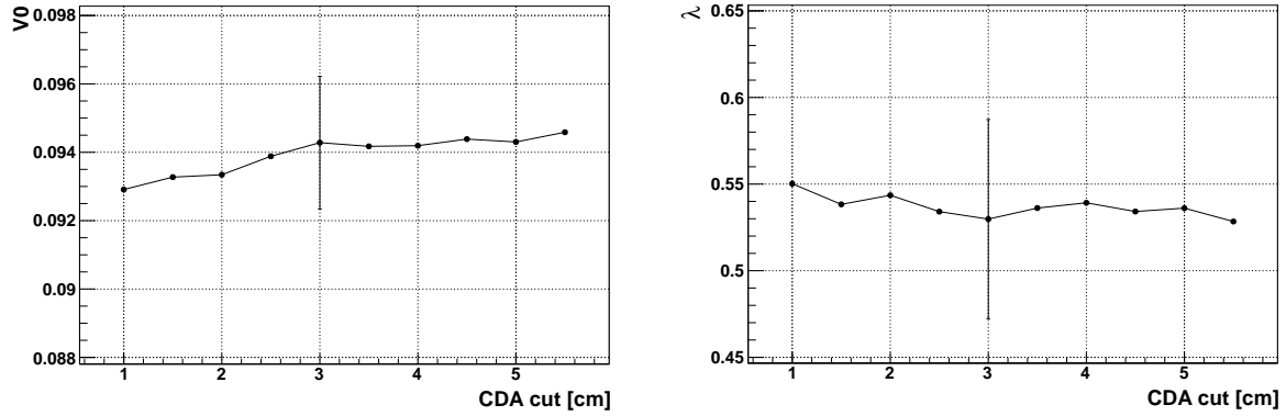
Figure 3.37: Stability check of the form factor parameters on the CDA cut. The variations of V_0 and \lambda are within the statistical errors associated for the nominal upper cut: \text{CDA} = 3 \text{ cm} . No systematic uncertainties are considered.
