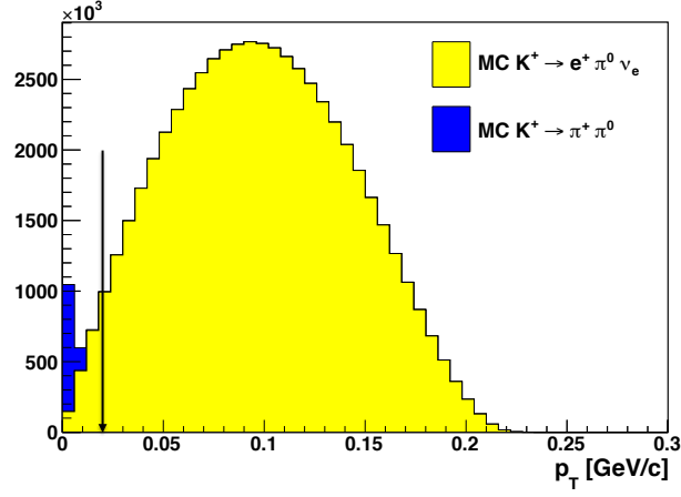
Figure 3.12: p_T distributions for K^+ \rightarrow \pi^0 e^+ \nu_e (signal, yellow) and K^+ \rightarrow \pi^+ \pi^0 (background, blue) MC events. The difference in the spectra suggests for the signal selection a cut at p_T > 0.02 GeV/ c in order to reject the background contamination from K^+ \rightarrow \pi^+ \pi^0 events.
