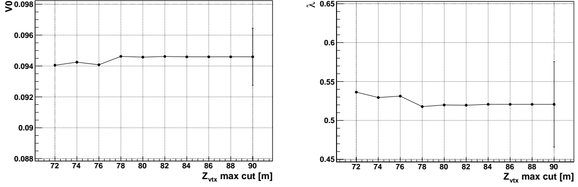
Figure 3.39: Stability check of the form factor parameters on the upper limit of the Z_{vtx} cut. The variations of V_0 and \lambda are within the statistical errors associated for the nominal upper cut: Z_{vtx} = 90 m. No fluctuations are observed in the last 4 points because the Z_{vtx} distribution for signal events at the end of the selection ends at 80 m. No systematic uncertainties are assigned.
