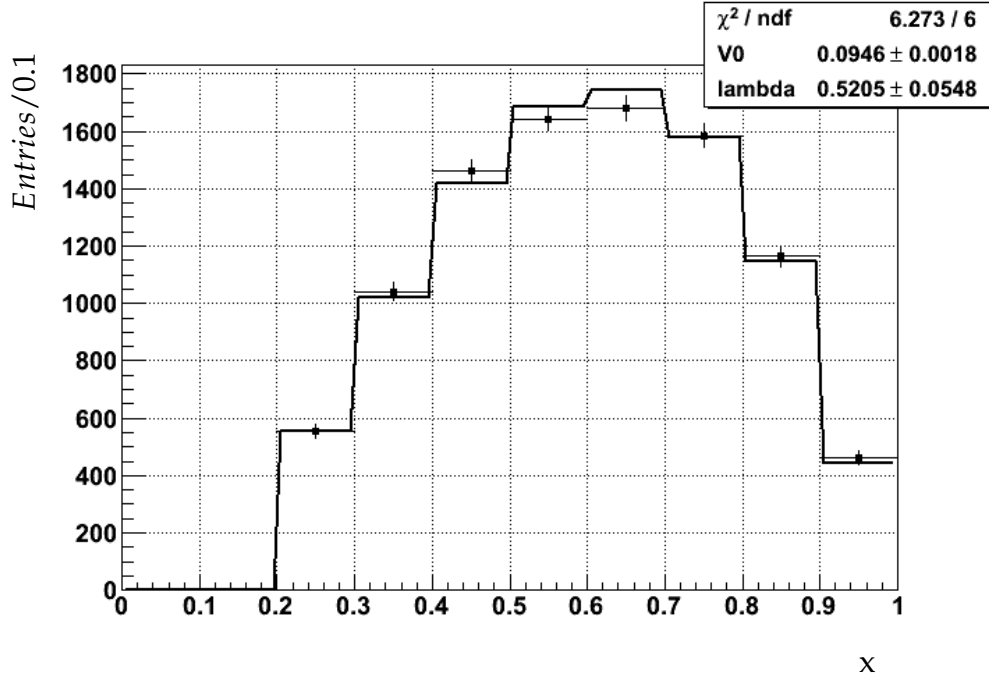
Figure 3.41: Fit to \chi PT at \mathcal{O}(p^6) . The fit parameters are the vector form factor V_0 and the “slope” \lambda , while the axial form factor is fixed to its \mathcal{O}(p^6) value F_A(q^2) = F_A(0) = 0.034 .
