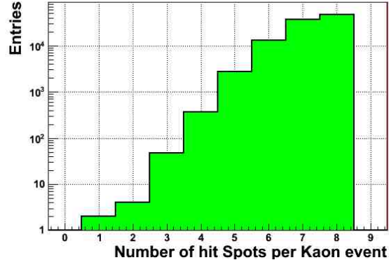
Figure 5.22: Number of hit spots per kaon event.
