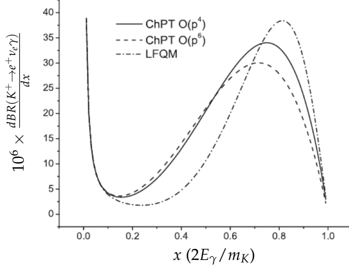
Figure 1.6: Theoretical predictions for the differential branching ratio of K_{e2\gamma}^+ as functions of x in LFQM (dashed-dotted line), in \chi PT at \mathcal{O}(p^4) (solid line) and \mathcal{O}(p^6) (dashed line).
