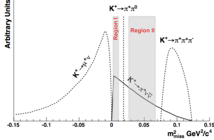
Figure 4.2: Distributions of the m_{miss}^2 variable, as expected under the assumption that the detected charged particle in the final state is a pion, for the signal (solid curve) and the kaon decays kinematically constrained (dotted curves). The spectra are plotted in arbitrary units and neglecting the resolution effects introduced by the detector. The K^+ \rightarrow \pi^+ \pi^0 kinematic signature forces the analysis region to be split into two parts: “Region I” and “Region II” (grey areas) [84].
