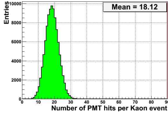
Figure 5.20: Number of photo-electrons detected per kaon event.
