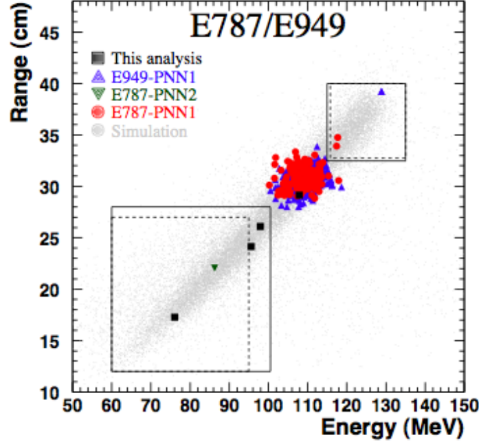
Figure 1.11: Distribution of the pion range as a function of the pion kinetic energy for events passing the K^+ \rightarrow \pi^+ \nu \bar{\nu} analysis event selection. The square markers represent the events observed by E949 [58] (source of the plot) in \pi \nu \bar{\nu}(2) . The downward-pointing triangle marker represents the event observed by E787 in the same region. The circle and upward-pointing triangle markers represent the events selected by E787 and E949 in \pi \nu \bar{\nu}(1) . The solid (dashed) lines represent the limits of the \pi \nu \bar{\nu}(1) and \pi \nu \bar{\nu}(2) signal regions for the E949 (E787) analyses. The markers outside the boxes correspond to K^+ \rightarrow \pi^+ \pi^0 events surviving the photon veto cuts and passing the analysis event selection. The light gray points are simulated K^+ \rightarrow \pi^+ \nu \bar{\nu} events.
