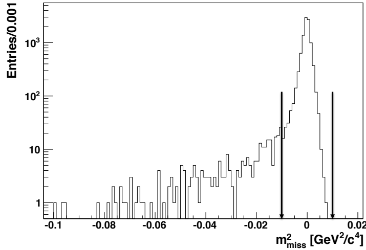
Figure 3.10: Squared missing mass m_{miss}^2 distribution for data (log scale). The complete list of cuts for the charged-track, photon and kinematic selections of K_{e2\gamma}^+ ( SD^2 ) events is applied. The arrows represent the m_{miss}^2 cut chosen for the event selection.
