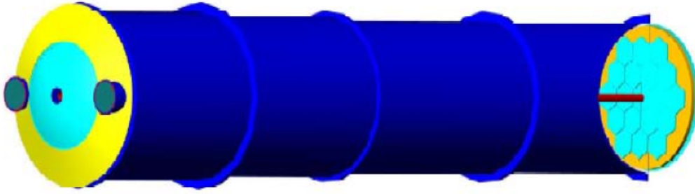
Figure 4.8: Schematic layout of the NA62 RICH detector: the right section of the vessel is cut to show the spherical mirror and the beam pipe.
