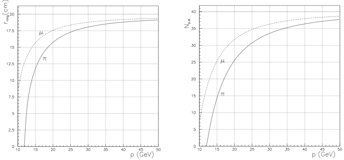
Figure 4.9: Ring radius (left) and N_{pe} (right) as a function of momentum, for a pion (solid line) and a muon (dashed line), for a RICH filled with Neon at 1 atm and with focal length of 17 m.
