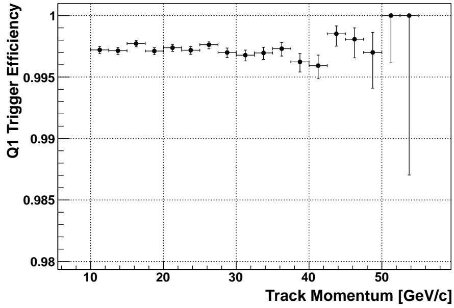
Figure 3.19: The Q1 trigger efficiency as a function of the track momentum measured using K_{e3} events.
