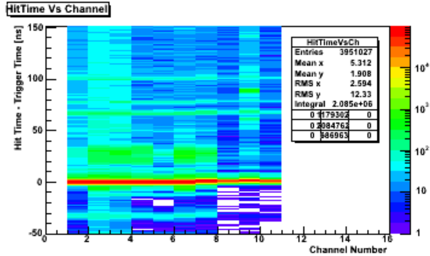
Figure 6.18: Signal time distributions with respect to the trigger time: standard PMTs in channels 1 – 7 and new PMTs in channels 8 – 10.
