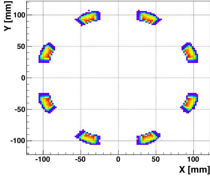
Figure 5.4: Cherenkov light distribution at the eight CEDAR quartz windows.
