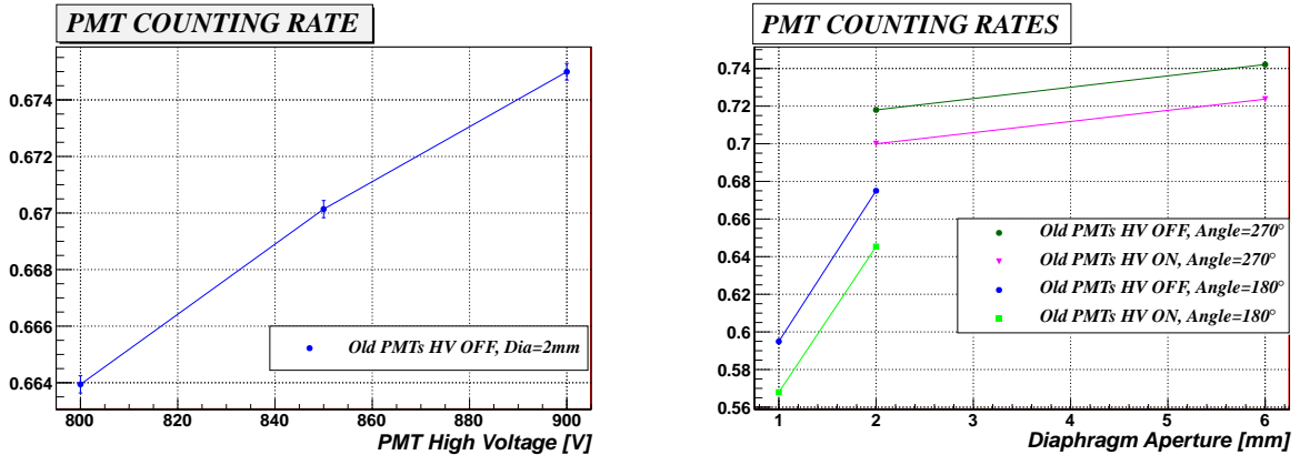
Figure 6.12: Left: new-PMT high voltage scan. Right: new-PMT response dependence on the diaphragm aperture w_D .
