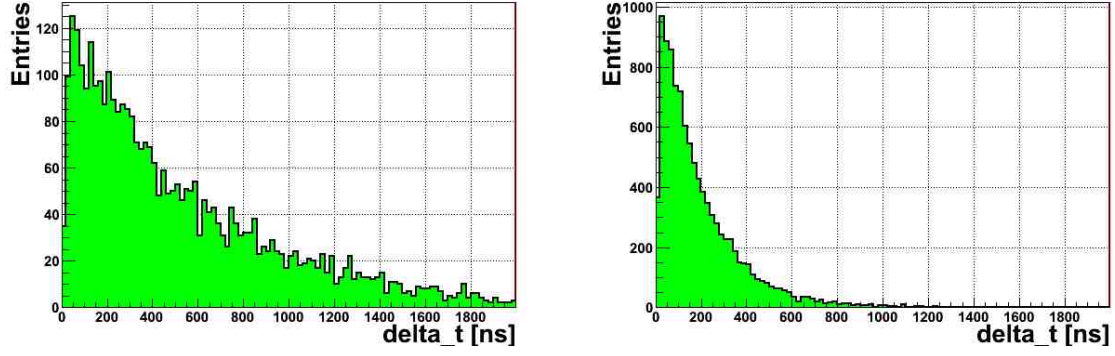
Figure 5.17: Photon arrival time distribution for PMTs collecting light from the border (a) and the central (b) parts of the spot.
