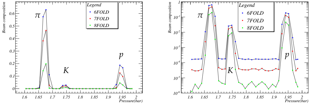
Figure 6.22: Pressure scan over the full range of gas pressures.
