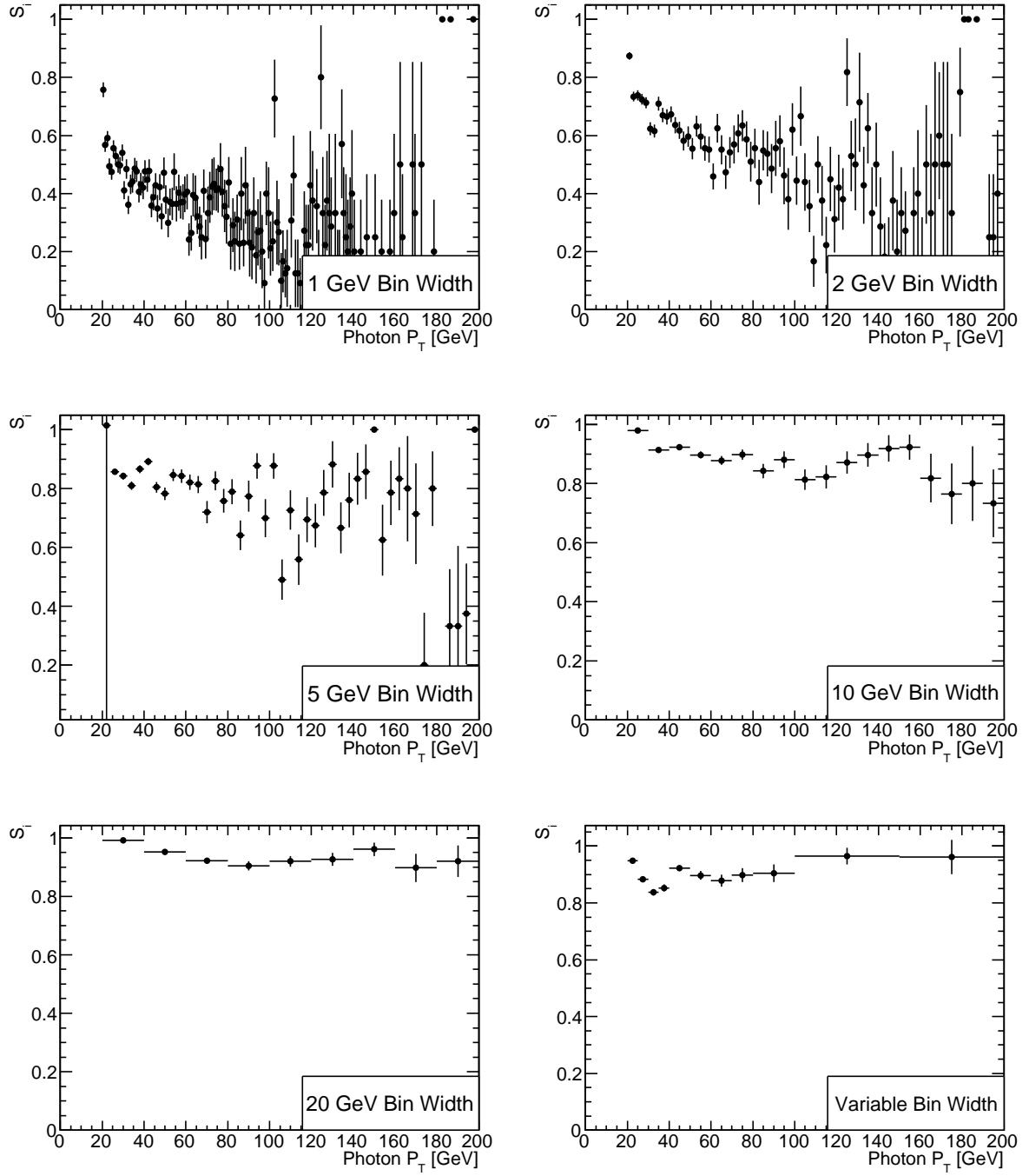
Figure 5.14: Photon p_T bin width stability for various bin widths, including the final choice of variable bin width: [20–25], [25–30], [30–35], [35–40], [40–50], [50–60], [60–70], [70–80], [80–100], [100–150], and [150–200+] GeV bins.
