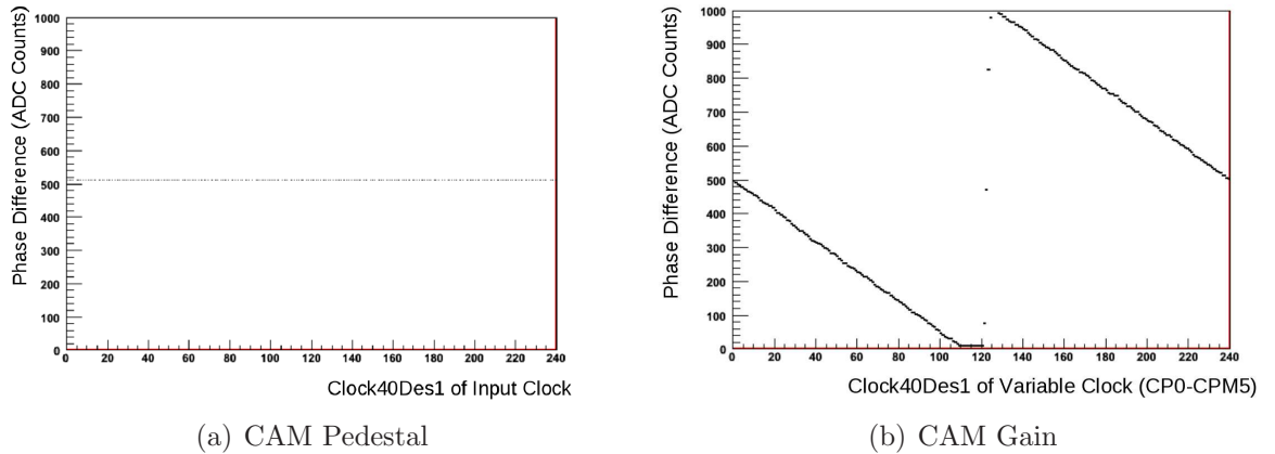
Figure 3.10: (a) An example CAM pedestal result, showing the value of the phase difference (in ADC counts) for two “in-phase” clocks. (b) The ADC response to the phase difference between clocks, when one clock is cycled through its whole phase ( 2\pi ), and the reference clock kept constant.
