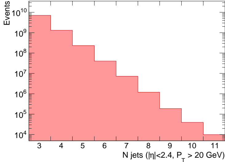
Figure 5.2: The expected number of events containing N jets ( |\eta| < 2.4 , p_T > 20\text{GeV} ), derived from the JF17 di-jet Monte Carlo sample, normalised to an integrated luminosity of \mathcal{L} = 1\text{fb}^{-1} .
