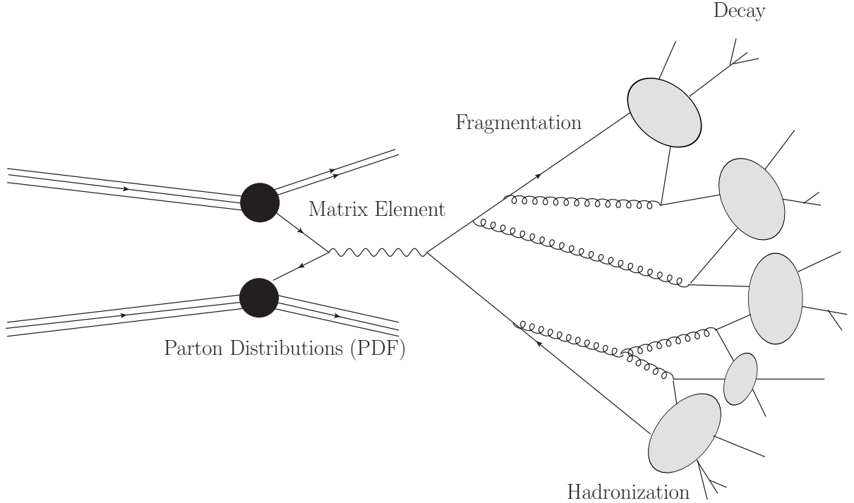
Figure 1.2: Schematic representation of the processes simulated in a Monte Carlo generator such as Pythia .
