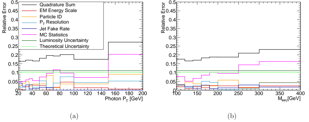
Figure 5.26: (a) Breakdown of systematic uncertainties, and quadratic total sum for p_T(\gamma) distribution. (b) M_{ee\gamma} distribution.
