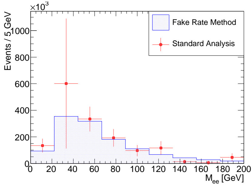
Figure 5.9: Comparison of the invariant mass of “Loose” di-electron pairs derived using the fake-rate method, and using the standard analysis routine, for binned J0 - J4 di-jet samples, normalised to \mathcal{L} = 1\text{fb}^{-1} integrated luminosity. The structure in the statistical errors originates from the fact that the distributions are the sum of the binned di-jet distributions, each having a different normalisation factor.
