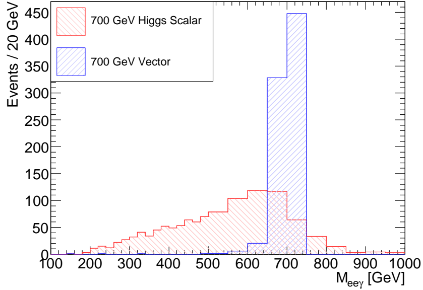
Figure 5.29: Reconstructed M_{ee\gamma} for a 700 GeV scalar Higgs, and vector particle decays, with 5,000 events.
