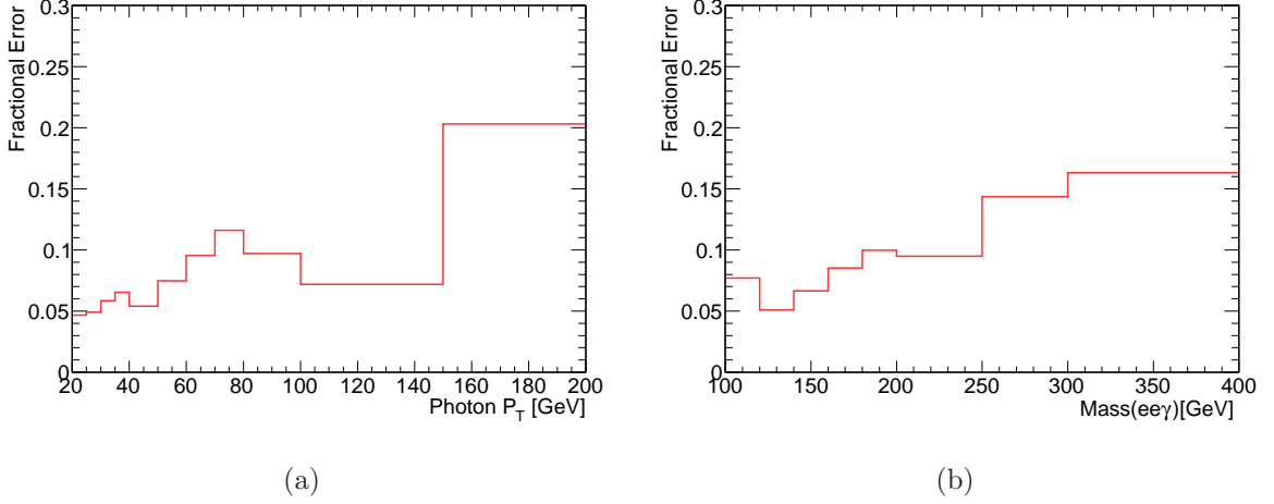
Figure 5.24: (a) Systematic effect of Monte-Carlo statistics in p_T(\gamma) distribution. (b) M_{ee\gamma} distribution.
