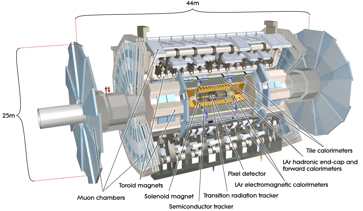
Figure 2.2: The ATLAS detector[30].
