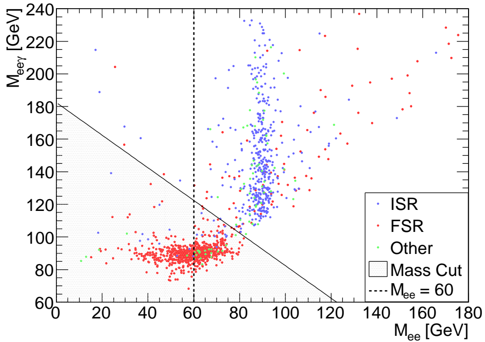
Figure 5.13: M_{ee} versus M_{ee\gamma} for ISR, FSR and Fake photons, with selection cut M_{ee\gamma} > (2M_Z - M_{ee}) overlaid, for an expected integrated luminosity of \mathcal{L} = 5\text{fb}^{-1} .
