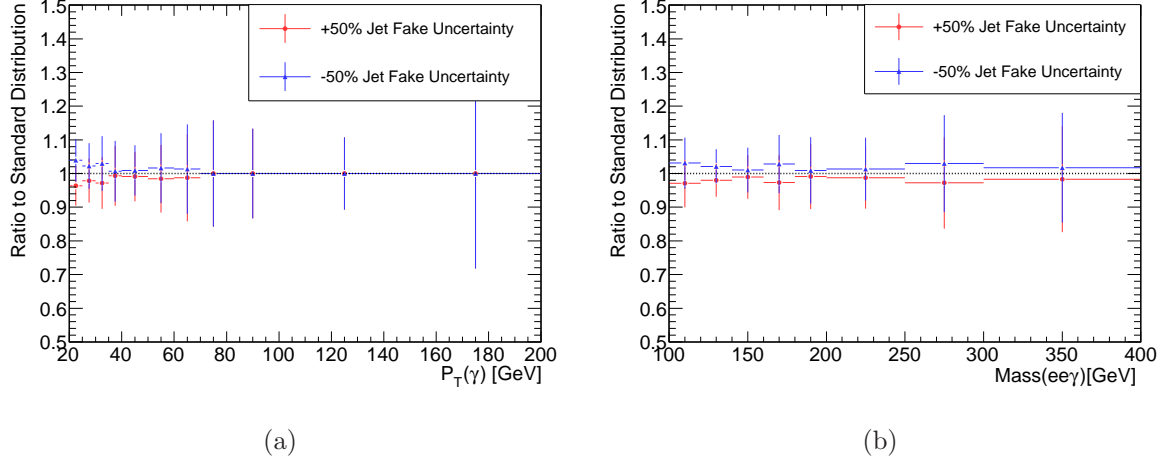
Figure 5.23: (a) Systematic effect of a \pm 50\% uncertainty in the photon fake-rate, binned in p_T(\gamma) . (b) M_{ee\gamma} distribution.
