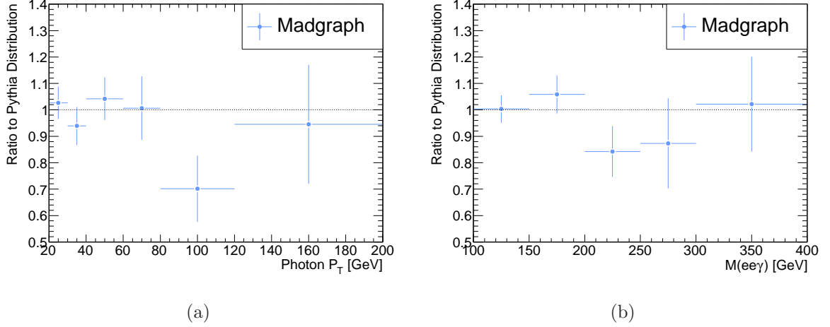
Figure 5.25: (a) The ratio of Madgraph to Pythia ISR differential cross-section predictions, in p_T(\gamma) . (b) Ratio of M_{ee\gamma} distributions, statistical errors only.
