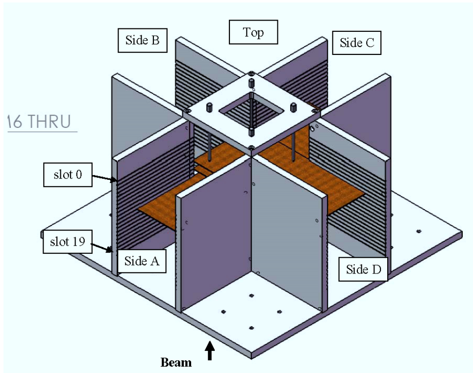
Figure 7.2: Test stand used for TPAC 1.2 test beam.
