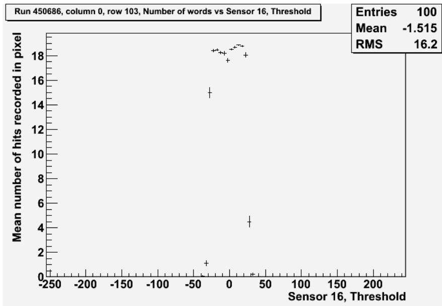
Figure 5.6: A sample threshold scan histogram for an active pixel in the shaper region of the sensor. For every threshold scan run 28224 pixel threshold scan histograms were produced of which 672 were scans of active pixels and 336 of those active pixels were shaper pixels. In the whole sensor there were 14112 shaper pixels and they commonly displayed the 'flat-top' distribution shown in the threshold scan above. It is likely that this distribution is in fact a gaussian distribution similar to the one shown in figure 5.5 with the 'flat-top' created by the pixel becoming saturated at 19 hits. All threshold measurements are in TU.
