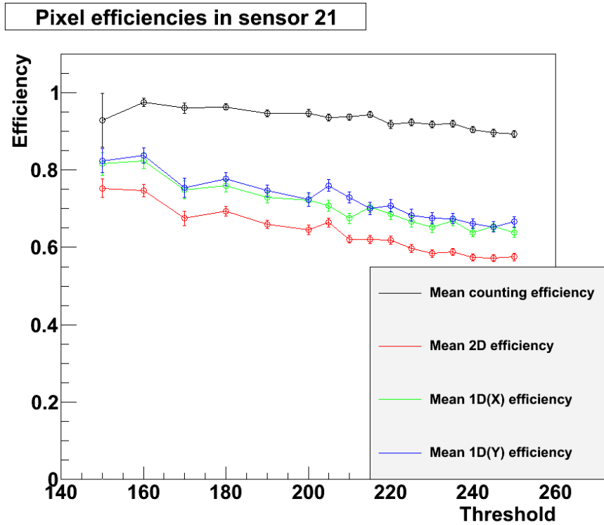
Figure 7.37: Pixel efficiencies in test sensor 21, averaged from several runs in the test beam. The counting method efficiencies were calculated using a three \sigma search range.
