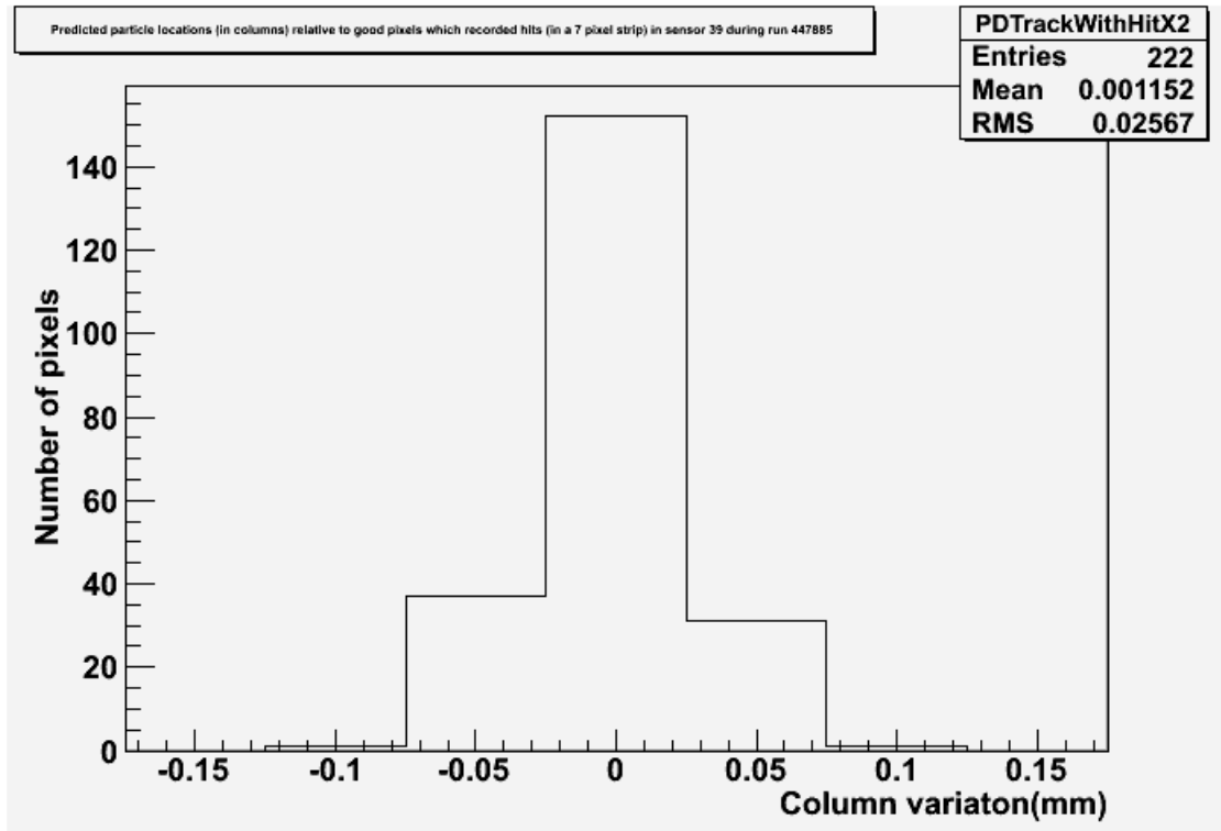
Figure 7.30: An example of the 1D histograms produced to record the particle track positions relative to the centres of nearby pixels which recorded hits in a typical run.
