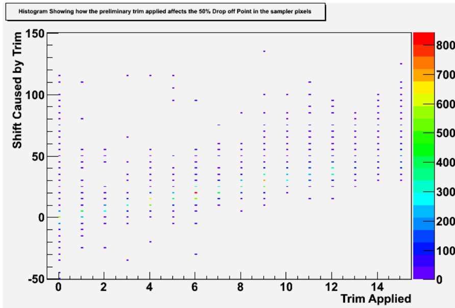
Figure 5.16: A plot showing the shifts in pixel 50% drop off points in sampler pixels in sensor 16 caused by applying different trim settings. This data was collected by comparing run set 450674 to 450715 (untrimmed) to run set 452056 to 452097 (trim based on 50% drop off point, separate targets for shapers and samplers, trim range assumed to be 100TU). All threshold measurements are in TU.
