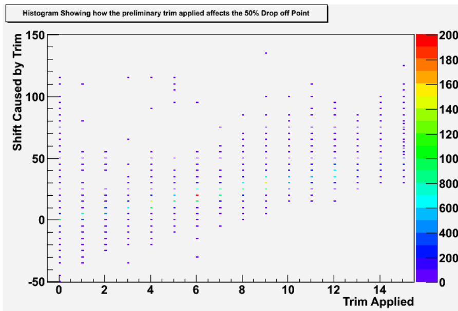
Figure 5.14: A plot showing the shifts in pixel 50% drop off points in sensor 16 caused by applying different trim settings. This data was collected by comparing run set 450674 to 450715 (untrimmed) to run set 452056 to 452097 (trim based on 50% drop off point, separate targets for shapers and samplers, trim range assumed to be 100 threshold units). Equivalent histograms showing only results from either shaper or sampler pixels are shown in figures 5.15 and 5.16 respectively. All threshold measurements are in TU.
