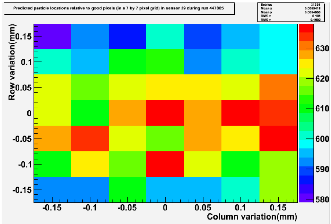
Figure 7.26: An example of the 2D histograms produced to record particle track postions relative to the centres of nearby pixels in a typical run (447885).
