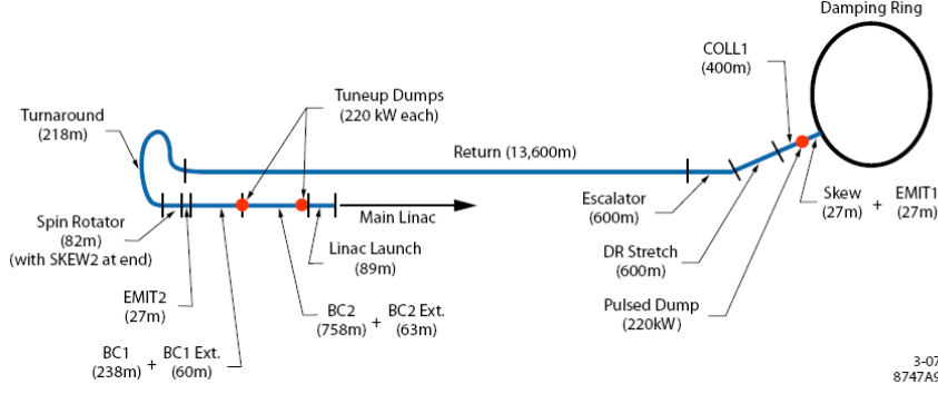
Figure 2.3: A diagram showing the layout of the proposed ILC ring to main linac system (RTML)[14].
