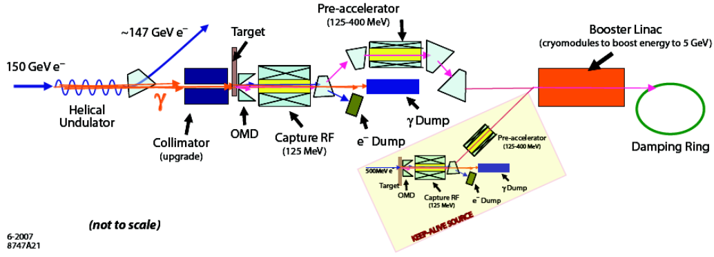
Figure 2.2: The proposed layout of the ILC positron source[14].
