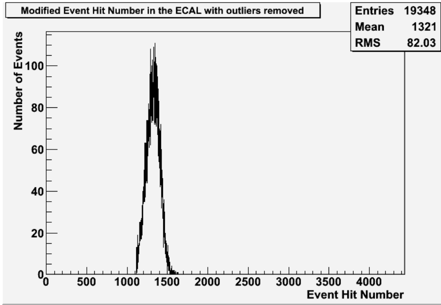
Figure 6.25: A sample histogram showing the distribution of the number of hits recorded in a simulated MAPS (digital) ECAL in single events. These hit numbers are modified so that hits recorded in the outer ECAL are doubled. Additionally the hit number distribution shown in this histogram has been modified to exclude all events where the number of hits recorded is more than the (unaltered) mean plus two (unaltered) standard deviations or less than the (unaltered) mean minus one (unaltered) standard deviation. The unmodified distribution used to produce this histogram is shown in figure 6.23. Each event in this distribution corresponds to a 15.78 GeV photon passing through the ECAL.
