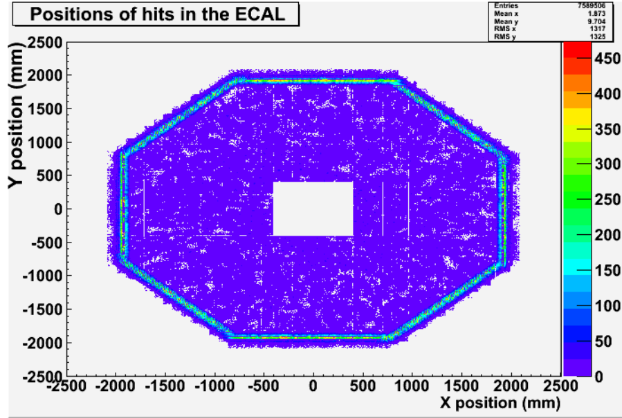
Figure 6.11: A sample hit map showing the distribution of all hits recorded in a simulated analogue ECAL during 20000 simulated 15.78 GeV photon events. This diagram shows the ECAL as it would be seen from further along the beam line (i.e. the beam is perpendicular to the page), X and Y are arbitrary directions perpendicular to the beam line and perpendicular to each other. The distribution of hits implies that the particle showers simulated were contained within the ECAL.
