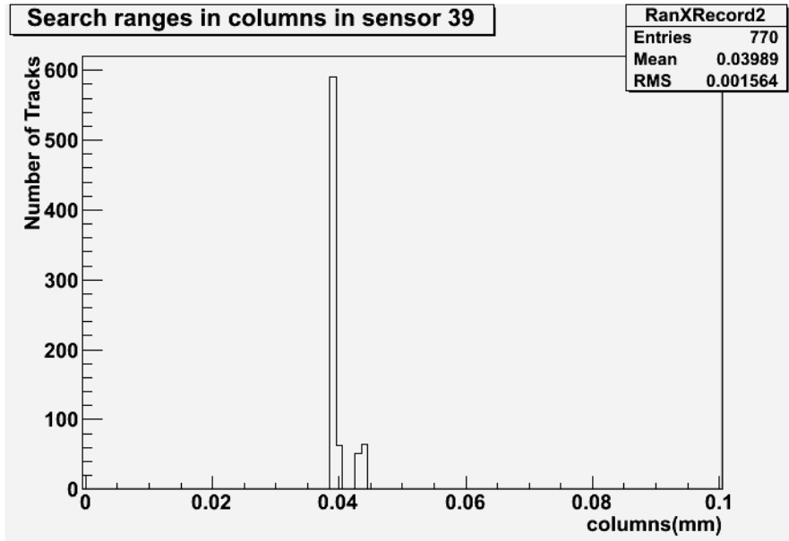
Figure 7.20: An example of one \sigma search ranges for the counting method, in columns, for sensor 39. This data was recorded during run 447885. Note: All search ranges were increased by 25\mu\text{m} to ensure that if the initial search range encompassed any part of a pixel, the search range eventually used would encompass the centre of that pixel (and therefore any hits recorded in that pixel). This histogram shows the final search ranges used.
