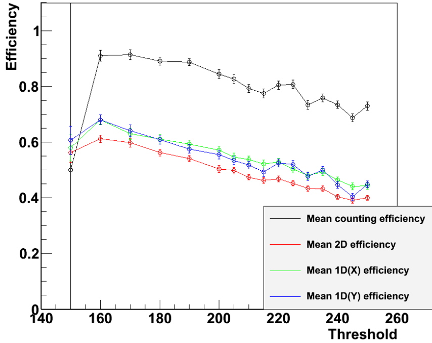
Figure 7.40: Pixel efficiencies in test sensor 39, averaged from several runs in the test beam. The counting method efficiencies were calculated using a three \sigma search range.
