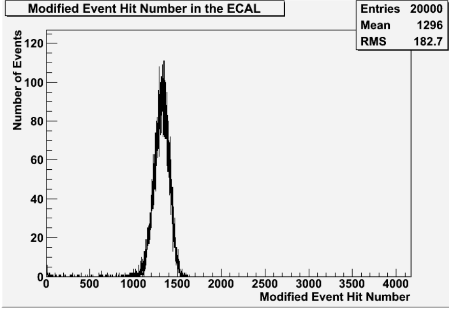
Figure 6.23: A sample histogram showing the distribution of the number of hits recorded in a simulated MAPS (digital) ECAL in single events. These hit numbers are modified so that hits recorded in the outer ECAL are doubled. Each event in this distribution corresponds to a 15.78 GeV photon passing through the ECAL.
