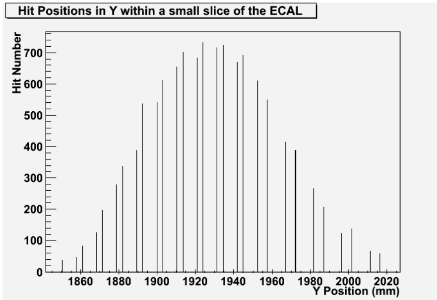
Figure 6.10: A sample histogram showing the distance in the Y direction between hits in a small segment of the analogue ECAL in the extreme positive Y direction (see figure 6.2 for the region used). This shows the distance between separate layers in the ECAL. The simulations used to produce this histogram used 15.78 GeV photons.
