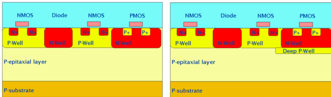
Figure 3.5: Vertical section of a standard CMOS wafer (distances not to scale), unmodified (left), and modified to include Deep P-Wells (DPW) to mask PMOS transistors(right)[32].
