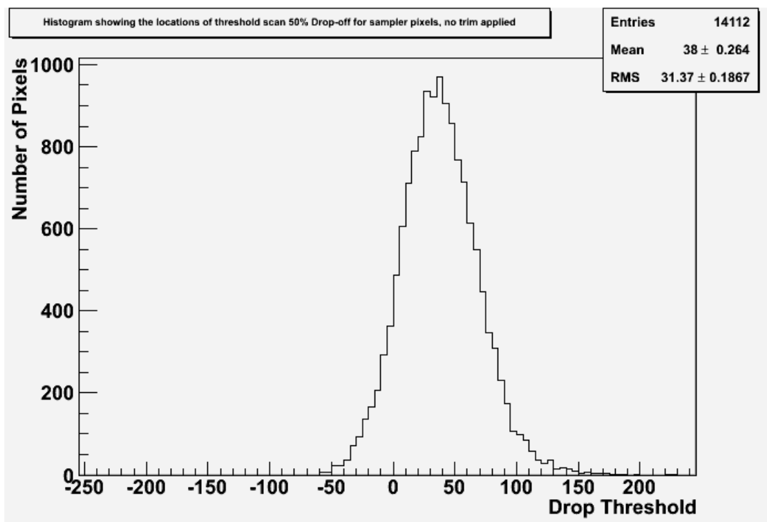
Figure 5.12: A plot showing the distributions of 50% drop-off points of sampler pixels in sensor 16 with no trim applied. All threshold measurements are in TU.
