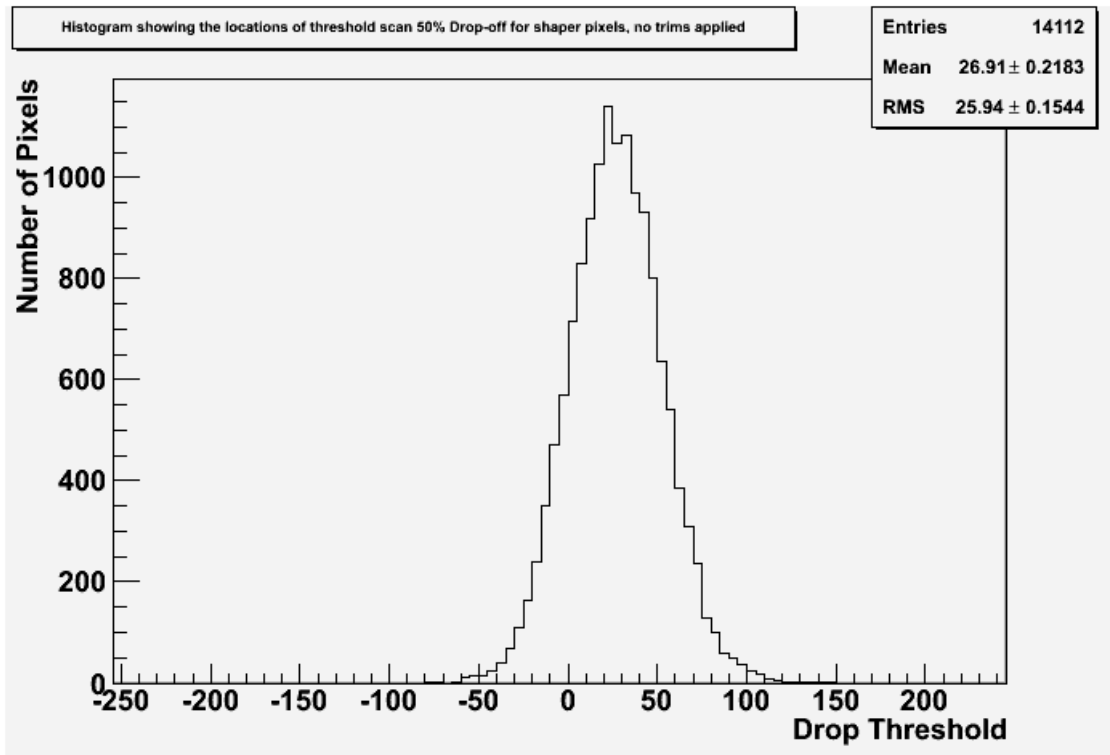
Figure 5.10: A plot showing the distributions of 50% drop-off points of shaper pixels in sensor 16 with no trim applied. All threshold measurements are in TU.
