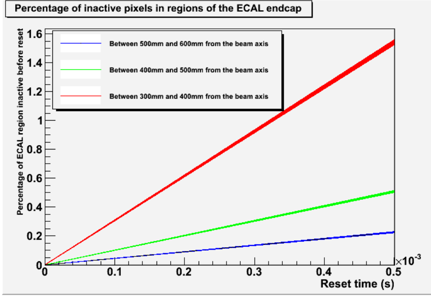
Figure 4.12: Variation in percentage of pixels inactive in ECAL endcap with reset time and location relative to the beam. The maximum reset/readout interval shown is the same order of magnitude as the time taken for a single bunch train passing through the detector[14].
