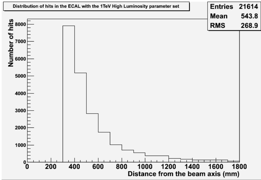
Figure 4.4: A sample histogram showing the distribution of hits in the LDC01 ECAL endcap relative to the beam axis recorded after a single bunch crossing using the 1TeV High Luminosity parameter set. Note: this distribution does have a minimum hit energy cutoff of 3 \times 10^{-6} GeV.
