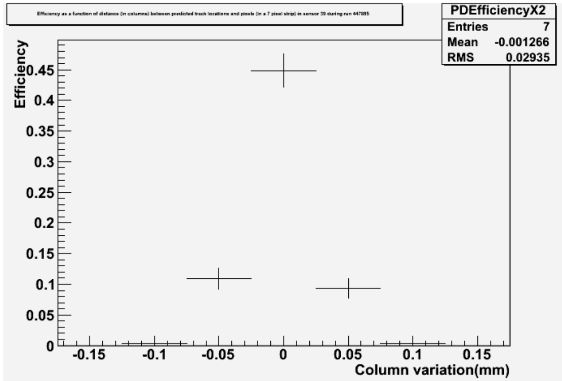
Figure 7.31: An example of the 1D histograms produced to record the variation in apparent pixel efficiency of pixels near to a particle track in a typical run.
