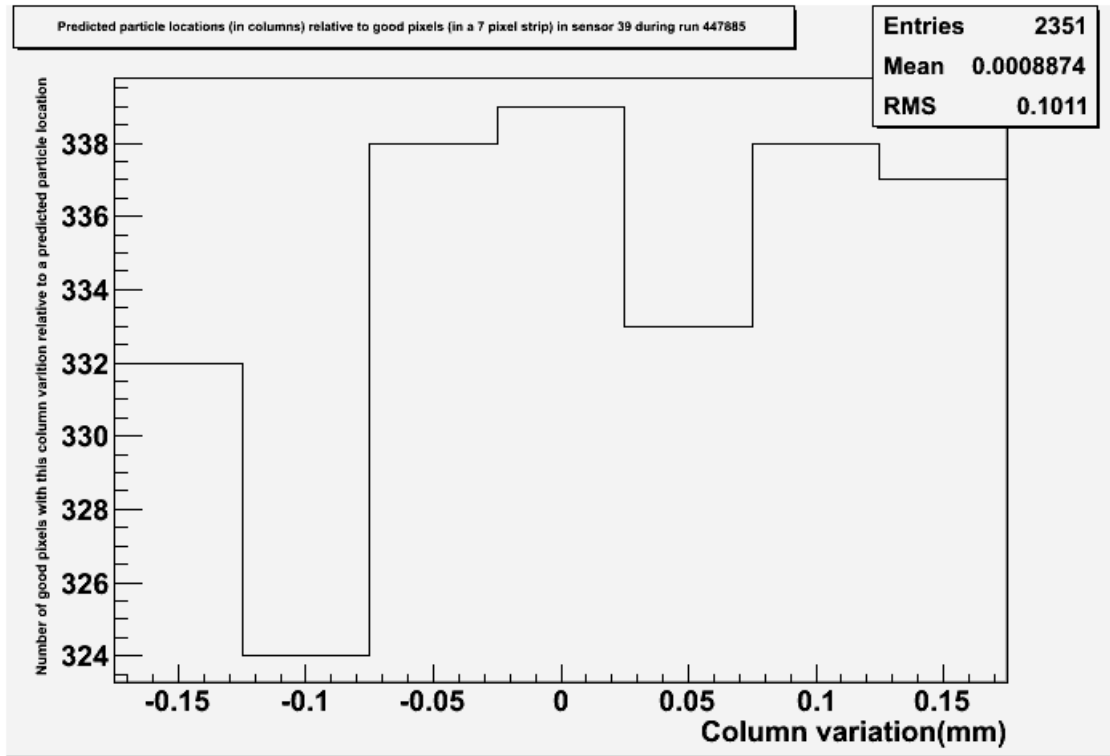
Figure 7.29: An example of the 1D histograms produced to record the particle track positions relative to the centres of nearby pixels in a typical run.
