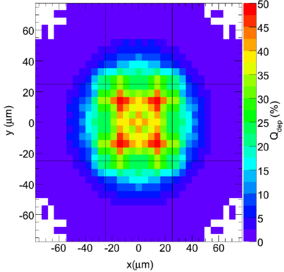
Figure 7.32: A plot showing what percentage the charge deposited by a laser is picked up by the diodes of a test pixel as the laser was moved across a 3 \times 3 pixel grid centered on the test pixel. On this plot the areas defined by 25\mu\text{m} \leq X \leq 25\mu\text{m} and 25\mu\text{m} \leq Y \leq 25\mu\text{m} represent the charge detected when the laser was focused on the test pixel, with X=0\mu\text{m} and Y=0\mu\text{m} corresponding to the charge detected when the laser was focused on the centre of the test pixel. A small percentage ( <10\% ) of charge collected for a given set of X-Y coordinates would indicate that the pixel is relatively insensitive to particles in that region[39].
