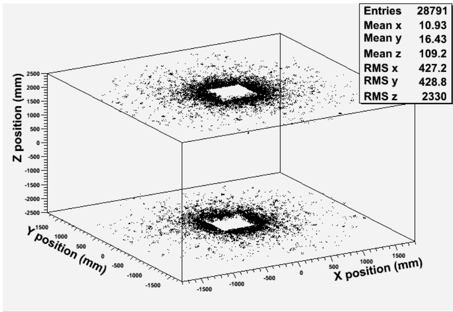
Figure 4.8: A sample histogram showing the positions of all hits in the LDC01 ECAL endcap recorded after a single bunch crossing using the 1TeV High Luminosity parameter set.
