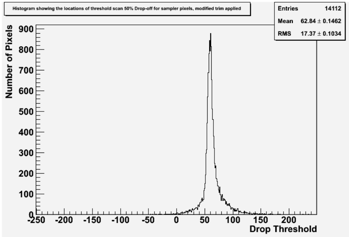
Figure 5.19: A plot showing the distributions of drop-off points of sampler pixels in sensor 16 with the final trims applied to pixels in the sensor. All threshold measurements are in TU.
