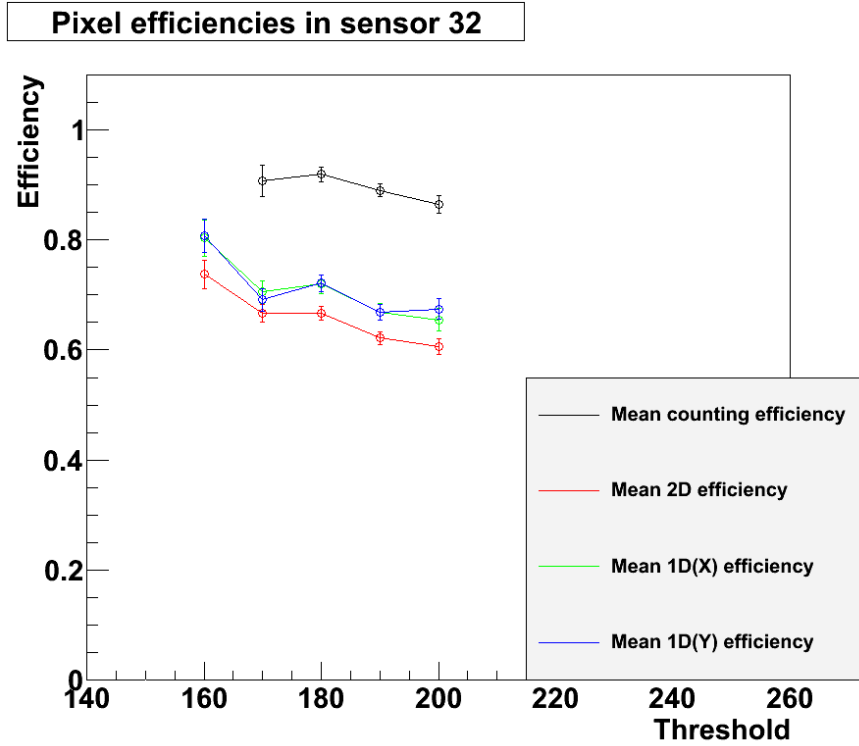
Figure 7.39: Pixel efficiencies in test sensor 32, averaged from several runs in the test beam. The counting method efficiencies were calculated using a three \sigma search range. The efficiency calculated using the counting method has no results at a threshold of 160 because low statistics resulted in several results with efficiencies of either 0 or 1 at this threshold. This was a problem because the binomial error calculated from these values was zero, meaning that these results could not be included in a weighted mean. This combined with the low statistics of the remaining results, made it impractical to include a data point using the counting method at a threshold of 160.
