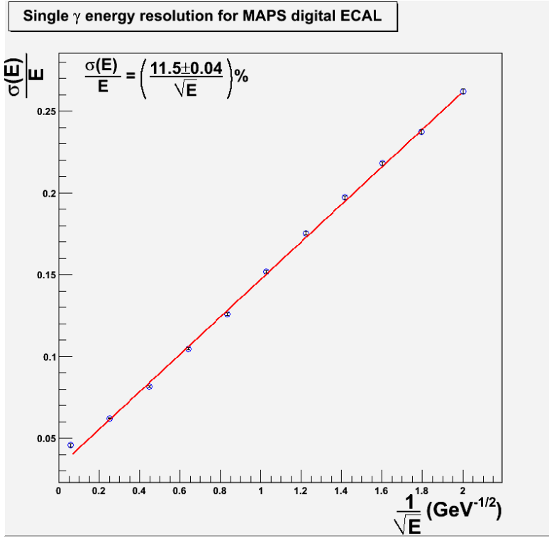
Figure 6.27: A graph showing the simulated variation in energy resolution with particle energy for a MAPS ECAL exposed to single photons within the ILD00 detector.
