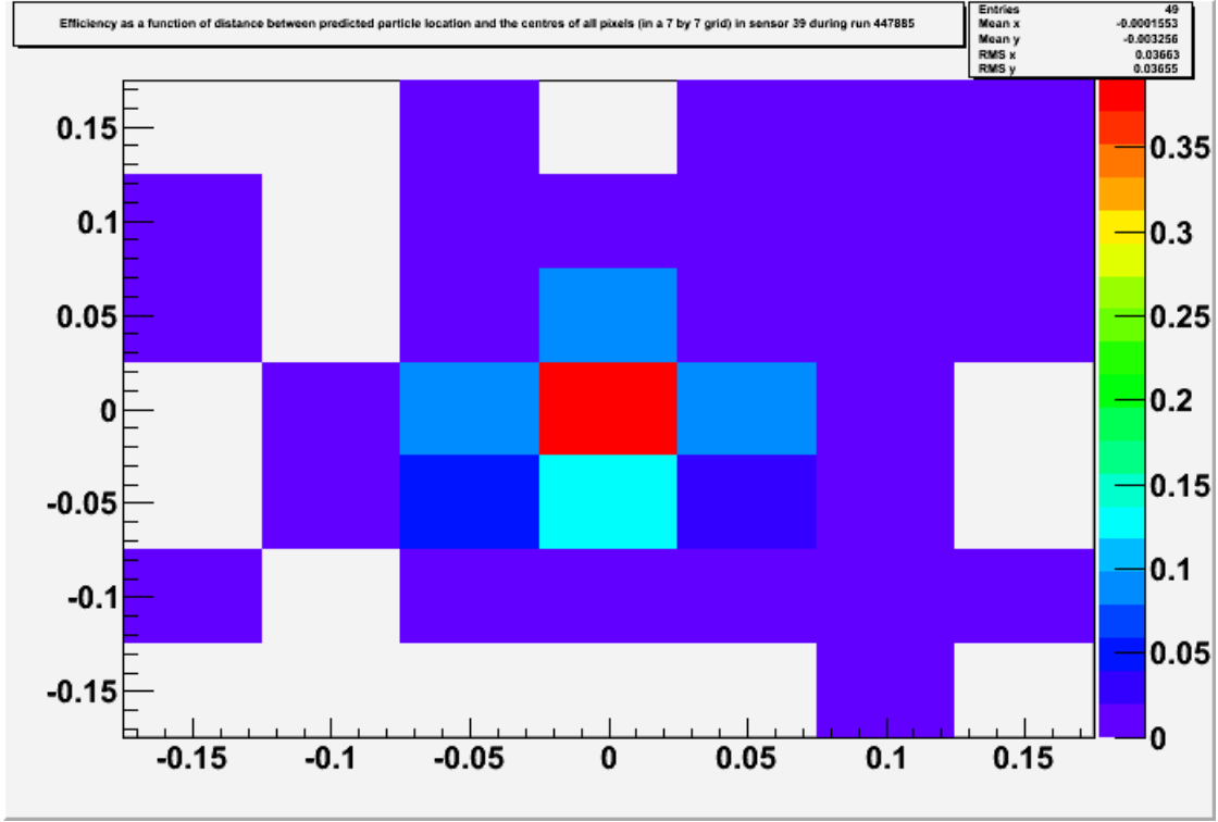
Figure 7.28: An example of the 2D histograms produced to record the variation in apparent pixel efficiency of pixels near to particle tracks in a typical run (447885).
