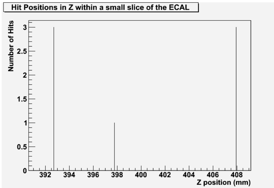
Figure 6.8: A sample histogram showing the transverse distance in the Z direction between hits in a small segment of the analogue ECAL in the extreme positive Y direction, in a single ECAL layer (see figure 6.2 for the region used). The simulations used to produce this histogram used 15.78 GeV photons.
