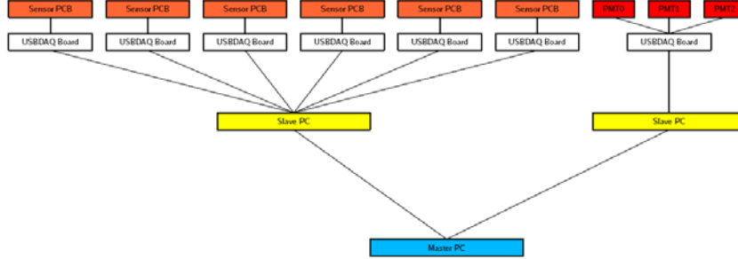
Figure 7.7: Block diagram of the original layout of DAQ apparatus used for the TPAC 1.2 test beam (used from 13/08/2009 to 21/08/2009). The black lines connecting components represent cables carrying data (in various formats) between the components.
