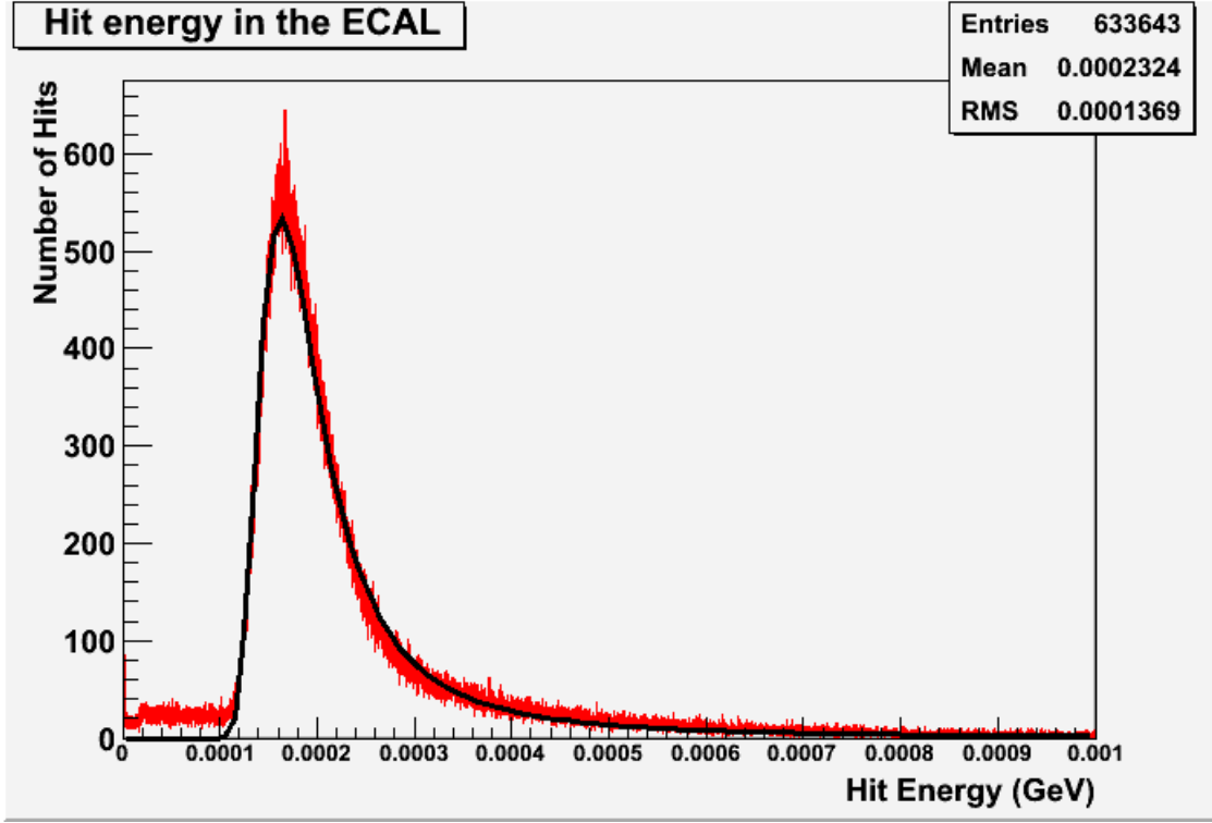
Figure 6.22: A histogram showing the distribution of hit energies recorded in the simulated analogue ECAL when a 10 GeV muon passed through.
