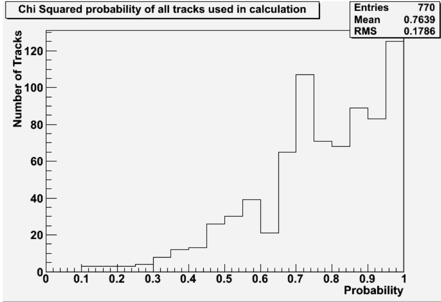
Figure 7.16: An example of the distribution of \chi^2 probabilities of tracks selected for analysis during a run. Notable differences to the unfiltered distribution shown in figure 7.15 include a greater predisposition to high probabilities (due selecting the highest probability in a single bunch train), a complete lack of probabilities below 0.1 (those tracks were discarded), and an overall much smaller number of tracks (due to discarding all but one track when multiple tracks might have been caused by a single particle). This data was recorded during run 447885.
