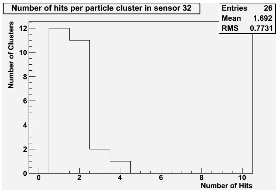
Figure 7.13: An example of the distribution of cluster sizes created by the passage of test particles through sensor 32 during run 447530 (the sensor threshold set during this run was 170TU).
