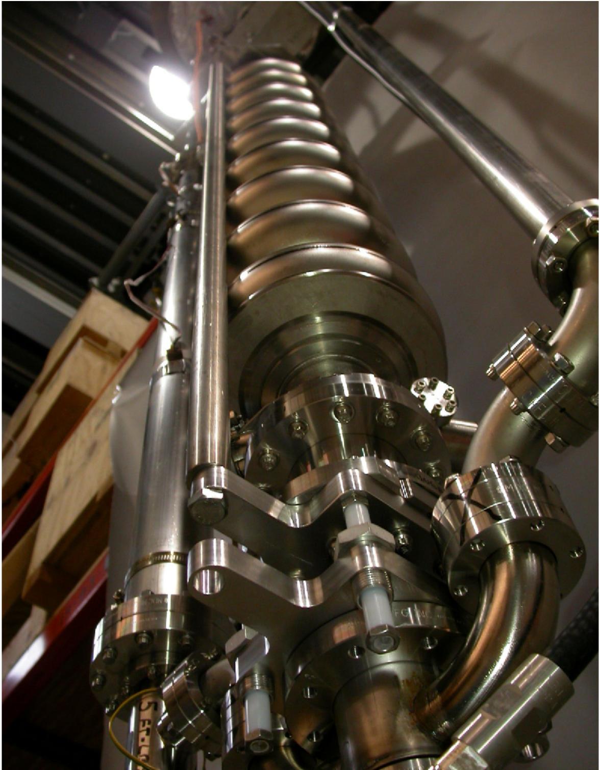
Figure 2.4: ILC SCRF cavity undergoing testing at Cornell[16].
