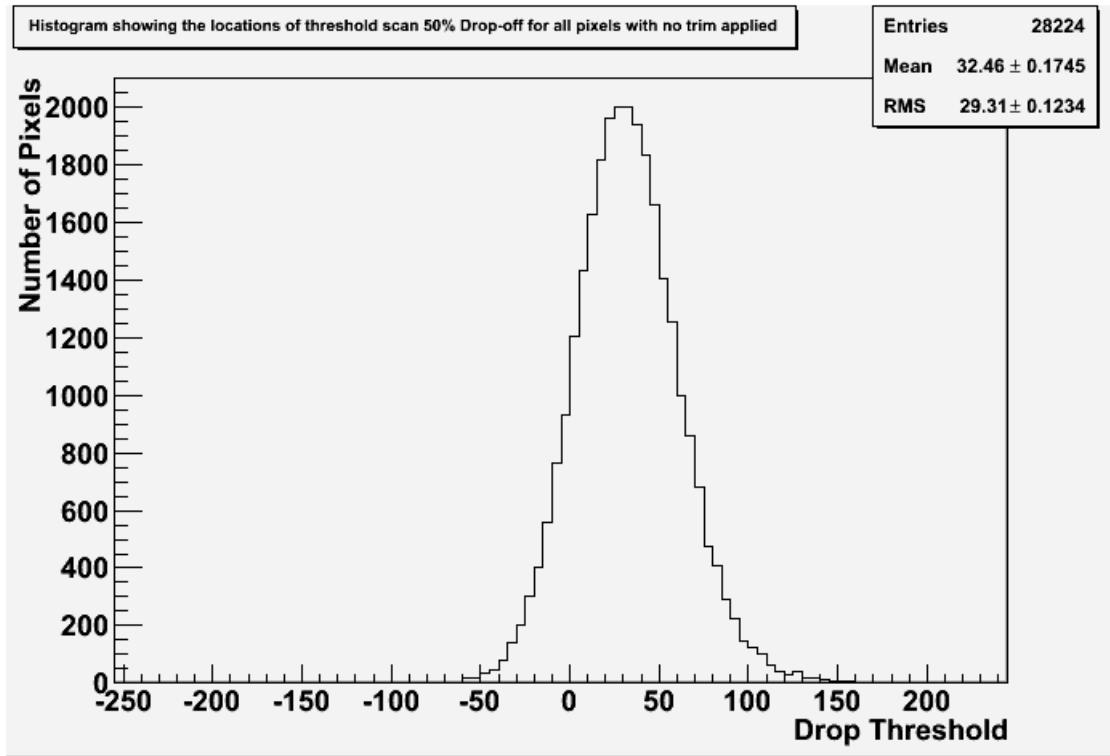
Figure 5.8: A plot showing the distributions of 50% drop-off points of all pixels in sensor 16 with no trim applied. All threshold measurements are in TU.
