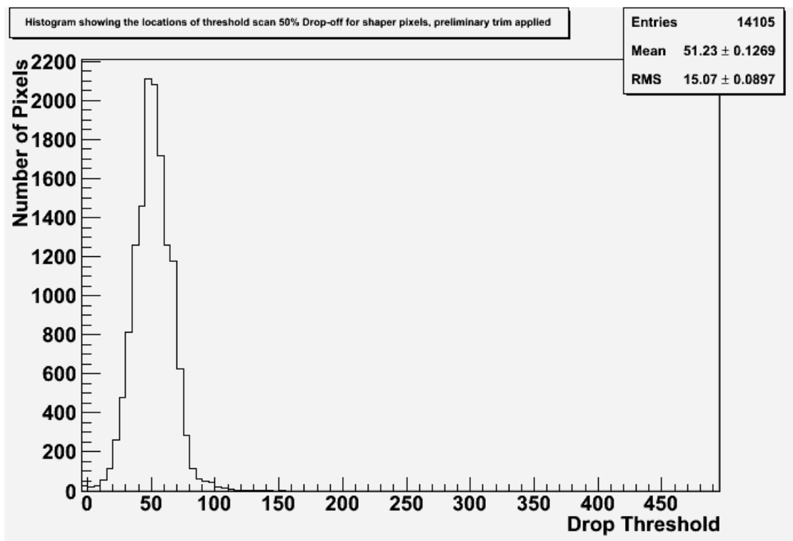
Figure 5.11: A plot showing the distributions of 50% drop-off points of shaper pixels in sensor 16 with a preliminary trim applied to pixels in the sensor. All threshold measurements are in TU.
