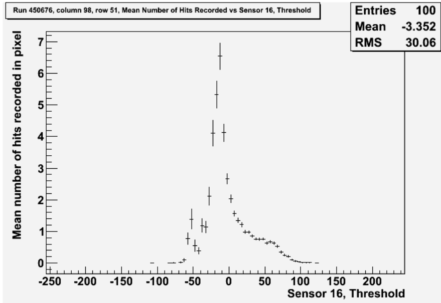
Figure 5.5: A sample threshold scan histogram for an active pixel in the sampler region of the sensor. For every threshold scan run 28224 pixel threshold scan histograms were produced of which 672 were scans of active pixels, and 336 of those active pixels were sampler pixels. In the whole sensor there were 14112 sampler pixels and they commonly displayed the gaussian distribution shown in the threshold scan above. All threshold measurements are in TU.
