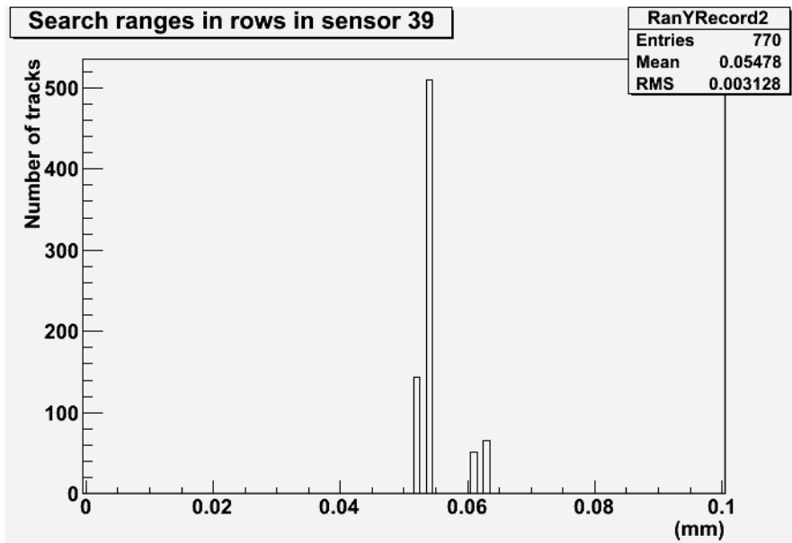
Figure 7.23: An example of two \sigma search ranges for the counting method, in rows, for sensor 39. This data was recorded during run 447885. Note: All search ranges were increased by 25\mu\text{m} to ensure that if the initial search range encompassed any part of a pixel, the search range eventually used would encompass the centre of that pixel (and therefore any hits recorded in that pixel). This histogram shows the final search ranges used
