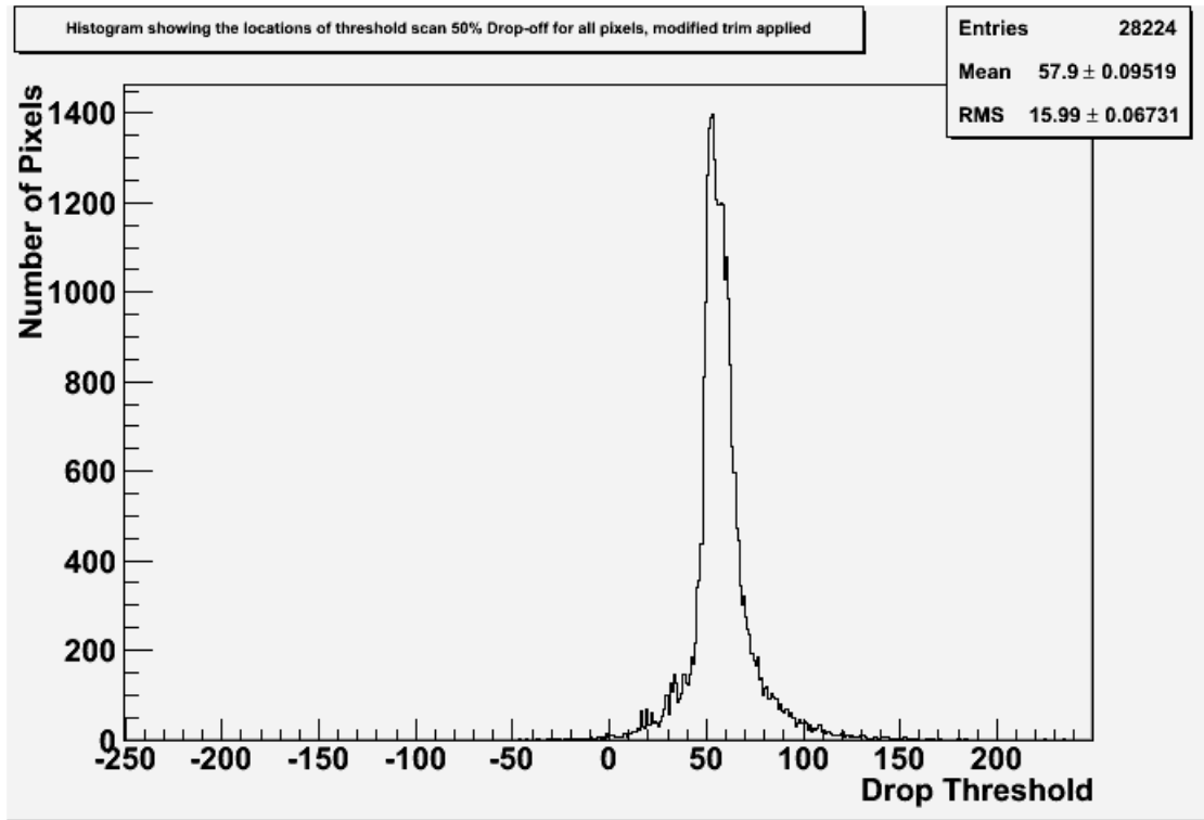
Figure 5.17: A plot showing the distributions of drop-off points of all pixels in sensor 16 with the final trims applied to pixels in the sensor. All threshold measurements are in TU.
