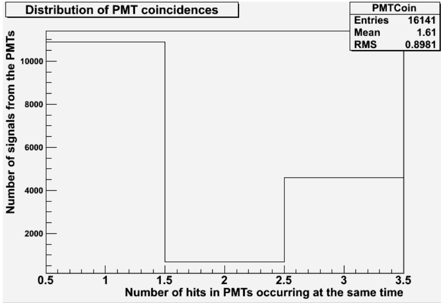
Figure 7.14: An example of the distribution of PMT signal types as recorded by the PMT USBDAQ board. A PMT signal in this case refers to the record of all PMT hits in the same timestamp (the shortest time difference measured by the USBDAQ boards, equal to 400ns), timestamps which did not include any PMT hits were not recorded in this fashion (although hits on the sensors were still recorded normally). This data was recorded during run 447885.
