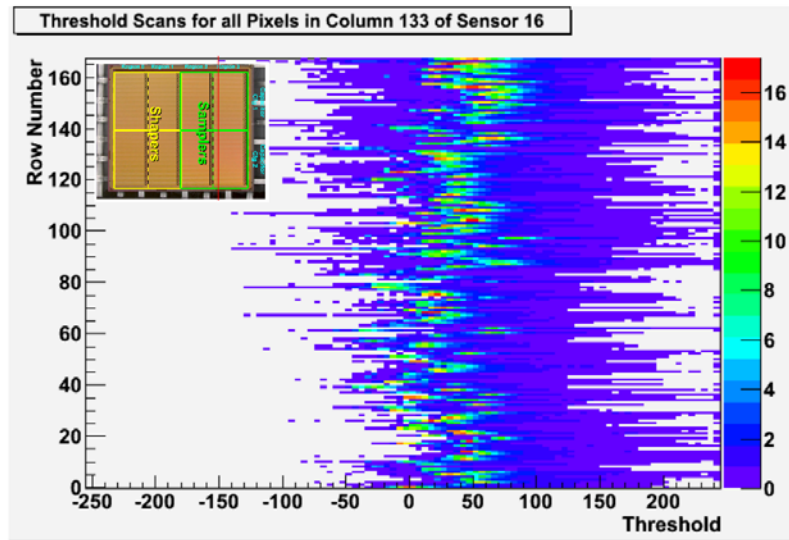
Figure 5.4: A sample 2D histogram showing the threshold scans of all pixels in column 133 of the test sensor when those pixels were active. Since columns 84 to 167 inclusive are composed of sampler pixels, all of the threshold scans in this histogram are from sampler pixels. In order to acquire all the threshold scans depicted, 42 threshold scan runs (with one in every 42 pixels active in each case) were merged together with the inactive pixels in each run being discarded. The small picture in the top left hand corner of the histogram is a picture of the test sensor with the location of column 133 marked by a red line. All threshold measurements are in TU.
