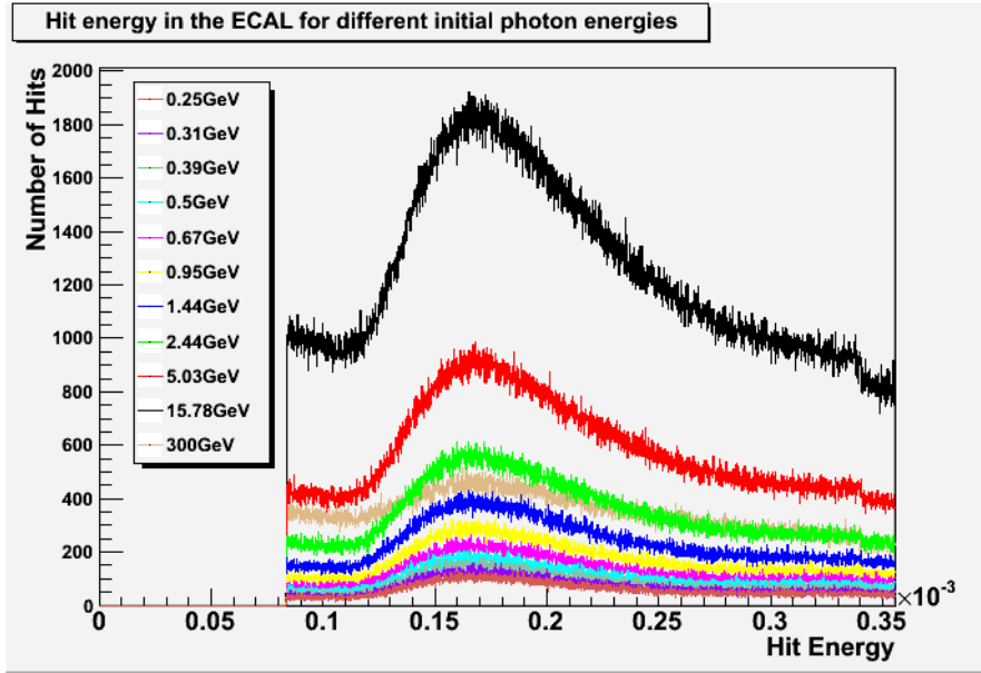
Figure 6.18: A sample histogram showing the distribution of hit energies in the analogue ECAL (i.e. the energy associated with an individual hits) for different initial photon energies. The peak of these distributions changes as the energy of the changes. This is due to an increased probability of multiple particles striking the same pixel leading to one high energy hit where a digital ECAL should measure several lower energy hits. This implies that the 5mm by 5mm pixels used in the analogue ECAL model would not be suitable for use in a digital ECAL.
