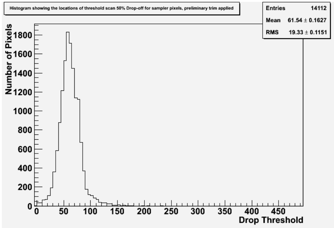
Figure 5.13: A plot showing the distributions of 50% drop-off points of sampler pixels in sensor 16 with a preliminary trim applied to pixels in the sensor. All threshold measurements are in TU.
