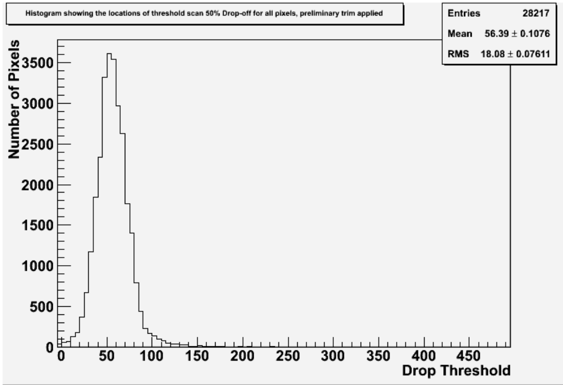
Figure 5.9: A plot showing the distributions of 50% drop-off points of all pixels in sensor 16 with a preliminary trim applied to pixels in the sensor. All threshold measurements are in TU.
