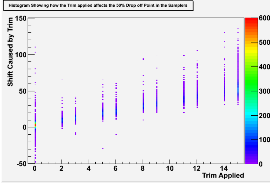
Figure 5.22: A plot showing the shifts in pixel drop off points in sampler pixels in sensor 16 caused by applying different trim settings. This data was collected by comparing run set 450674 to 450715 (untrimmed) to run set 452267 to 452308 (trim based on 50% drop off point, separate targets for shapers and samplers, trim range assumed to be 50 threshold units). All threshold measurements are in TU.
