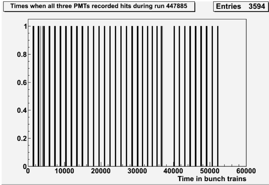
Figure 7.1: A histogram showing the distribution of test beam pulses during a single test run. On this histogram a 1 represents a point in time when all three photo-multiplier tubes attached to the sensor stack recorded simultaneous hits, implying that a beam particle had passed through the sensor stack. Naturally the zeros on this histogram represent times when there were no such hits implying that the test beam was absent. Times are listed in the number of bunch trains (discrete 3.2ms periods when the sensor stack recorded data, see section 7.5 for details) since the run started. The approximately 50000 bunch trains during run 477885 were evenly spread out over a period of 1800 seconds.
