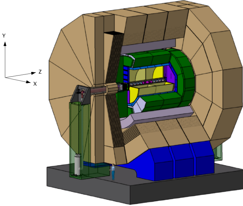
Figure 6.1: A diagram showing the overall layout of the ILD detector as well as the coordinates system used throughout this chapter. The zero point of all coordinate in this system is the interaction point at the centre of the detector.
