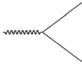
Bethe-Heitler Process
