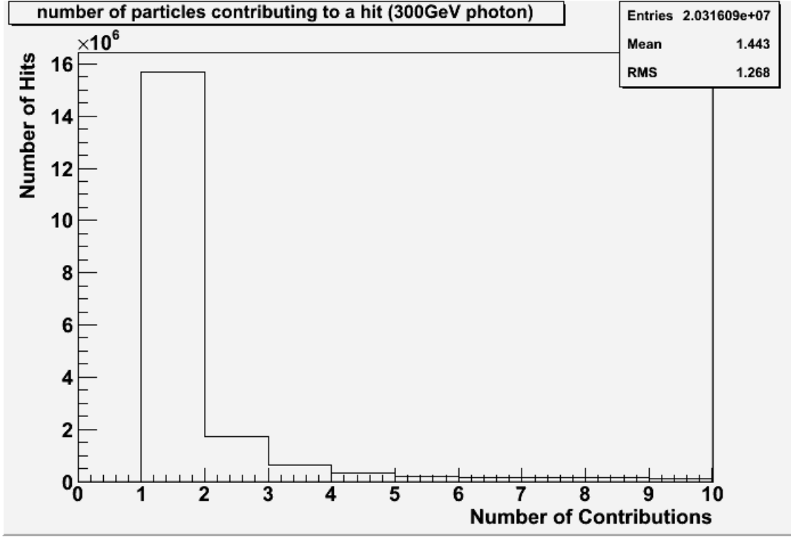
Figure 6.20: A sample histogram showing distribution of the number of particles contributing to each hit in a MAPS ECAL exposed to a 300 GeV photon.
