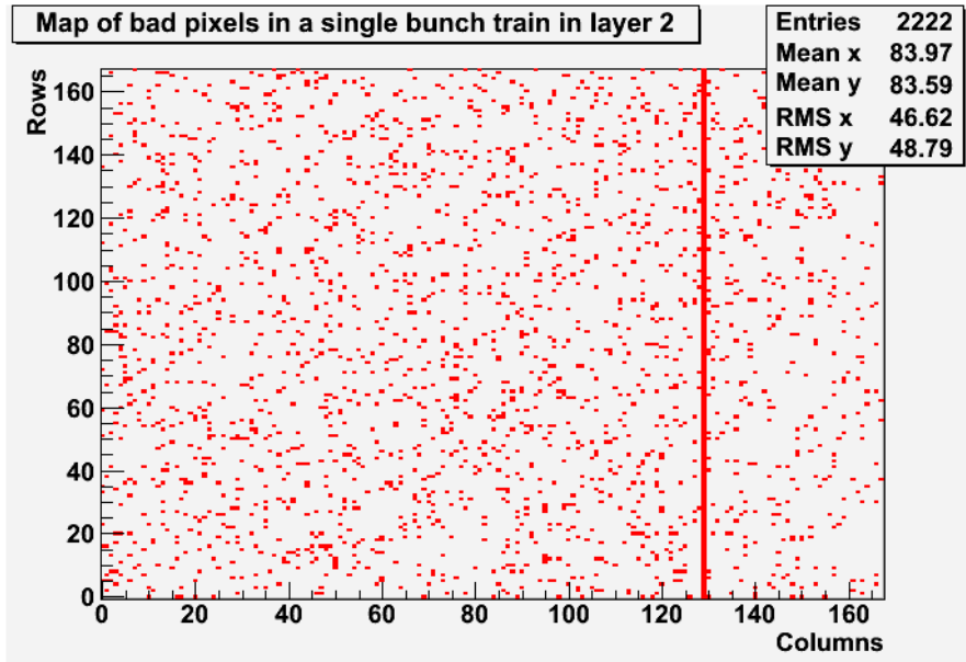
Figure 7.11: A map of the bad pixels on sensor 39. The red regions represent defective pixels while the white regions represent functioning pixels. The axes labels represent the column and row numbers of the pixels. This map was recorded during a single bunch train in run 447885. In this case the bad pixels represent approximately 8% of all the pixels on the sensor.
