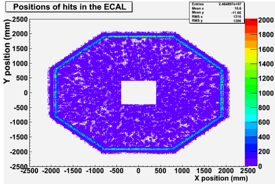
Figure 6.12: A sample hit map showing the distribution of all hits recorded in a simulated MAPS (digital) ECAL during 20000 simulated 15.78 GeV photon events. This diagram shows the ECAL as it would be seen from further along the beam line (i.e. the beam is perpendicular to the page), X and Y are arbitrary directions perpendicular to the beam line and perpendicular to each other. The distribution of hits implies that the particle showers simulated were contained within the ECAL.
