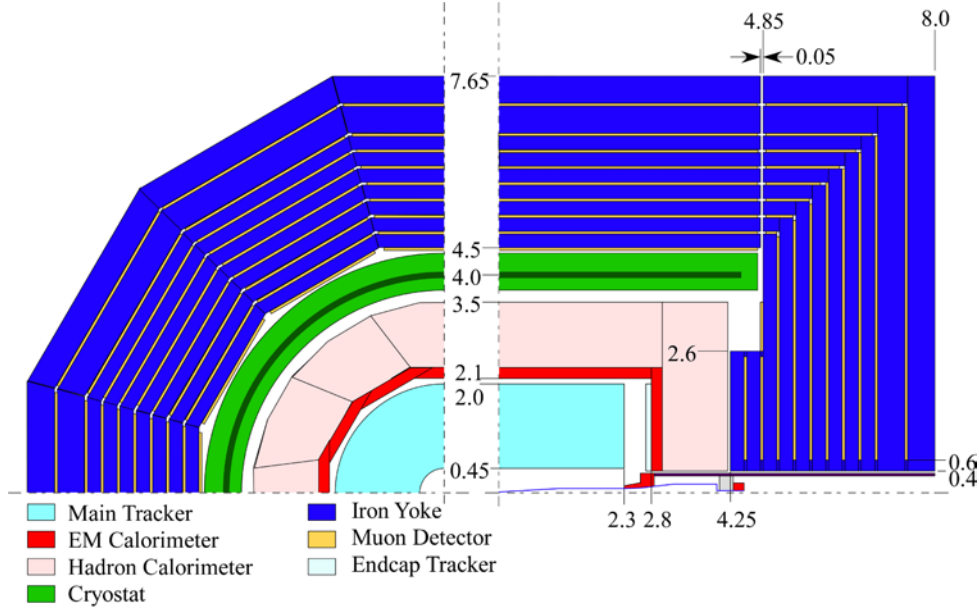
Figure 2.6: Diagram of the GLD detector[24]
