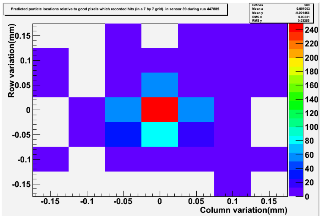
Figure 7.27: An example of the 2D histograms produced to record particle track positions relative to the centres of nearby pixels which recorded hits in a typical run (447885).
