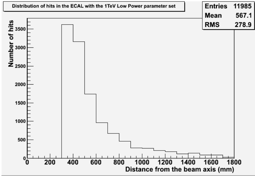
Figure 4.6: A sample histogram showing the distribution of hits in the LDC01 ECAL endcap relative to the beam axis recorded after a single bunch crossing using the 1TeV Low Power parameter set.
