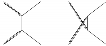
Landau-Lifshitz Process
