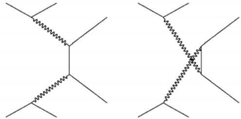
Landau-Lifshitz Process
