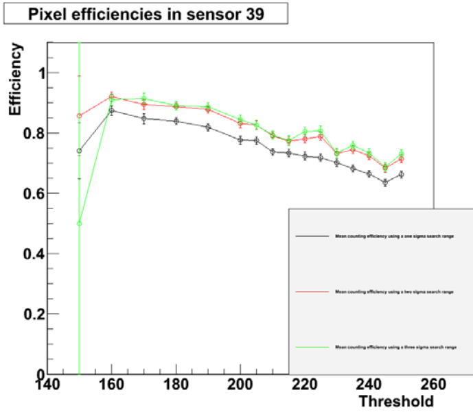
Figure 7.36: Counting method pixel efficiencies in test sensor 39, averaged from several runs in the test beam, using a range of different search areas.
