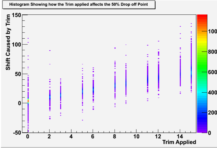
Figure 5.20: A plot showing the shifts in pixel drop off points in sensor 16 caused by applying different trim settings. This data was collected by comparing run set 450674 to 450715 (untrimmed) to run set 452267 to 452308 (trim based on 50% drop off point, separate targets for shapers and samplers, trim range assumed to be 50 threshold units). Equivalent histograms showing only results from either shaper or sampler pixels are shown in figures 5.21 and 5.22 respectively. All threshold measurements are in TU.
