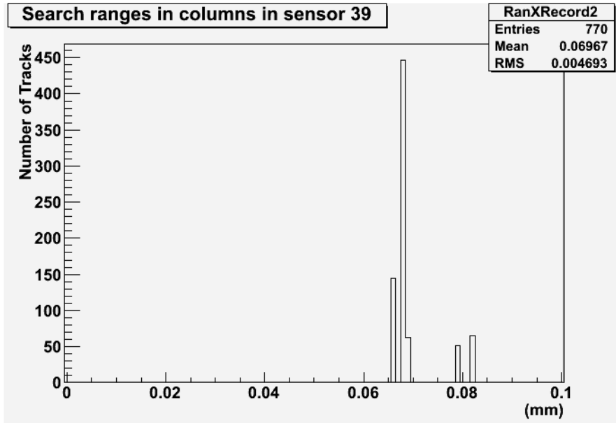
Figure 7.24: An example of three \sigma search ranges for the counting method, in columns, for sensor 39. This data was recorded during run 447885. Note: All search ranges were increased by 25\mu\text{m} to ensure that if the initial search range encompassed any part of a pixel, the search range eventually used would encompass the centre of that pixel (and therefore any hits recorded in that pixel). This histogram shows the final search ranges used
