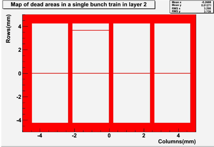
Figure 7.10: A map of the dead areas in and near sensor 39 during a single 3.2ms period (referred to as a bunch train). The red regions represent either areas which contain no pixels, or where the pixels were saturated during the bunch train in question, white regions represent functioning pixels. This map was recorded during a single bunch train in run 447885.
