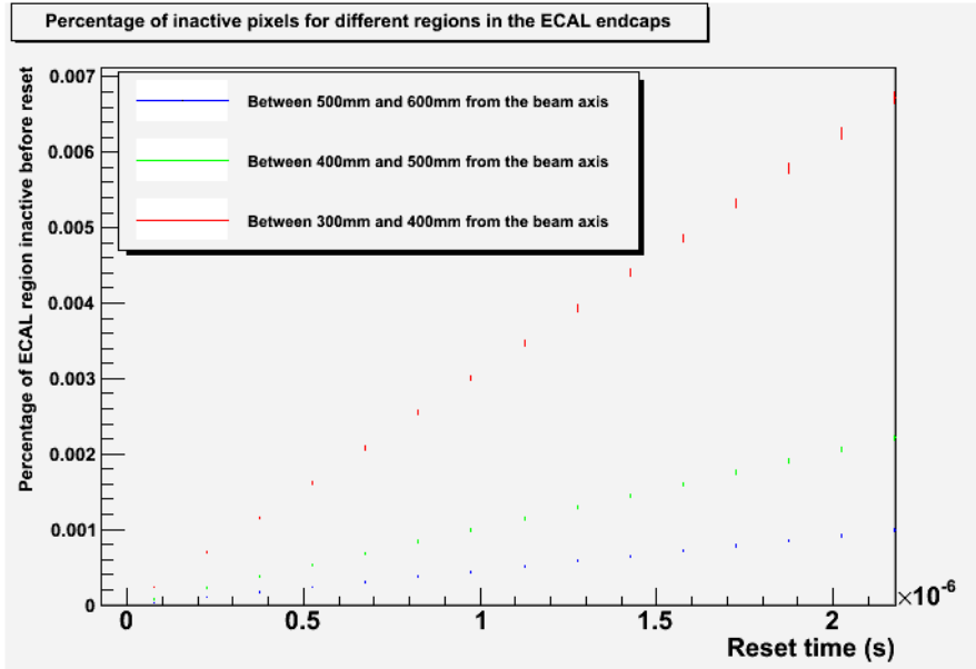
Figure 4.11: Variation in percentage of pixels inactive in ECAL endcap with reset time and location relative to the beam. The maximum reset/readout interval shown is 2000ns, approximately equal to the pixel reset times under consideration for a MAPS during this study.
