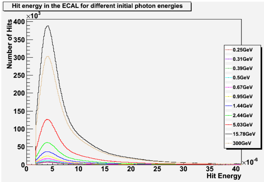
Figure 6.17: A sample histogram showing the distribution of hit energies in GeV in the MAPS ECAL (i.e. the energy associated with an individual hit) for different initial photon energies.
