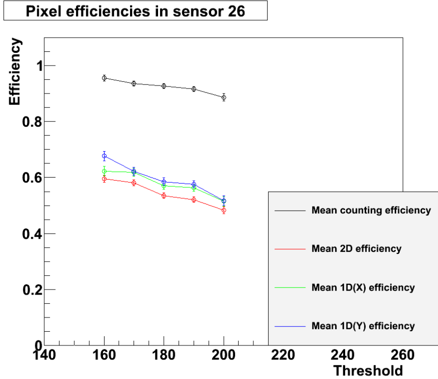
Figure 7.38: Pixel efficiencies in test sensor 26, averaged from several runs in the test beam. The counting method efficiencies were calculated using a three \sigma search range.
