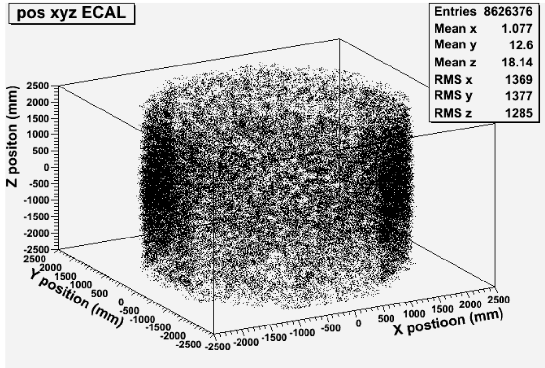
Figure 6.6: A sample 3D histogram showing the locations of all hits in an analogue ECAL. The simulation used to produce this histogram used 15.78 GeV photons.
