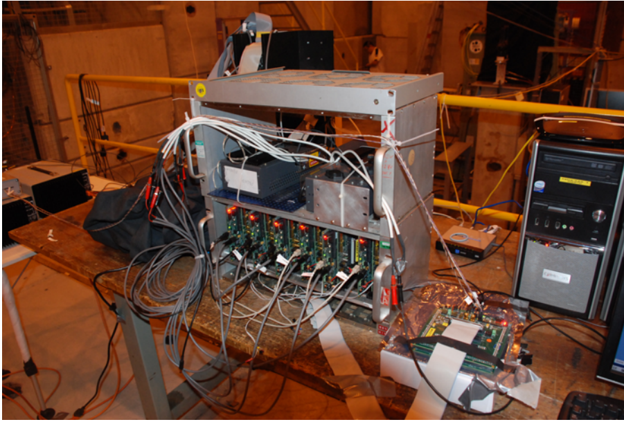
Figure 7.9: A picture of the DAQ crate containing six USBDAQ boards with the seventh board lying next to the crate in the foreground. The two cables attached at the front of each of the crated USBDAQ board are the data cables connecting the USBDAQ boards to one of the slave PCs (this is the USB cable), and a power lead connecting the USBDAQ boards to the power supplies on the upper level of the DAQ crate. The TPAC 1.2 test stand is visible at the back of the picture and the sensor PCBs and PMTs are connected to their respective USBDAQ boards via ribbon cables (the connection between the cables and the USBDAQ boards is obscured by the USBDAQ boards themselves and the DAQ crate).
