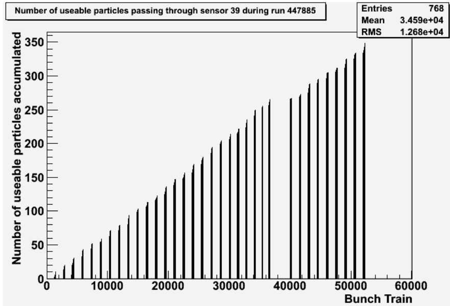
Figure 7.17: An example of how useable particles passing through a sensor are accumulated in a typical run. In this case useable are particles detected by all three PMTs and not having any dead areas or bad pixels in their projected search area)
