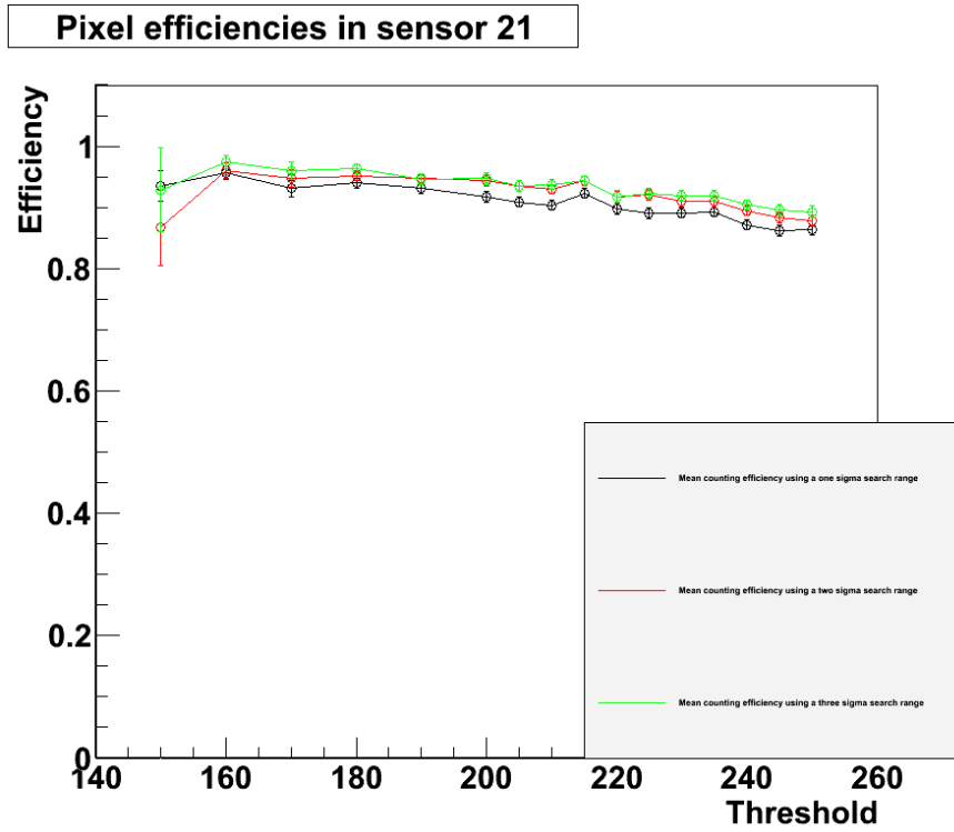
Figure 7.33: Counting method pixel efficiencies in test sensor 21, averaged from several runs in the test beam, using a range of different search areas.
