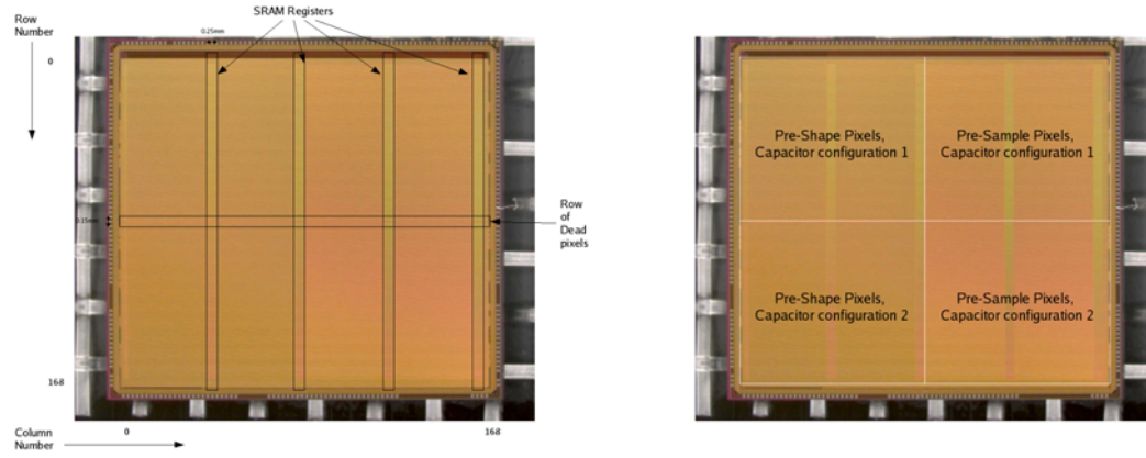
Figure 3.6: A picture of a TPAC 1.0 sensor showing the dead areas present in the sensitive region(left), and the relative positions of different pixel types(right)[32].
