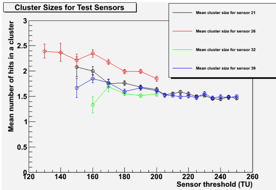
Figure 7.12: A graph showing how the sensor threshold set affected the mean number of hits found clustered together when test particles passed through the sensors. Sensor thresholds where there were insufficient statistics to estimate errors in the mean number of hits per cluster (i.e. where less than two clusters were detected for all results analysed) were omitted from this graph. The plots for sensors 26 and 32 were based on results from runs 447526-447533, 447596-447603, 447667-447674, and 447683-447690. The plots for sensors 21 and 39 were based on results from runs 447783-447790, 447820-447827, 447883-447892, 447903-447912, and 447951-447960. An example of the distribution of cluster sizes during a single run is shown in figure 7.13.
