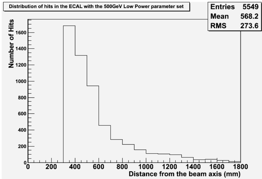
Figure 4.7: A sample histogram showing the distribution of hits in the LDC01 ECAL endcap relative to the beam axis recorded after a single bunch crossing using the 500 GeV Low Power parameter set.
