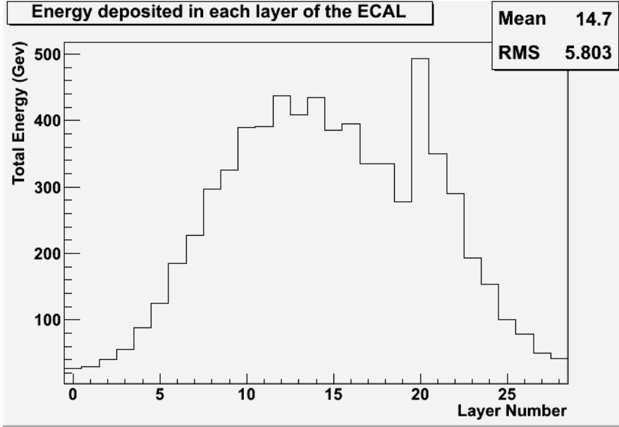
Figure 6.16: A sample histogram showing the distribution of energies deposited in different layers of the analogue ECAL during 1000 simulated events using a 300 GeV photon. The relatively small energy deposited in the outer layers of the ECAL implies that the photon shower was typically well contained within the ECAL at this energy (300 GeV was the highest particle energy used for this study). The energy deposited on the outermost 10 layers of the ECAL was doubled to represent the increased thickness of the absorber layers paired with these sensitive layers. This causes the energy recorded to increase at layer 20. Note: this histogram records the combined energies deposited on the ECAL during the entire simulation run, not the energies of individual events.
