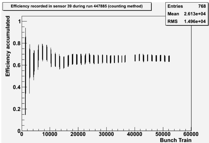
Figure 7.19: An example of how efficiency for a sensor is produced (using the counting method) during a typical run.
