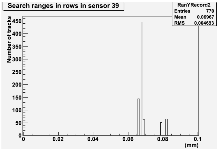
Figure 7.25: An example of three \sigma search ranges for the counting method, in rows, for sensor 39. This data was recorded during run 447885. Note: All search ranges were increased by 25\mu\text{m} to ensure that if the initial search range encompassed any part of a pixel, the search range eventually used would encompass the centre of that pixel (and therefore any hits recorded in that pixel). This histogram shows the final search ranges used.
