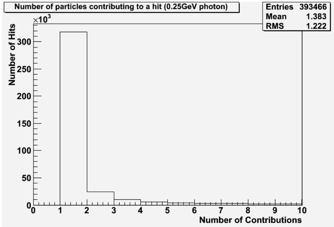
Figure 6.19: A sample histogram showing distribution of the number of particles contributing to each hit in a MAPS ECAL exposed to a 0.25 GeV photon.
