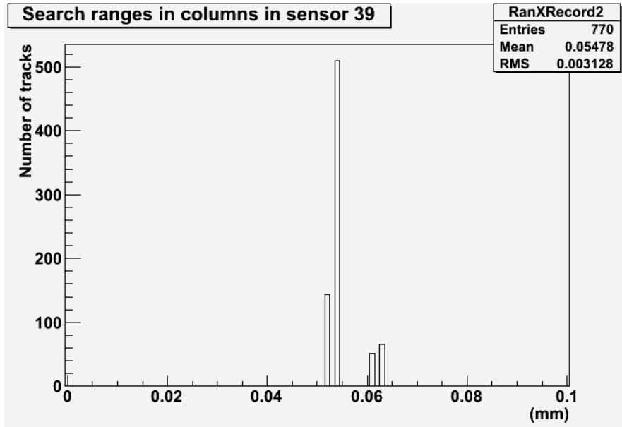
Figure 7.22: An example of two \sigma search ranges for the counting method, in columns, for sensor 39. This data was recorded during run 447885. Note: All search ranges were increased by 25\mu\text{m} to ensure that if the initial search range encompassed any part of a pixel, the search range eventually used would encompass the centre of that pixel (and therefore any hits recorded in that pixel). This histogram shows the final search ranges used
