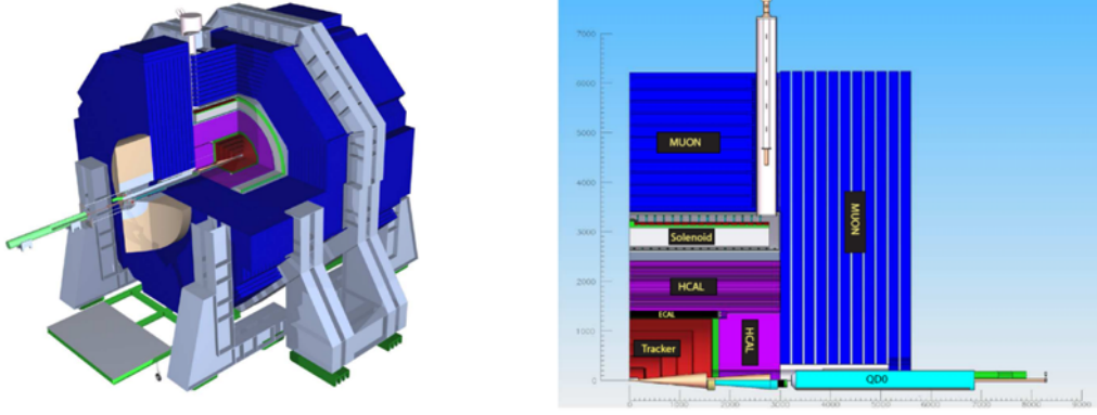
Figure 2.8: 3D diagram of the SiD concept (left), and a \frac{1}{4} diagram showing the structure of the SiD concept(right). Note: on this diagram the iron return yoke of the solenoid has been labelled as the muon system because the muon system uses the return yoke for its absorber layers, meaning both systems occupy the same space.[25]
