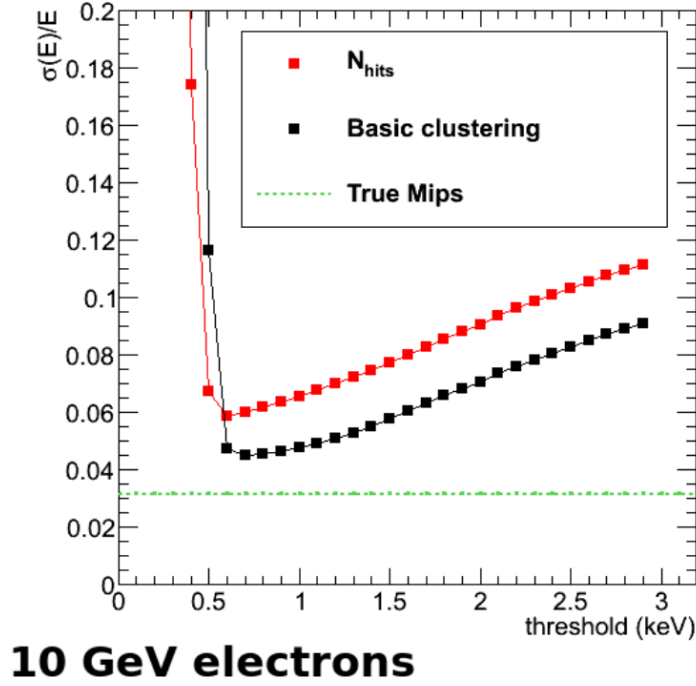
Figure 3.3: Predicted variations in ECAL energy resolution with varying sensor threshold based on simulations. The line labelled N_{hits} represents the energy resolution based on simply counting the number of hits found within the sensor for an energy measurement while the line labelled Basic Clustering counted only hits found within clusters. Similarly the line labelled “True MIPs” represents the energy resolution based on counting the number of MIPs simulated[39][29].
