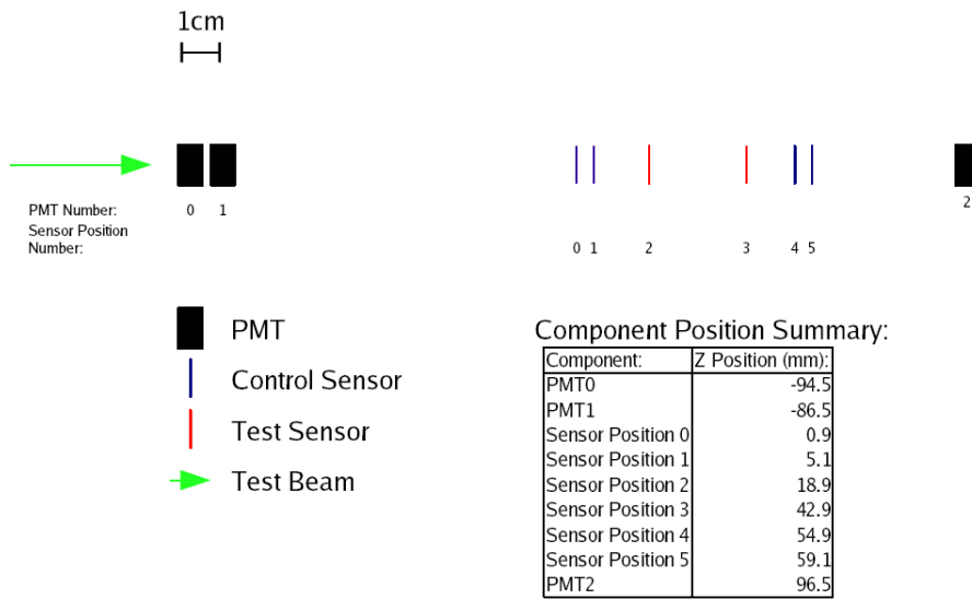
Figure 7.6: Layout of sensitive regions (both sensors and PMTs) within a completed sensor stack. Z position for each component is the distance (along the beam line) between the base plate of the sensor stack and the centre of the sensitive region of the component in question.
