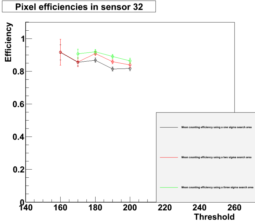
Figure 7.35: Counting method pixel efficiencies in test sensor 32, averaged from several runs in the test beam, using a range of different search areas. The efficiency calculated using the three \sigma search area has no results at a threshold of 160 because low statistics resulted in several results with efficiencies of either 0 or 1 at this threshold. This was a problem because the binomial error calculated from these values was zero, meaning that these results could not be included in a weighted mean. This combined with the low statistics of the remaining results, made it impractical to include a data point using the three \sigma search area at a threshold of 160.
