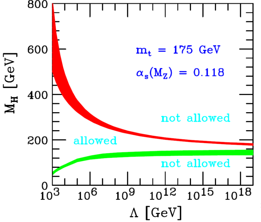
Figure 1.1: Theoretical range of the Higgs mass assuming the Standard Model remains valid up to cut-off scale \Lambda [8].
