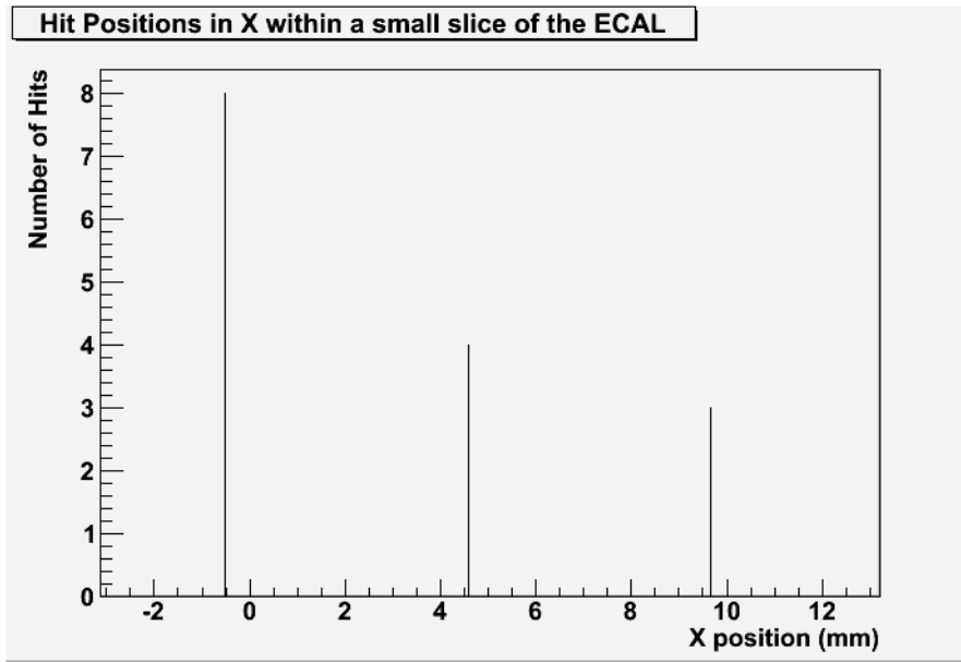
Figure 6.7: A sample histogram showing the transverse distance in the X direction between hits in a small segment of the analogue ECAL in the extreme positive Y direction, in a single ECAL layer (see figure 6.2 for the region used). The simulations used to produce this histogram used 15.78 GeV photons.
