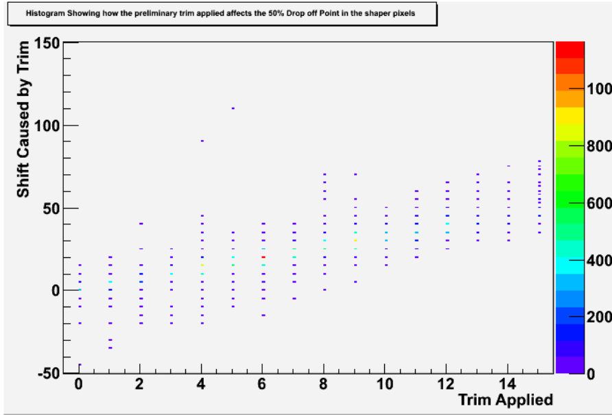
Figure 5.15: A plot showing the shifts in pixel 50% drop off points in shaper pixels in sensor 16 caused by applying different trim settings. This data was collected by comparing run set 450674 to 450715 (untrimmed) to run set 452056 to 452097 (trim based on 50% drop off point, separate targets for shapers and samplers, trim range assumed to be 100TU). All threshold measurements are in TU.
