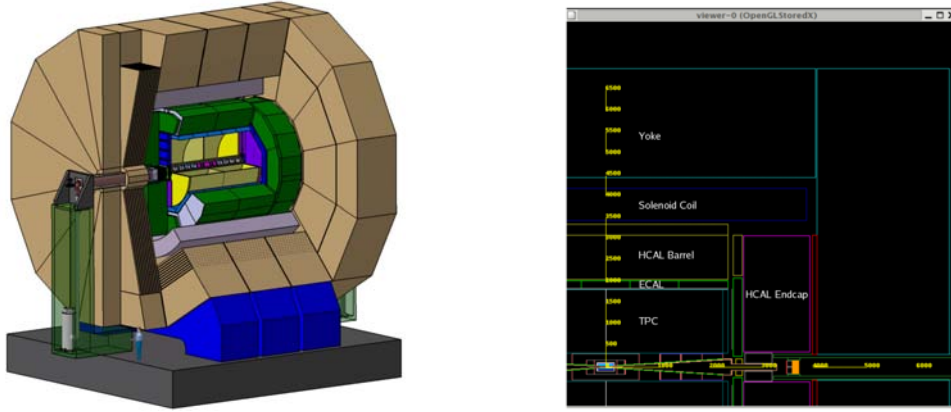
Figure 2.5: The overall intended structure of the ILD(left)[17] and a \frac{1}{4} diagram showing the relative locations of major components(right)[23].
