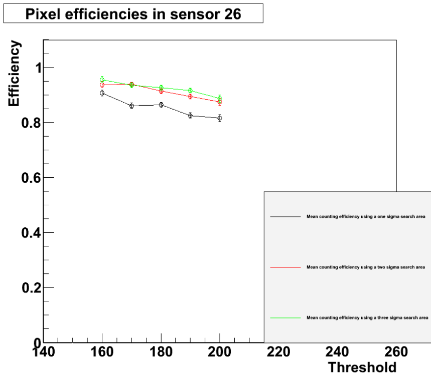
Figure 7.34: Counting method pixel efficiencies in test sensor 26, averaged from several runs in the test beam, using a range of different search areas.
