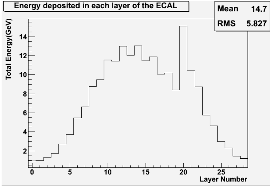
Figure 6.14: A sample histogram showing the distribution of energies deposited in different layers of the MAPS ECAL during 20000 simulated events using a 300 GeV photon. The relatively small energy deposited in the outer layers of the ECAL implies that the photon shower was typically well contained with the ECAL at this energy (300 GeV was the highest particle energy used for this study). The energy deposited on the outermost 10 layers of the ECAL was doubled to represent the increased thickness of the absorber layers paired with these sensitive layers. This causes the energy recorded to increase at layer 20. Note: this histogram records the combined energies deposited on the ECAL during the entire simulation run, not the energies of individual events.
