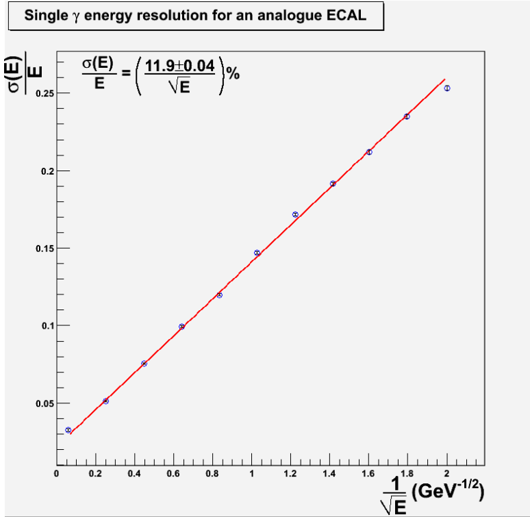
Figure 6.28: A graph showing the simulated variation in energy resolution with particle energy for an analogue ECAL exposed to single photons within the ILD00 detector.
