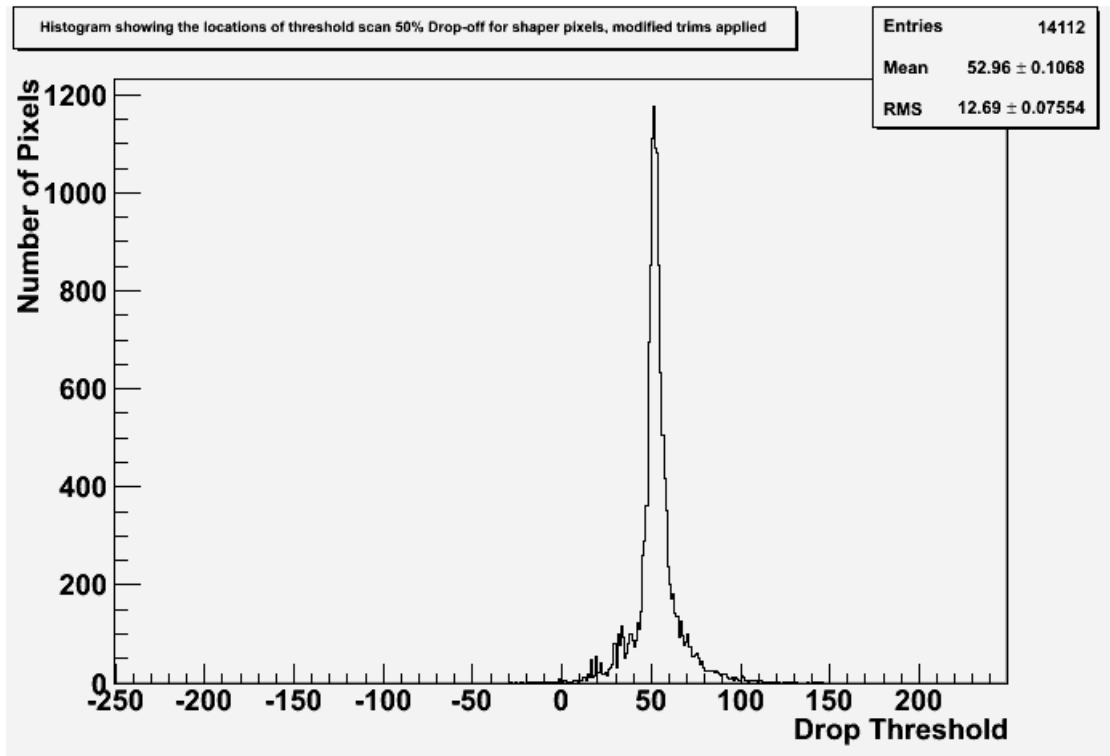
Figure 5.18: A plot showing the distributions of drop-off points of shaper pixels in sensor 16 with the final trims applied to pixels in the sensor. All threshold measurements are in TU.
