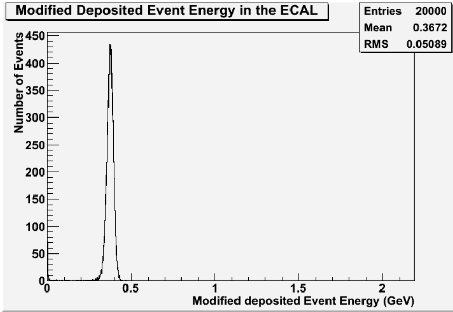
Figure 6.24: A sample histogram showing the distribution of the energy deposited in the sensitive silicon of a simulated analogue ECAL in single events. These energies have been modified so that the energies of hits recorded in the outer ECAL are doubled. Each event in this distribution corresponds to a 15.78 GeV photon passing through the ECAL.
