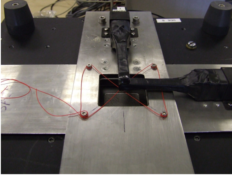
Figure 7.4: A pair of PMTs attached to the underside of the test stand used for the TPAC 1.2 test beam. Due to the alignment of the sensor stack in the test beam, these two PMTs were the first sensor stack component in the path of test beam particles.
