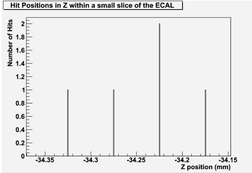
Figure 6.5: A sample histogram showing the transverse distance in the Z direction (along the beam line) between hits in a small segment of the MAPS ECAL in the extreme positive Y direction, in a single ECAL layer (see figure 6.2 for the region used). The simulations used to produce this histogram used 15.78 GeV photons.
