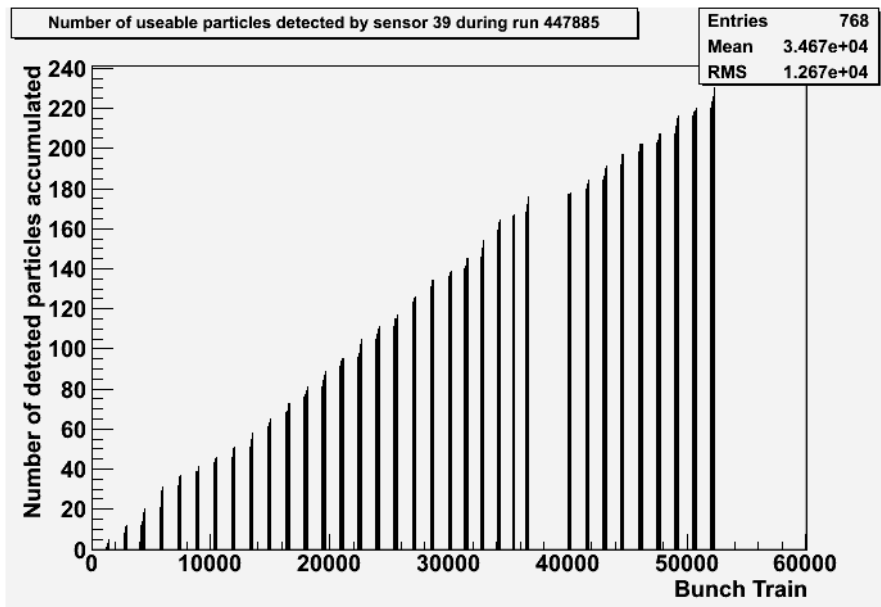
Figure 7.18: An example of how useable particles detected by a particular sensor are accumulated in a typical run. In this case useable particles are particles detected by all three PMTs and not having any dead areas or bad pixels in their projected search area.
