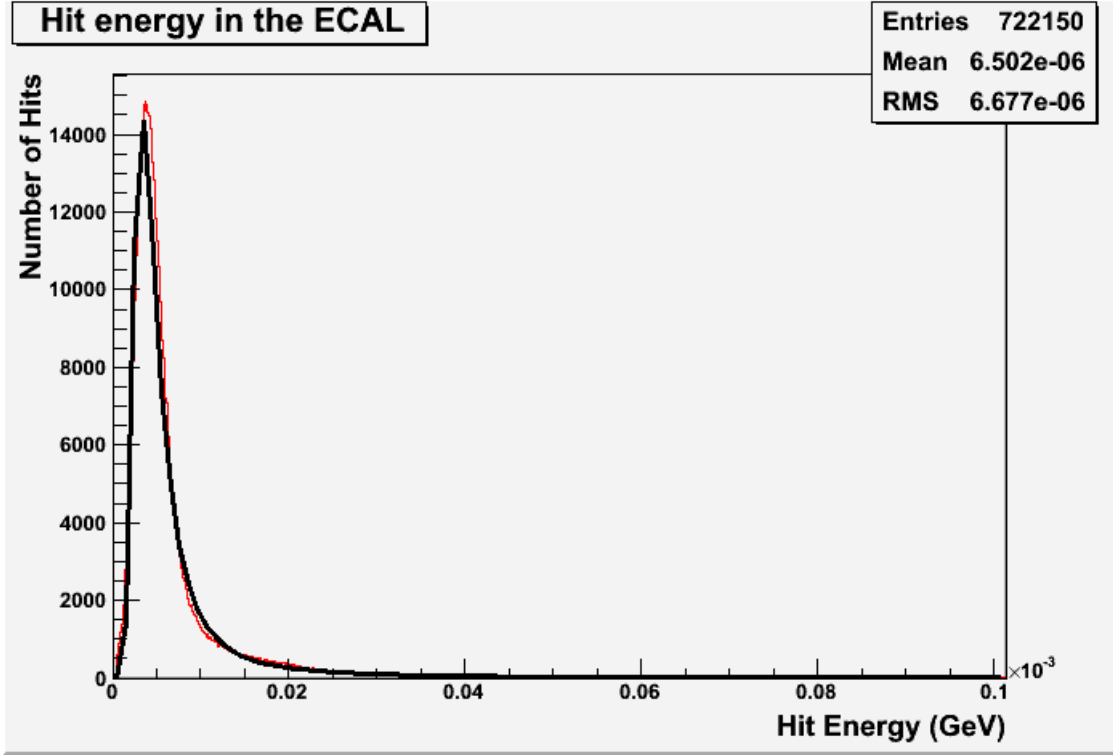
Figure 6.21: A histogram showing the distribution of hit energies recorded in the simulated MAPS ECAL when a 10 GeV muon passed through.
