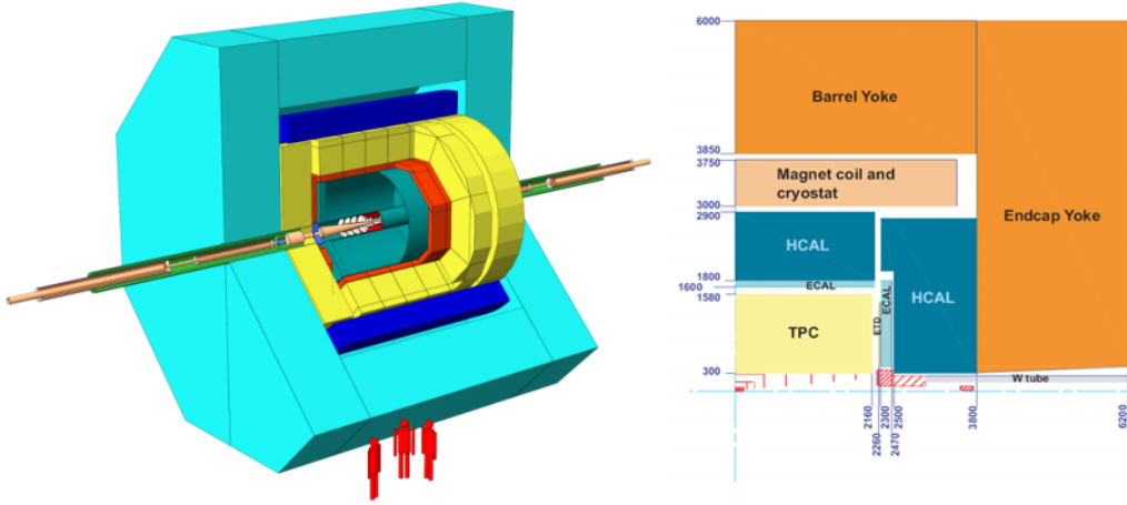
Figure 2.7: 3D diagram of the Large Detector Concept(LDC)(left) and a \frac{1}{4} diagram showing the relative locations of components[15].
