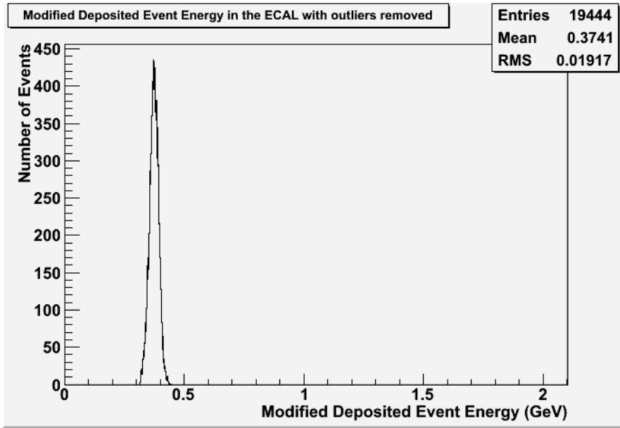
Figure 6.26: A sample histogram showing the distribution of the energy deposited in the sensitive silicon of a simulated analogue ECAL in single events. These energies have been modified so that the energies of hits recorded in the outer ECAL are doubled. Additionally the distribution of deposited energies shown in this histogram has been modified to exclude all events where the energy deposited was more than the (unaltered) mean plus two (unaltered) standard deviations or less than the (unaltered) mean minus one (unaltered) standard deviation. The unmodified distribution used to produce this histogram is shown in figure 6.24. Each event in this distribution corresponds to a 15.78 GeV photon passing through the ECAL.
