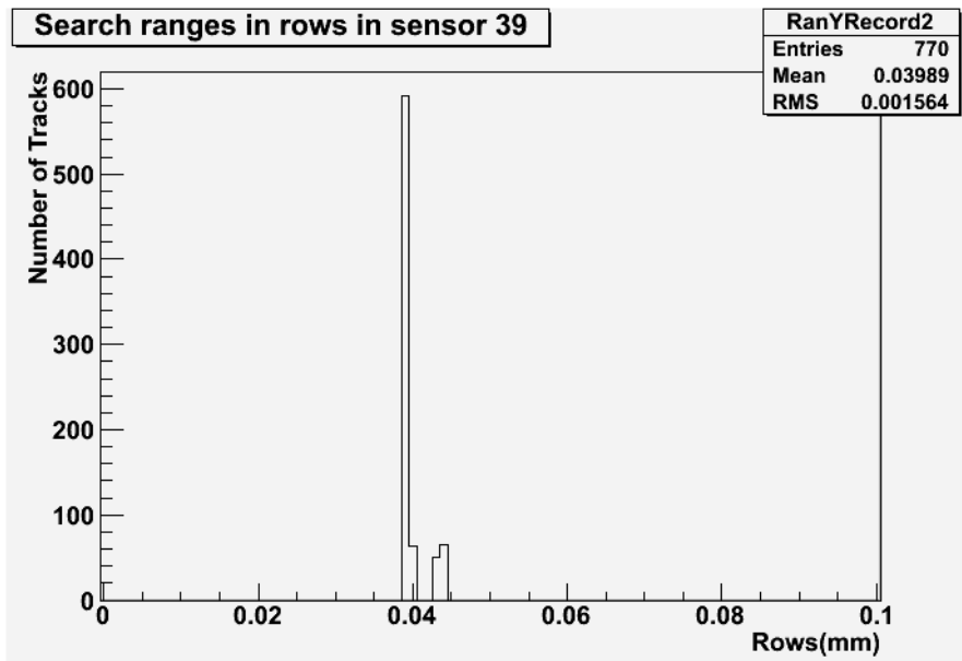
Figure 7.21: An example of one \sigma search ranges for the counting method, in rows, for sensor 39. This data was recorded during run 447885. Note: All search ranges were increased by 25\mu\text{m} to ensure that if the initial search range encompassed any part of a pixel, the search range eventually used would encompass the centre of that pixel (and therefore any hits recorded in that pixel). This histogram shows the final search ranges used.
