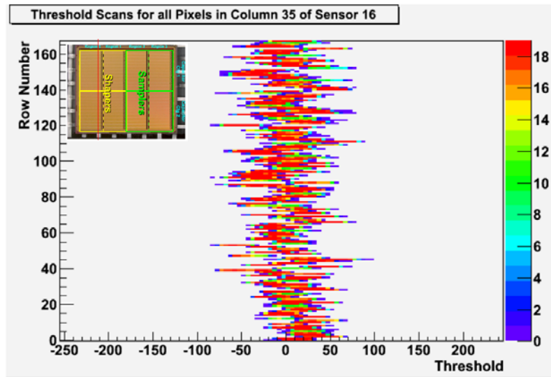
Figure 5.3: A sample 2D histogram showing the profiles of the threshold scan histograms of all pixels in column 35 of the test sensor when those pixels were active. Since columns 0 to 83 inclusive are composed of shaper pixels, all of the threshold scans in this histogram are from shaper pixels. In order to acquire all the threshold scans depicted, 42 threshold scan runs (with one in every 42 pixels active in each case) were merged together with the inactive pixels in each run being discarded. The small picture in the top left hand corner of the histogram is a picture of the test sensor with the location of column 35 marked by a red line. All threshold measurements are in TU.
