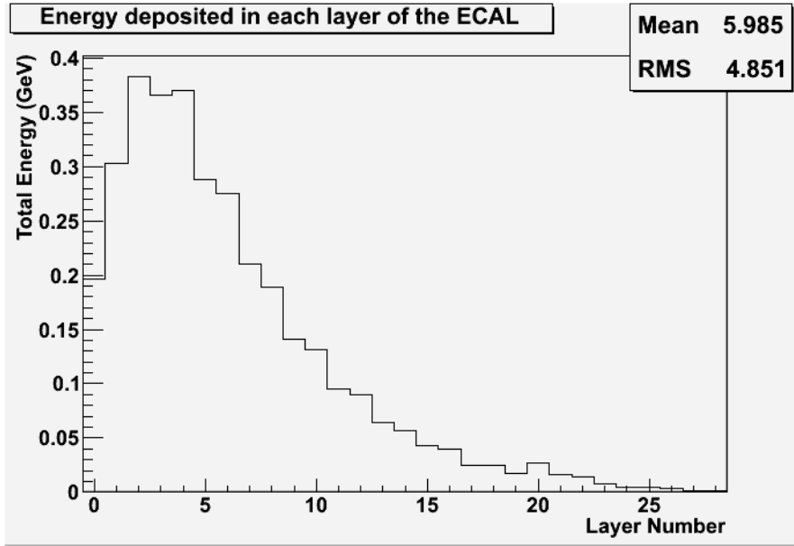
Figure 6.13: A sample histogram showing the distribution of energies deposited in different layers of the MAPS ECAL during 20000 simulated events using a 0.25 GeV photon. The relatively small energy deposited in the outer layers of the ECAL implies that the photon shower was typically well contained with the ECAL at this energy (0.25 GeV was the lowest particle energy used for this study). The energy deposited on the outermost 10 layers of the ECAL was doubled to represent the increased thickness of the absorber layers paired with these sensitive layers. This causes the energy recorded to increase at layer 20. Note: this histogram records the combined energies deposited on the ECAL during the entire simulation run, not the energies of individual events.
