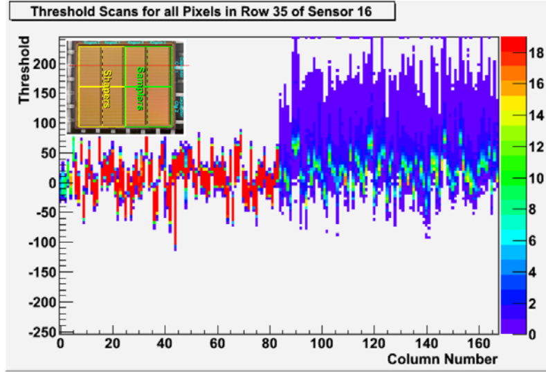
Figure 5.2: A sample 2D histogram showing the profiles of the threshold scan histograms for all pixels in row 35 of the test sensor when those pixels were active. In order to acquire all the threshold scans depicted, 42 threshold scan runs (with one in every 42 pixels active in each case) were merged together with the inactive pixels in each run being discarded. The small picture in the top left hand corner of the histogram is a picture of the test sensor with the location of row 35 marked by a red line. All threshold measurements are in TU.
