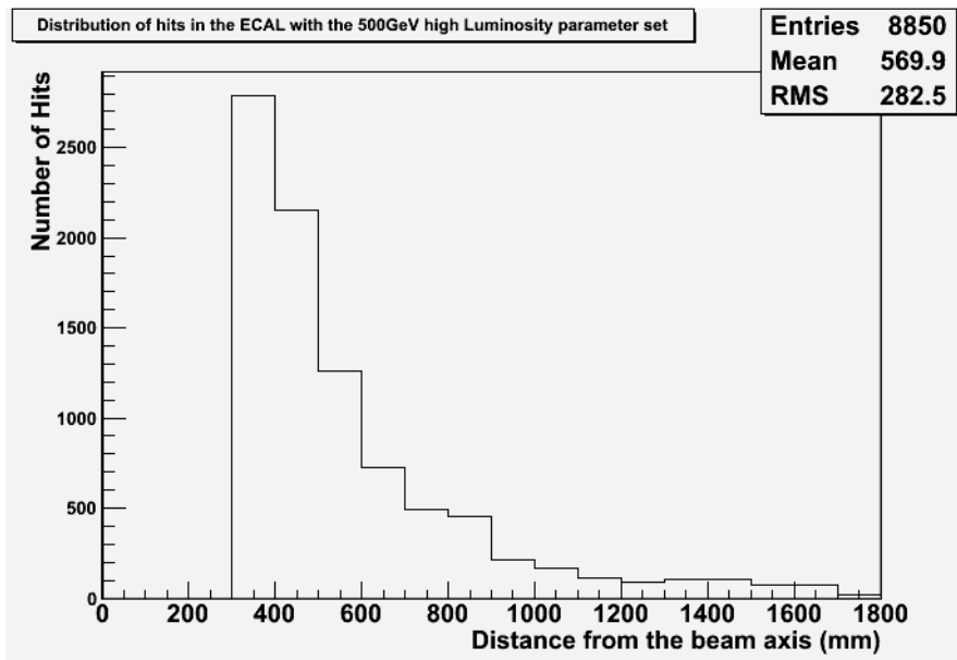
Figure 4.5: A sample histogram showing the distribution of hits in the LDC01 ECAL endcap relative to the beam axis recorded after a single bunch crossing using the 500 GeV High Luminosity parameter set. Note: this distribution does have a minimum hit energy cutoff of 3 \times 10^{-6} GeV.
