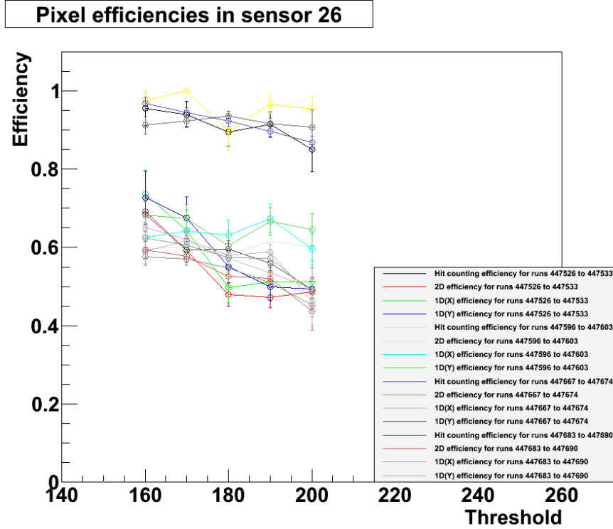
Figure 7.41: Pixel efficiencies in test sensor 26 calculated separately for each test beam run. As shown on this plot there were a small number of cases where the efficiency was calculated to be either exactly zero or exactly one. This was due to extremely low statistics in the runs in question (the small error bars in these cases are due to limitations in the error calculations at very high or very low efficiencies, not low uncertainty). Runs where this occurred were typically excluded from the mean efficiencies shown in figures 7.33 to 7.40. The counting method efficiencies shown here were calculated using a three \sigma search range.
