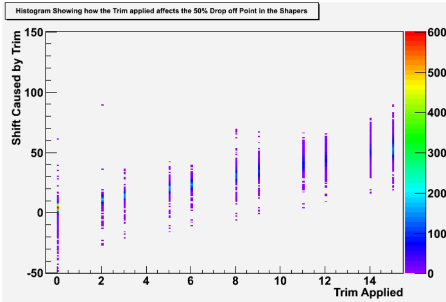
Figure 5.21: A plot showing the shifts in pixel drop off points in shaper pixels in sensor 16 caused by applying different trim settings. This data was collected by comparing run set 450674 to 450715 (untrimmed) to run set 452267 to 452308 (trim based on 50% drop off point, separate targets for shapers and samplers, trim range assumed to be 50 threshold units). All threshold measurements are in TU.
