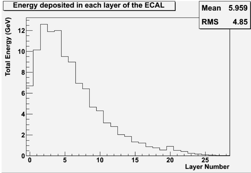
Figure 6.15: A sample histogram showing the distribution of energies deposited in different layers of the analogue ECAL during 1000 simulated events using a 0.25 GeV photon. The relatively small energy deposited in the outer layers of the ECAL implies that the photon shower was typically well contained with the ECAL at this energy (0.25 GeV was the lowest particle energy used for this study). The energy deposited on the outermost 10 layers of the ECAL was doubled to represent the increased thickness of the absorber layers paired with these sensitive layers. This causes the energy recorded to increase at layer 20. Note: this histogram records the combined energies deposited on the ECAL during the entire simulation run, not the energies of individual events.
