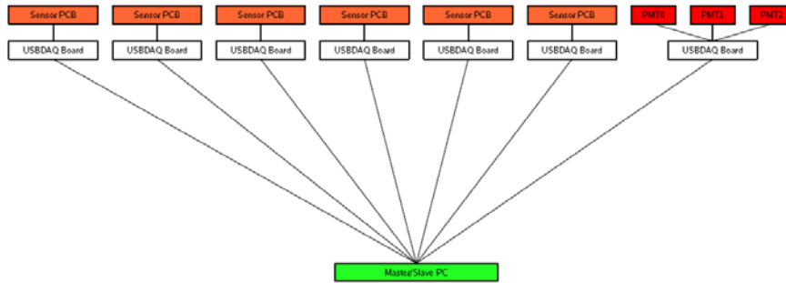
Figure 7.8: Block diagram of the second DAQ layout used for the TPAC 1.2 test beam (used from 21/08/2009 to 28/08/2009). The black lines connecting components represent cables carrying data (in various formats) between the components.
