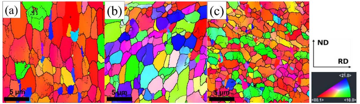
Figure 3-14. Microstructural evolution of as-received sample (a) IPF map with grain boundary distribution of as-received sample (b), IPF map with grain boundary distribution of 600 °C sample and (c) IPF map with grain boundary distribution of 700 °C sample.
