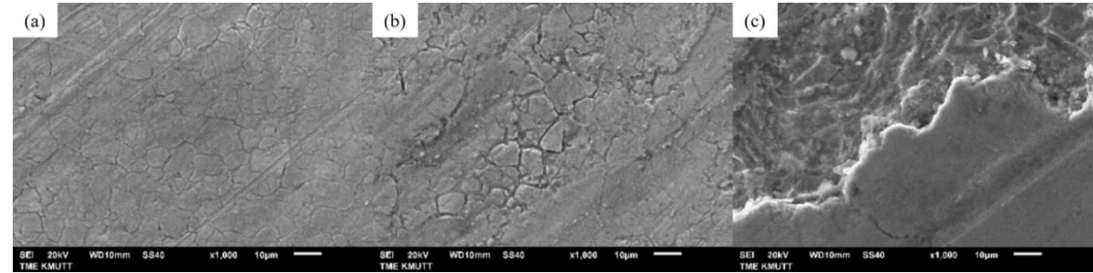
Figure 2-25. Surface quality on workpiece, (a) SUS 304, (b) SUS 316L, (c) Ti Gr2 [87].
