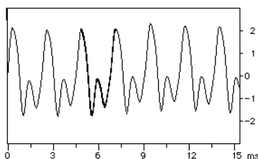
(a) Waveform of a flute playing the note A4 (440Hz). Taken from [63].
