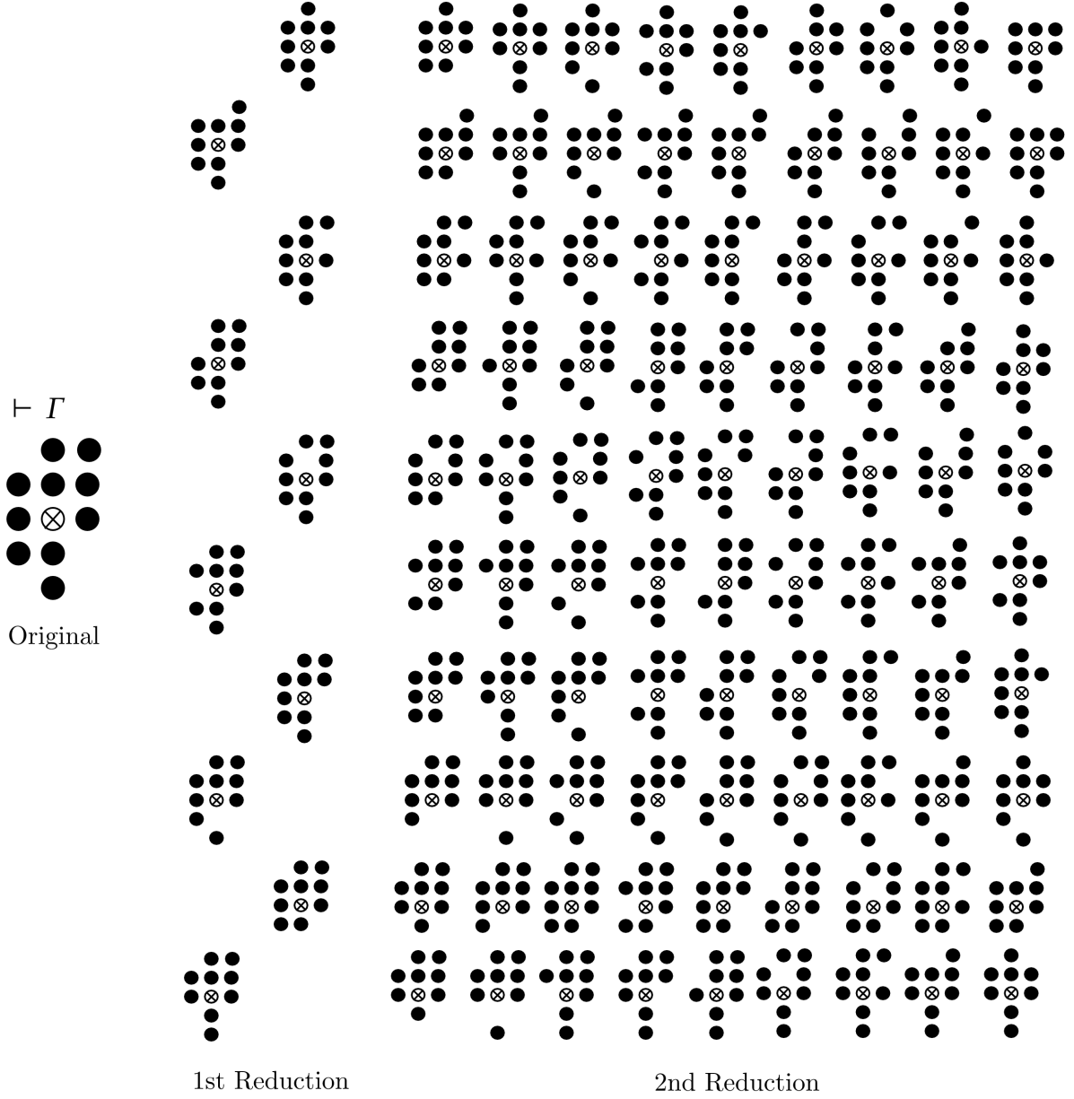
Figure 4.19: Enumeration of the first two reduction steps of a \otimes for a \vdash \Gamma configuration, given the maximum number of possible generators. Each row shows an edge case reached from a single reduction on the original case, and the corresponding 10 cases following a second reduction.
