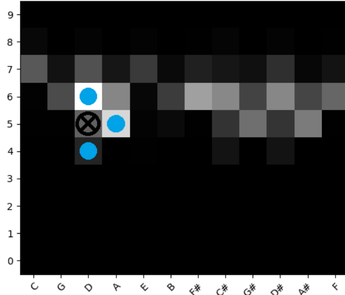
Figure 5.26: An edge case (specifically \emptyset ) being exhibited on real data (trumpet) - with D4, A5, and D6 (dots) as the fundamentals, and D5 being the false fundamental, \otimes .
