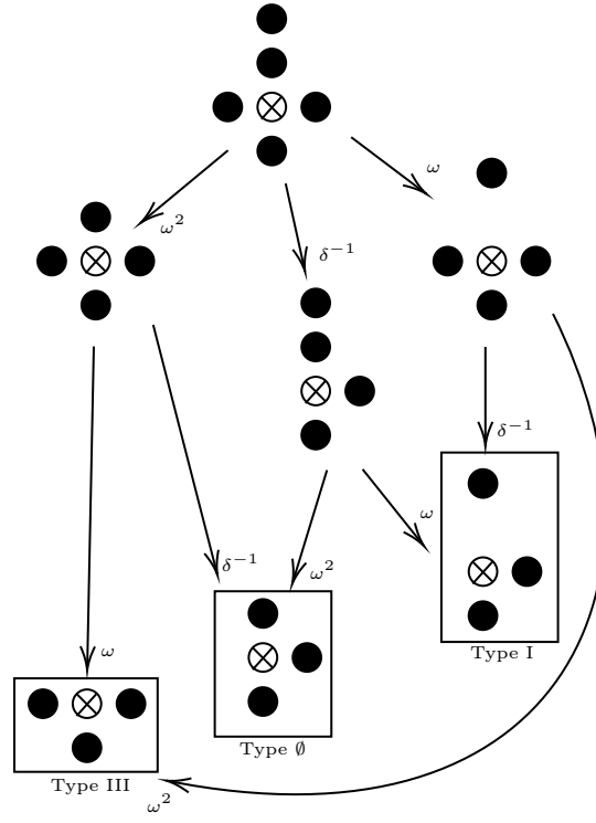
Figure 4.18: An example of a reduction graph, with each step (arrow) showing a reduction in the set of generators. Note that the special case of \{\omega, \omega^{-1}, g(f_2)\} is denoted as ‘Type \emptyset ’, and the configuration is \Gamma\Gamma or \Gamma \vdash .
