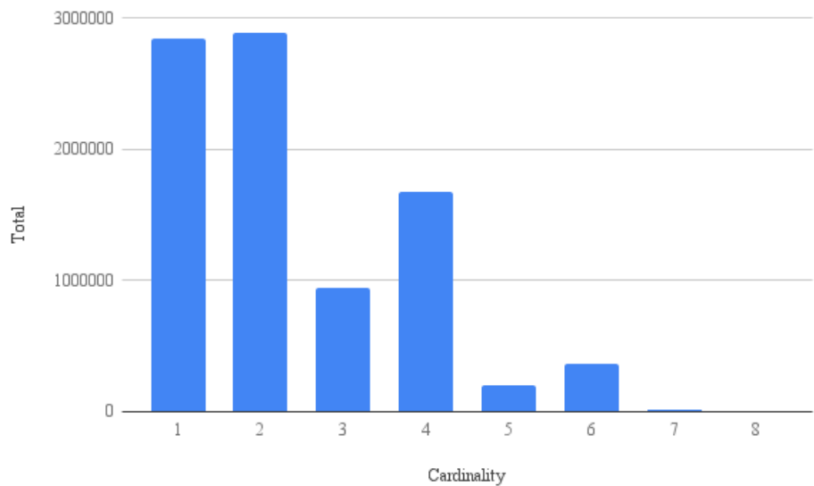
Figure 5.17: Prevalence of graphs with terminal edge set of a given cardinality, averaged across all numbers of simultaneous fundamentals.
