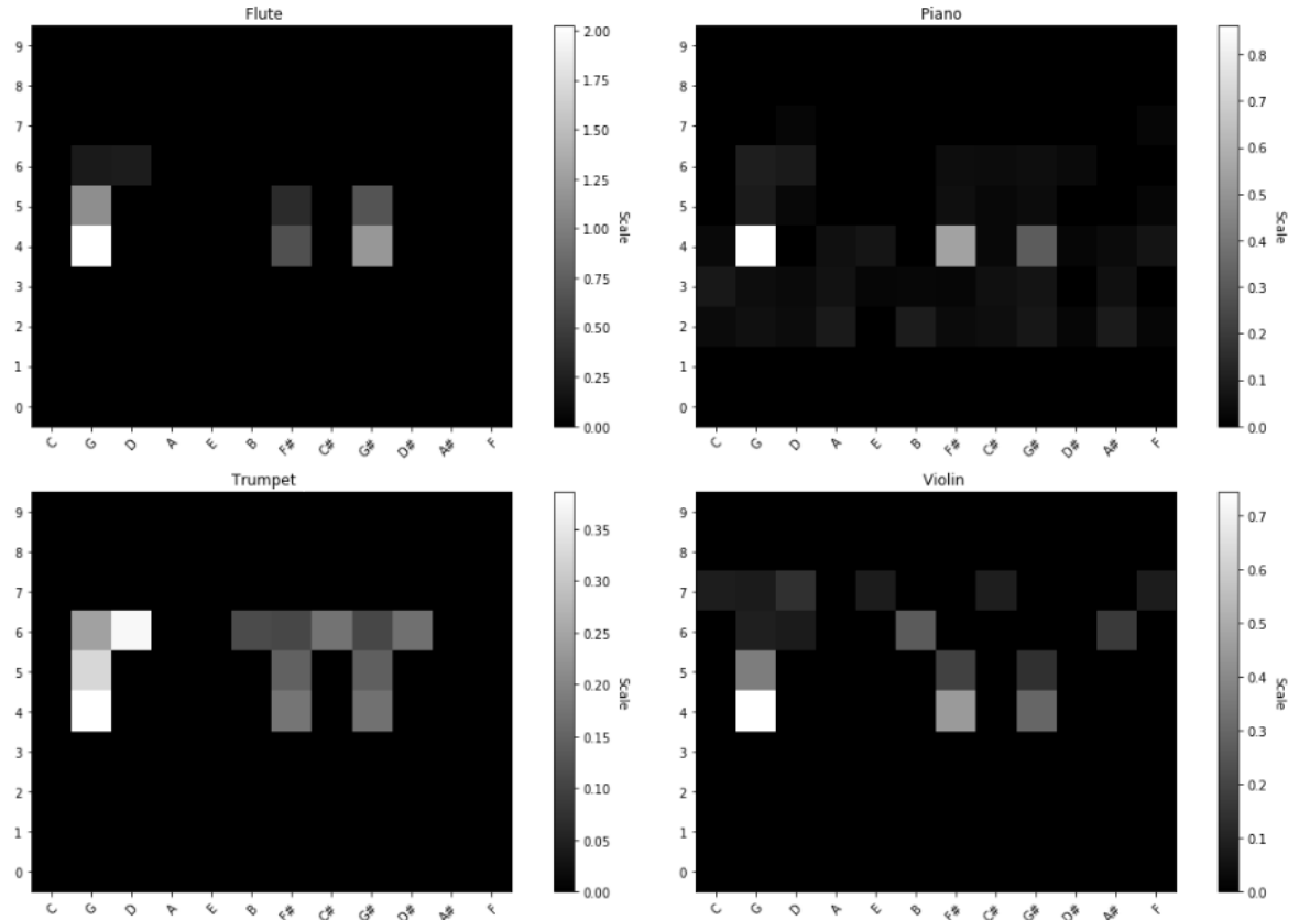
Figure 5.23: The tone G4 being played on a variety of instruments, all exhibiting the \Gamma shape described in Section 4.3. For flute, trumpet, and violin, the sample was taken from the stationary period, whereas the Piano sample was from part-way through the onset, as this resulted in a clearer image
