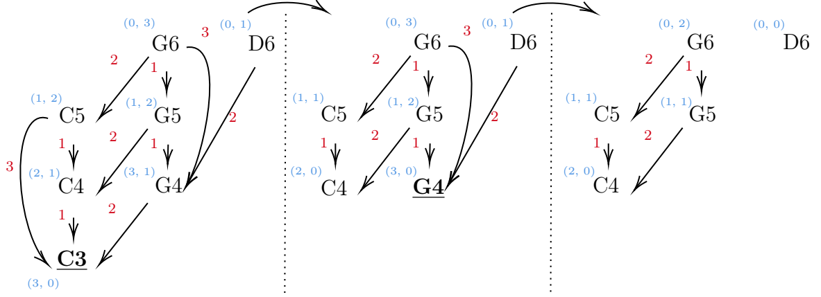
Figure 4.4: ( left ) A directed graph depicting C3 and G4 (and each of their first three harmonics sounding). The degrees of each vertex are shown in parentheses. The following steps represent the steps of the simple algorithm described. The bolded/underlined tone at each step is the one selected as a fundamental.
