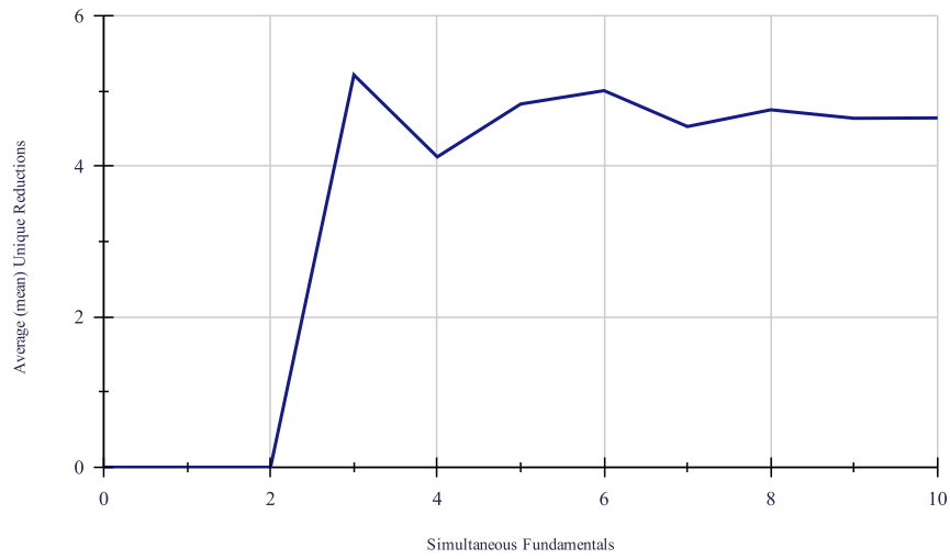
Figure 5.6: A graph showing the estimated average number of terminal vertices for varying numbers of simultaneous unique fundamentals (0, 10] - corresponding to the left hand side of Subfigure 5.2. Note that contrary to Subfigure 5.2, 20000 sample interpretations were taken here, as opposed to 1000.
