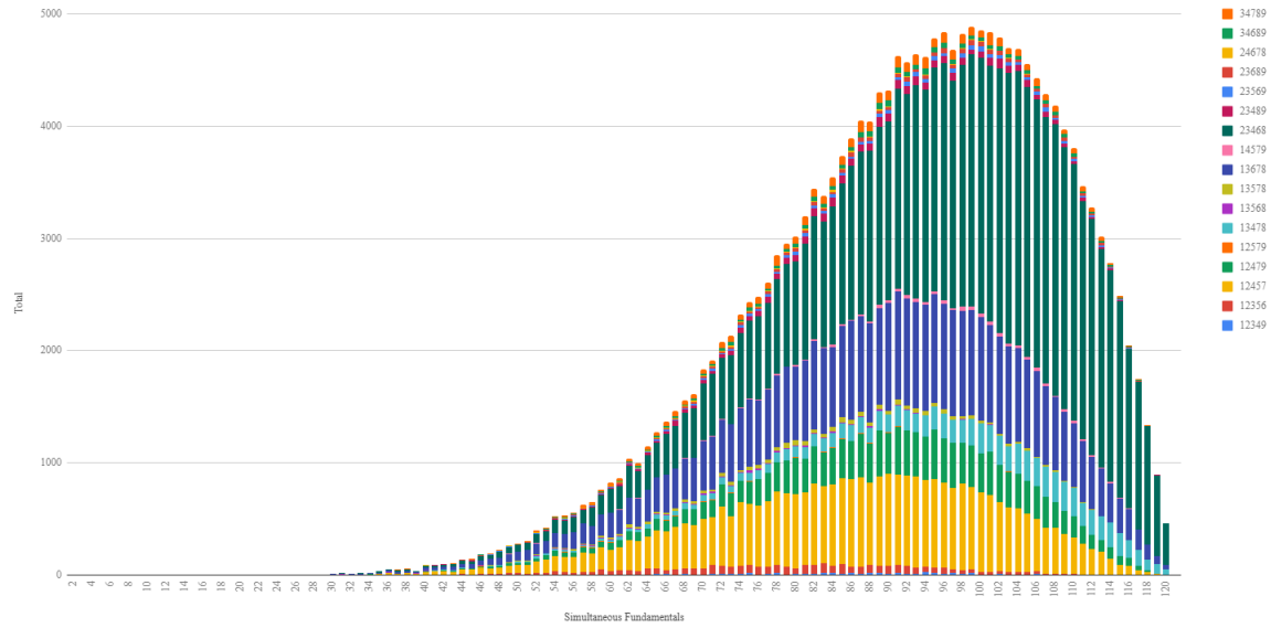
Figure 5.13: Breakdown of terminal vertex sets with cardinality 5 against number of simultaneous fundamentals.
