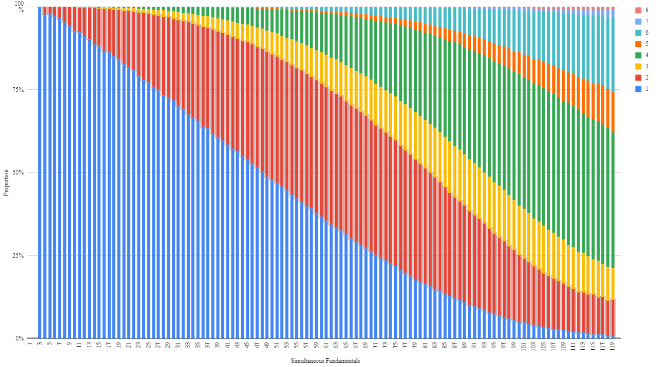
Figure 5.22: Proportion of graphs with terminal vertex sets of varying cardinality as the number of simultaneous fundamentals is varied.
