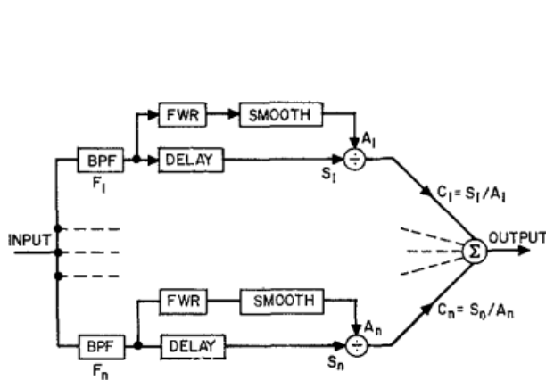
(a) A schematic for a spectrum flattener.
