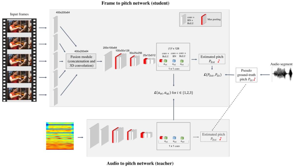
Figure 3.6: An overview of the NN architecture described in [97].
