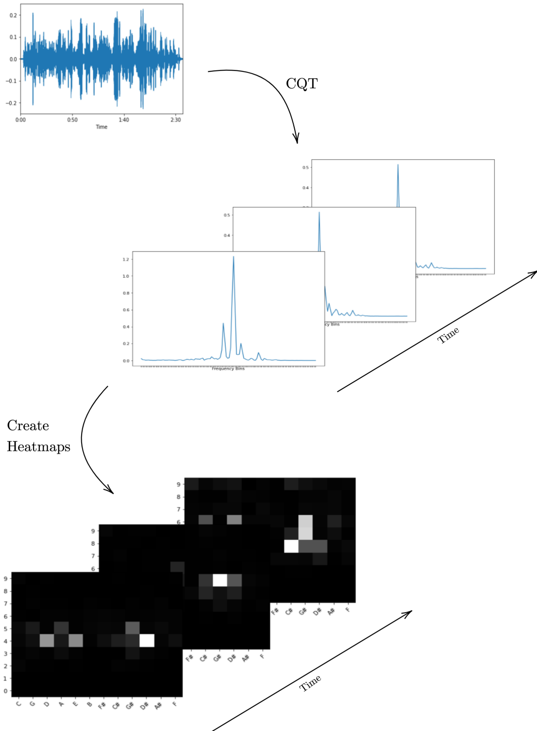
Figure 5.27: Example of the path ‘real’ data takes from waveform (i.e. time domain signal) to frequency domain signal, and then to heatmap. The data used is from Bach’s Prelude and Fugue in C-sharp minor, BWV 849.
