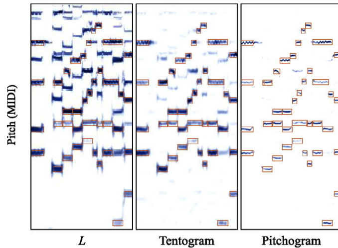
Figure 3.7: Demonstration of the progression from Spectrogram to Tentogram, and then to Pitchogram. Taken from [51].
