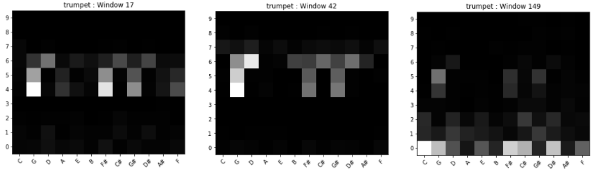
Figure 5.25: A closer look at how heatmaps differ as the tone progresses from onset/attack, to stationary period, to offset/decay (left-to-right).
