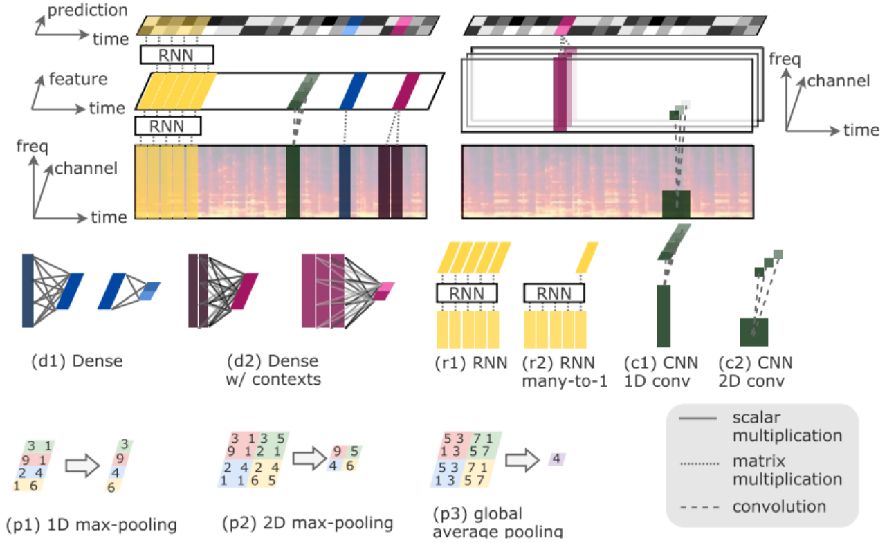
Figure 3.5: Neural Network layers in the context of MIR. Taken from [25].
