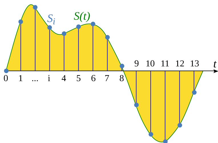
Figure 2.19: A demonstration of discrete sampling of a continuous signal. The green line ( S(t) ) represents the continuous signal, whilst the vertical blue lines, S_i , represent the samples.
