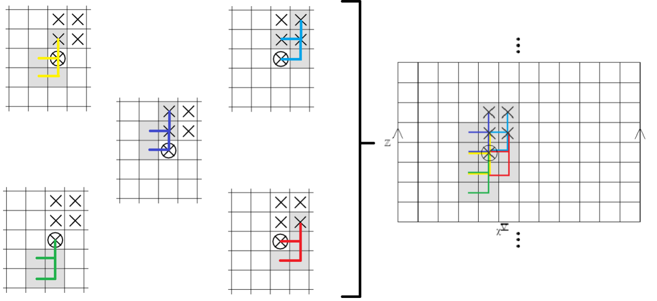
Figure 4.10: Figure showing where a false fundamental and each of its apparent harmonics could have been generated from, with colours tracing out \neg and \downarrow for each tone (overlying both \Gamma and \vdash situations).
