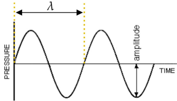
Figure 2.14: An annotated sine wave with wavelength, \lambda .
