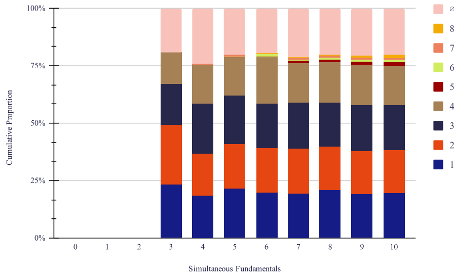
Figure 5.7: A stacked bar chart showing the change in proportional prevalence of basic edge types and \emptyset for (0, 10] simultaneous unique fundamentals.
