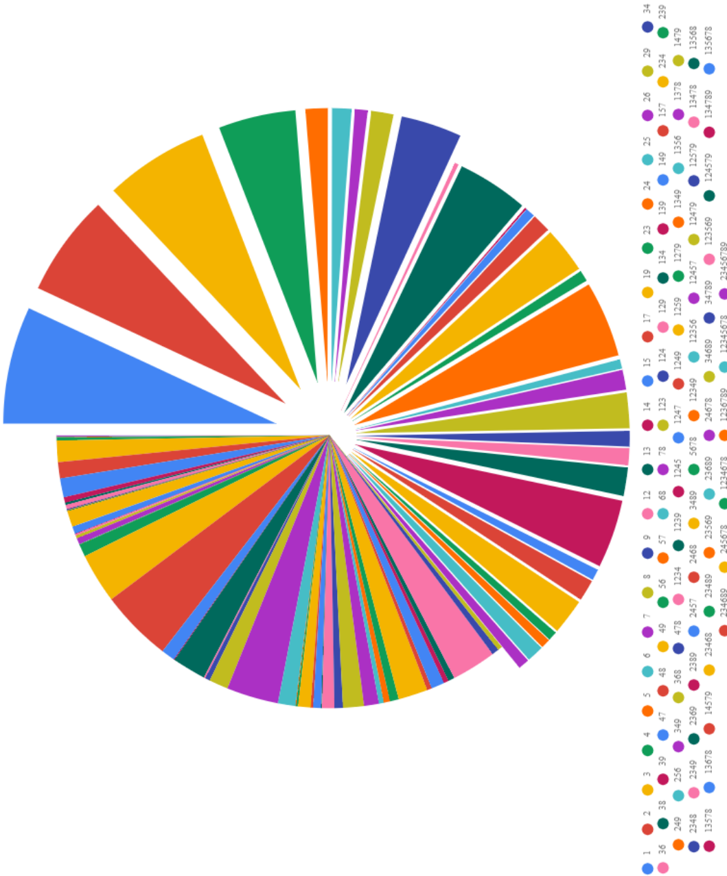
Figure 5.21: Prevalence of all 92 terminal vertex sets, with the cardinality one cases floated out furthest from the centre, and the cardinality two cases floated out half way between these and the rest of the cases. Note that slices are labelled ascending in a clockwise fashion.
