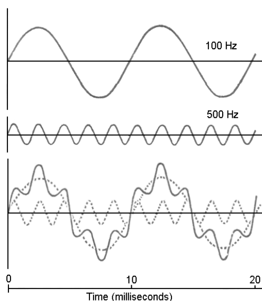
(a) Superposition of two waves. Taken from [43], adapted from [103].
