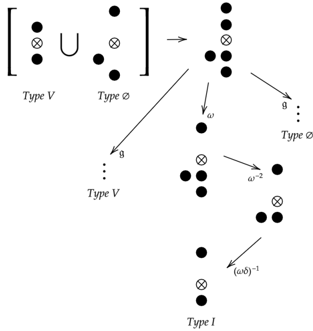
Figure 5.20: Partial reduction graph for the reduction of the union of Types V and \emptyset , demonstrating the appearance of a further basic edge Type as a terminal vertex. Note that the vertical dots after the reduction by an arbitrary generator, g , are used to denote that some number of reduction steps lead to the indicated Type.
