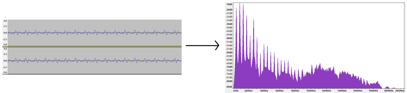
Figure 2.29: Fourier Transform (right) of the waveform of a Flute playing A440 (left).
