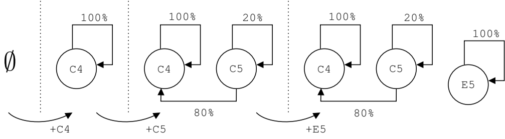
Figure 4.1: The build-up of a simplistic probabilistic representation.
