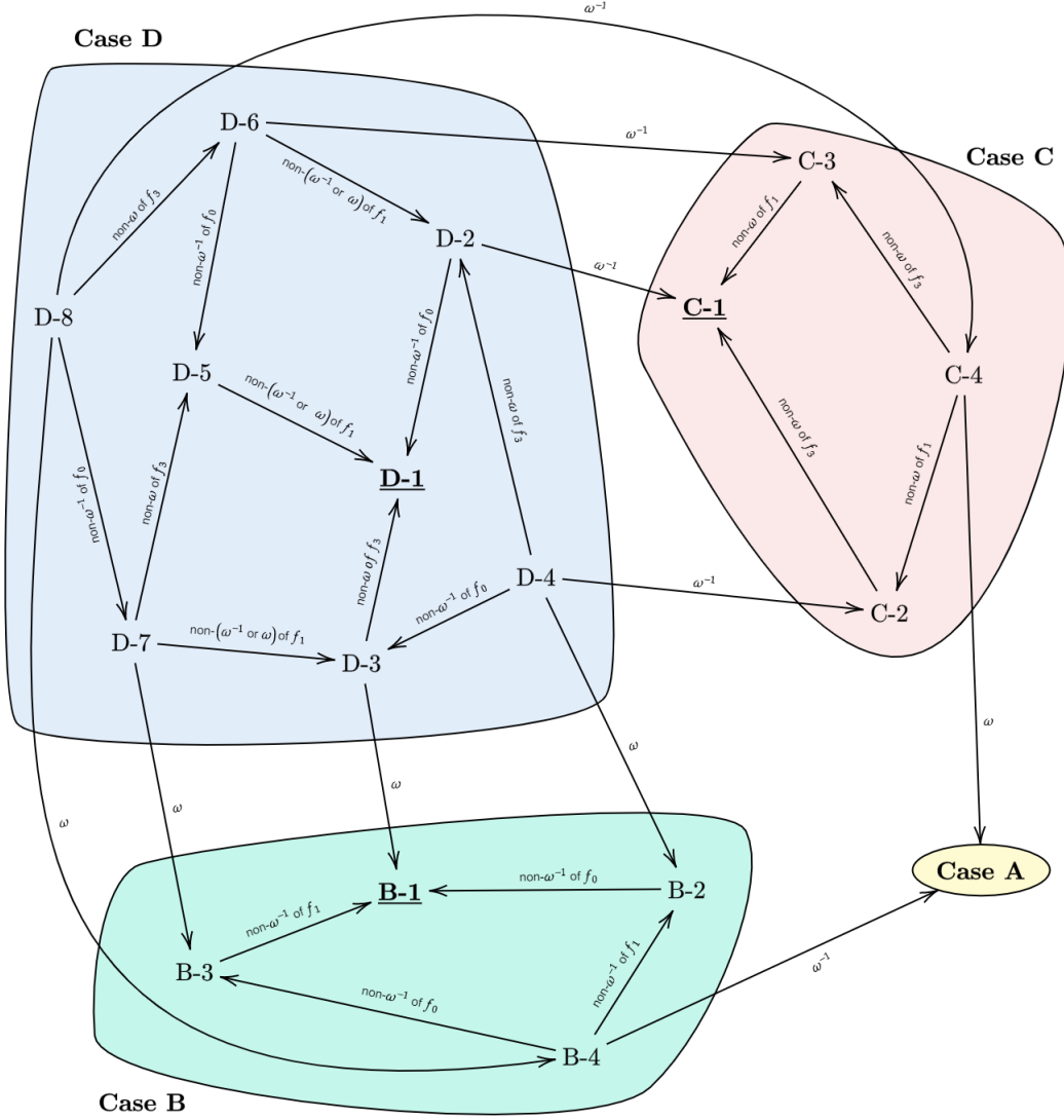
Figure 4.17: A diagram representing the graphical structure relating the various cases laid out in Proposition 6.1. For the terminal vertices (bolded), Cases A, B-1, and C-1 are all basic, and D-1 is the irreducible non-basic case.
