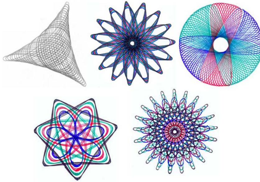
Figure 2.26: Various designs drawn using a Spirograph, demonstrating just some of the possible complexity achievable, even with the toy.
