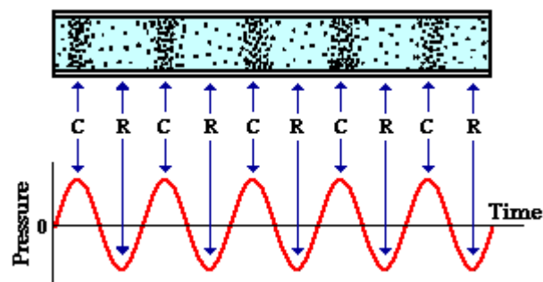
Figure 2.15: Compression (C) and Rarefaction (R) of a sine wave. Taken from [135].
