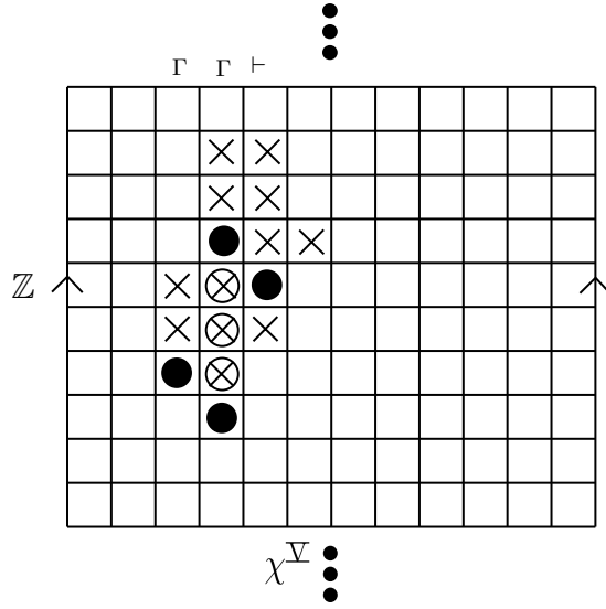
Figure 4.9: Counterexample showing that not all \Gamma shape-exhibiting tones are fundamentals.
