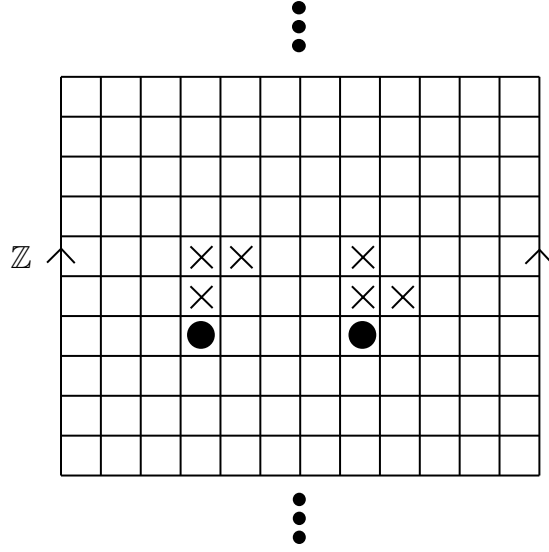
Figure 4.7: Demonstration of the \Gamma and \vdash shapes in \mathcal{N}^{\mathbb{V}} .
