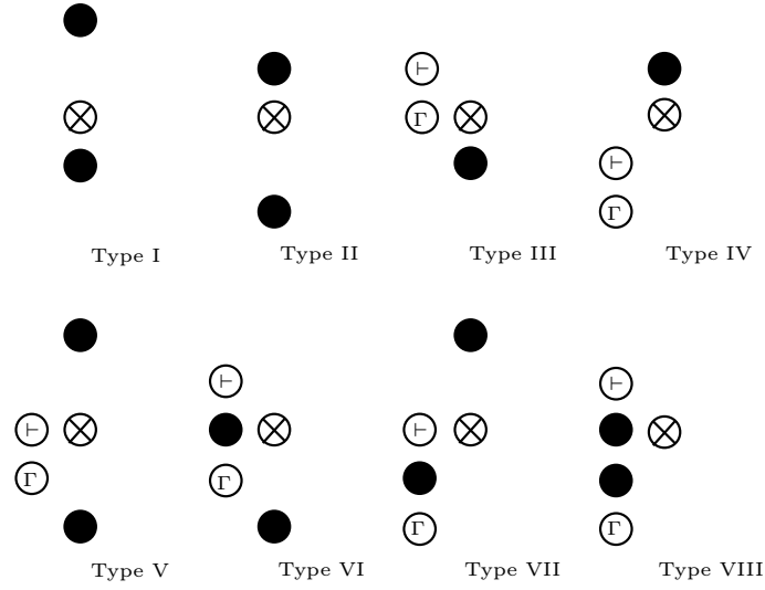
Figure 4.13: The eight basic edge types represented visually. Each \bullet represents a generator, with \otimes representing the false fundamental, and the unfilled generators containing \vdash or \Gamma denoting the shape drawn out in the \delta^{-1} column (i.e. corresponding to \Psi(\pi_\chi(\delta^{-1}(\otimes))) ).
