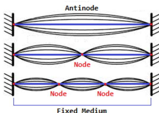
Figure 2.18: The first three standing waves of a fixed medium - namely the fundamental ( f_0 ), first harmonic ( f_1 ), and second harmonic ( f_2 ), from top to bottom.
