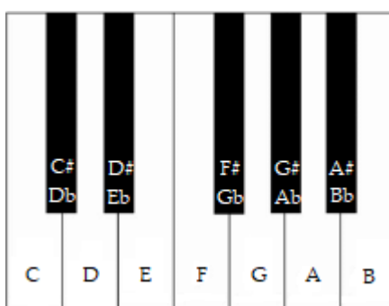
Figure 2.23: The twelve semitones in an octave, demonstrating the ordering to the pitch chromas.
