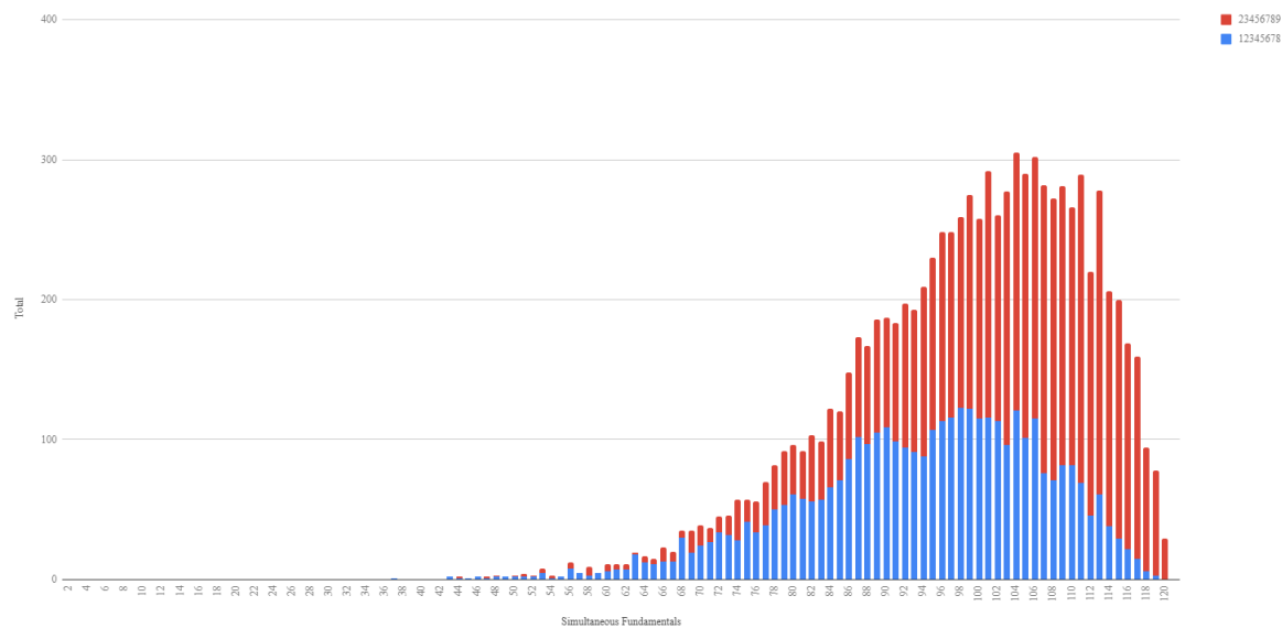
Figure 5.16: Breakdown of terminal vertex sets with cardinality 8 against number of simultaneous fundamentals.
