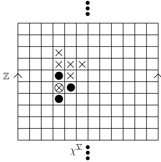
Figure 4.16: An irreducible non-basic edge case.
