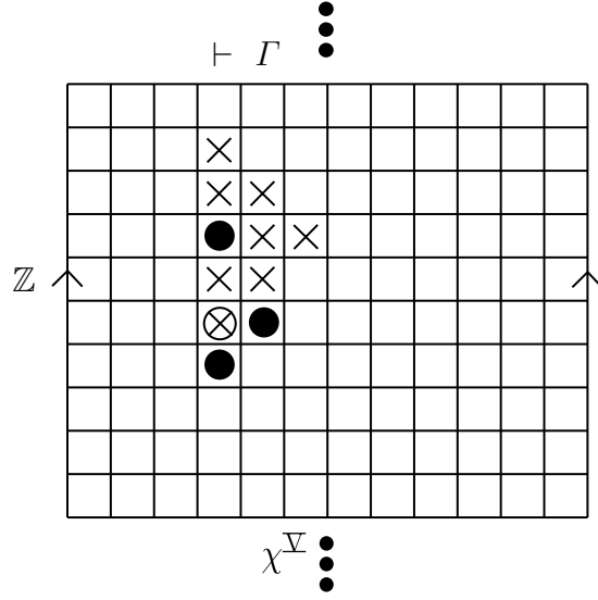
Figure 4.11: A basic edge case in a \vdash \Gamma configuration - note that each of the harmonics associated to the constituent tones of the false fundamental, \otimes , have a single generator.
