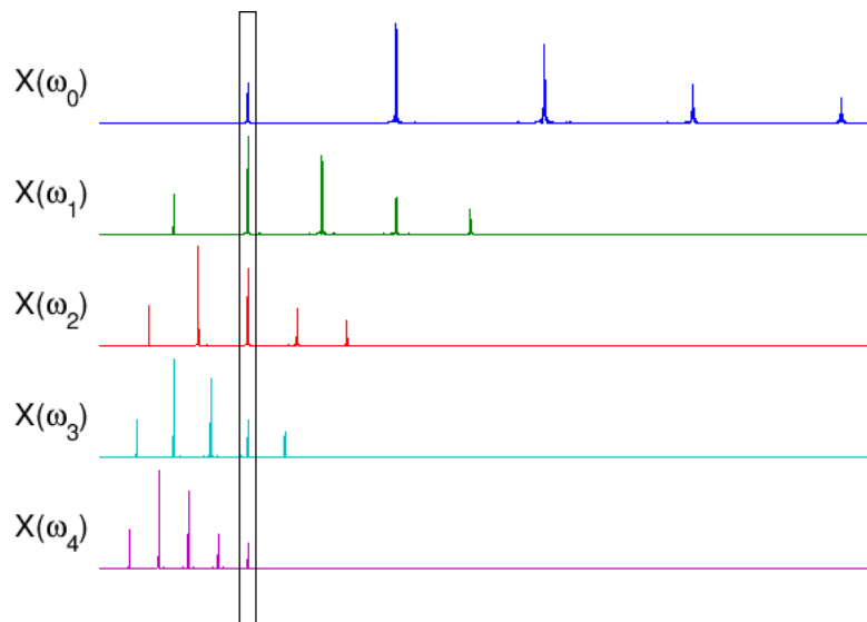
Figure 3.3: Visual representation of Noll’s HPS algorithm. Taken from [160].
