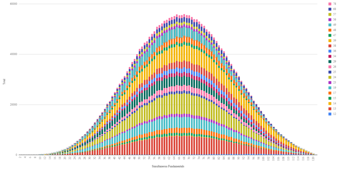
Figure 5.10: Breakdown of terminal vertex sets with cardinality 2 against number of simultaneous fundamentals.
