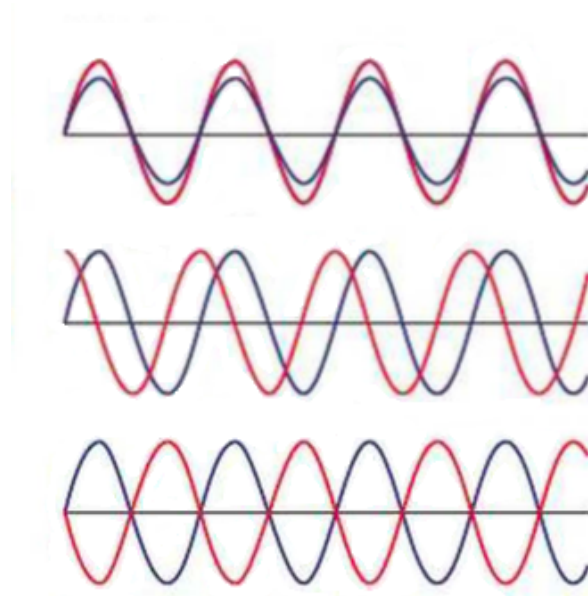
(b) Two waves in phase, out of phase, and in antiphase respectively.
