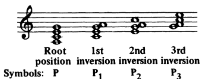
Figure 2.3: The root position and first three inversions of the pentatonic chord. Figure taken from [8].
