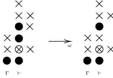
Figure 4.15: A reduction removing a generator in \vdash \bigcup \Gamma . Note that g(f_2) is omitted for brevity.
