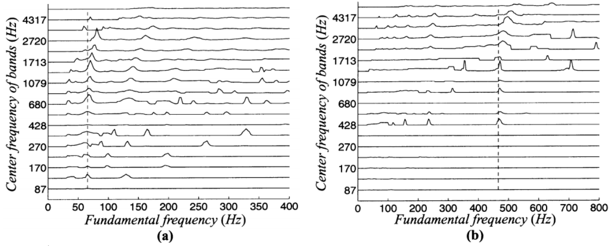
Figure 3.4: Bandwise-calculated weights of two piano tones, (a) f_0 = 65\text{Hz} and (b) f_0 = 470\text{Hz} . The actual pitches of the harmonics are depicted by the vertical dashed lines. Adapted from [96].
