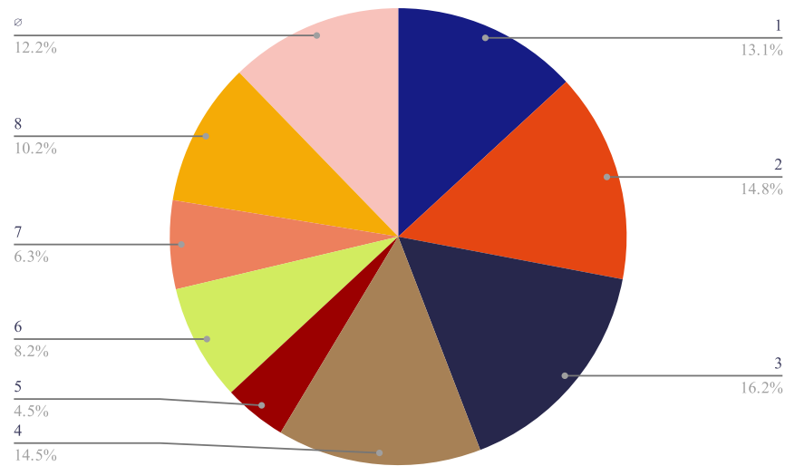
Figure 5.1: A pie chart showing the average (proportional) prevalence of each edge type, and \emptyset when considering between 0 and 120 simultaneous fundamentals.
