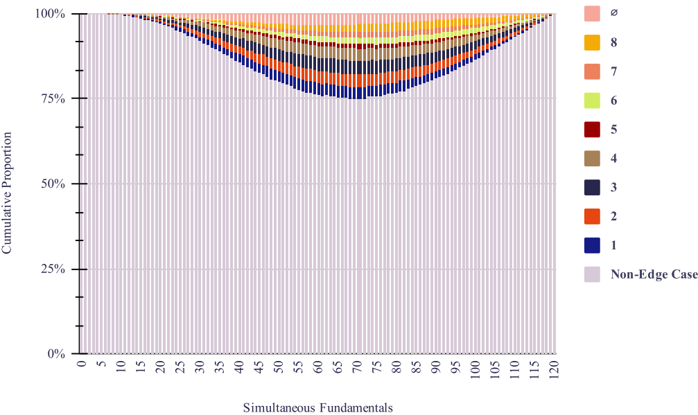
Figure 5.4: Another stacked bar chart, mirroring Figure 5.3, but including the proportion of non-edge cases.
