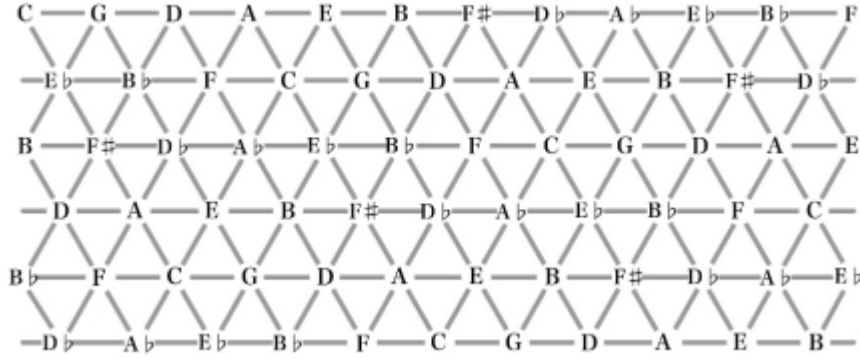
Figure 3.8: A Tonnetz without identified edges - clearly showing its periodic nature in both the vertical and horizontal directions. Taken from [15].
