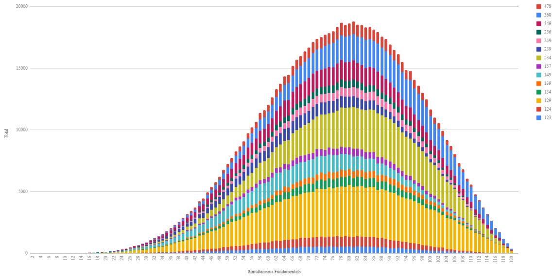
Figure 5.11: Breakdown of terminal vertex sets with cardinality 3 against number of simultaneous fundamentals.
