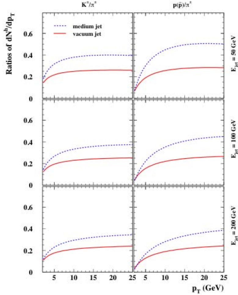
Figure 3.12: Results of the MLLA+LPHD formalism for K^\pm/\pi^\pm and p(\bar{p})/\pi^\pm ratios in jets with energies E_{\text{jet}} = 50, 100 and 200 GeV [83]. The enhancement in both ratios increases with decreasing jet energy and the onset of the enhancement occurs more sharply at lower jet energy
