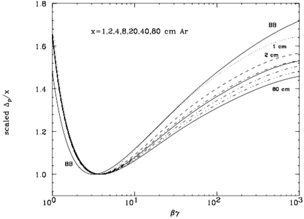
Figure 4.11: Scaled values of \Delta_p/x for Argon segment lengths x as a function of particle momentum. The Bichsel functions (dashed lines) are shown to differ with segment length from the Bethe-Bloch function at higher \beta\gamma [100].
