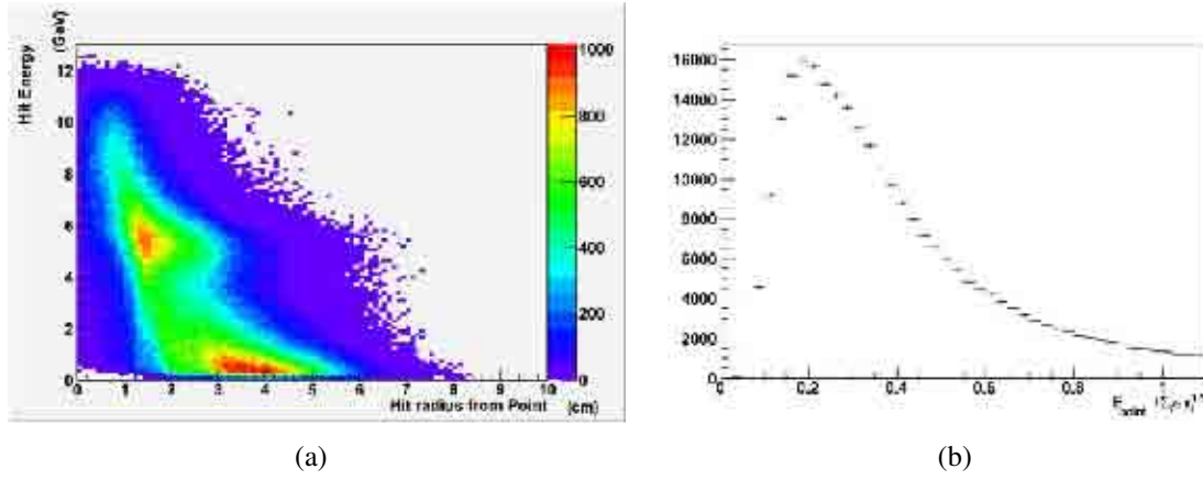
Figure 6.26: Figure (a) shows the distribution of the point energy on the shower maximum detector from point centre. Figure (b) shows the total point energy to the sum of radius weighted hit energy ratio for each point trigger.
