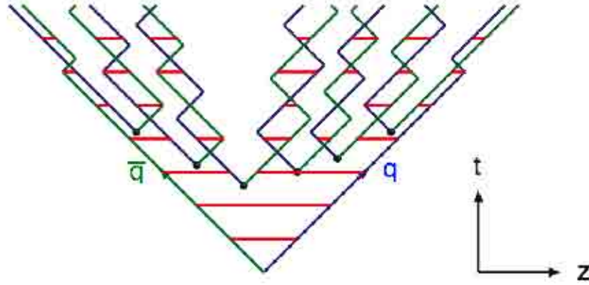
Figure 3.5: Space-time evolution of a string fragmenting into hadrons [2]. Hadronisation commences at the centre of the string where lower momentum hadrons are produced
