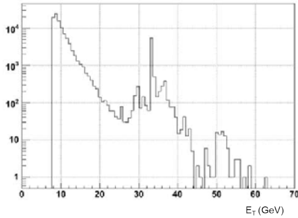
Figure 5.1: Tower E_T distribution taken from electromagnetic calorimeter triggers. A power law distribution is expected however large fluctuations are observed, above 20 GeV, that can be attributed to faults in individual towers
