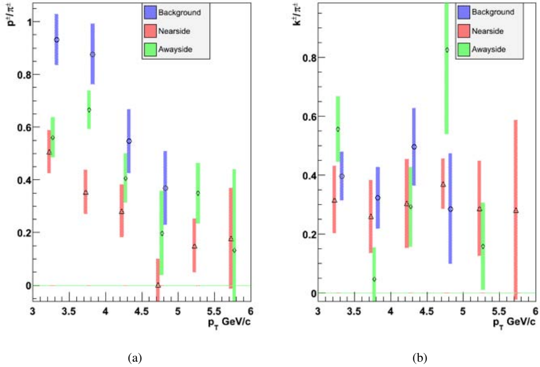
Figure 6.29: Figure (a) reveals the p^\pm/\pi^\pm ratios for the near side jet, away side jet and background regions of \Delta\phi , without the background correction, using \gamma rich central Au + Au event selection. Figure (b) reveals the K^\pm/\pi^\pm ratios for the near side jet, away side jet and background regions of \Delta\phi , without the background correction, using \gamma rich central Au + Au event selection.
