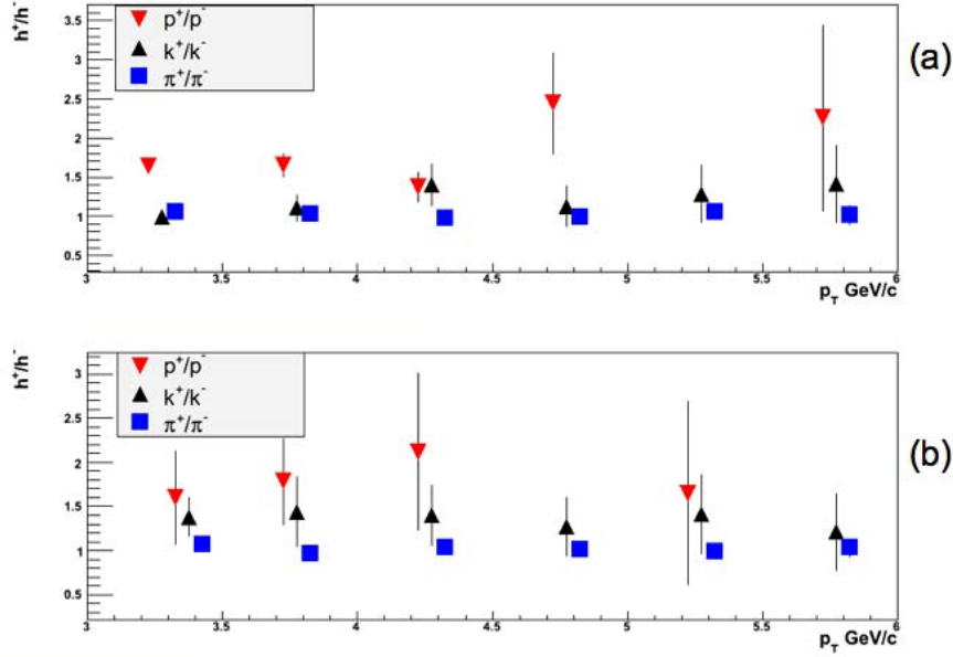
Figure 5.14: Inclusive h^+/h^- hadron ratios Au + Au . Figure (a) shows the hadron ratios from central Au + Au collisions while figure (b) shows the hadron ratios from peripheral Au + Au collisions. Missing data points are caused due to the marker value not being on the graph scale even though the error bars would be present.
