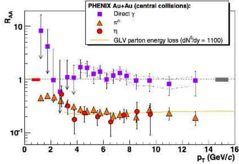
Figure 2.2: PHENIX data showing the R_{AA} for \eta , \pi^0 and direct \gamma [26]. The neutral hadrons exhibit similar suppression in central Au + Au as charged hadrons however the photons show no indication of suppression.
