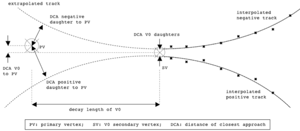
Figure 4.13: Strange hadron reconstruction using reconstructed TPC tracks. The geometrical cuts are also illustrated.
